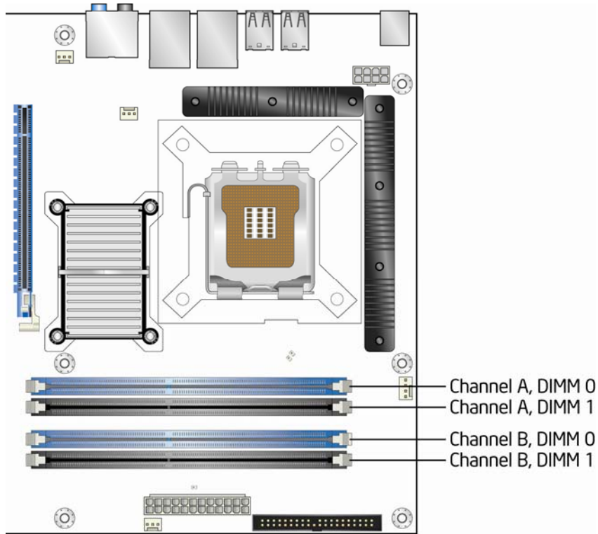
Figure 3. Memory Channel and DIMM Configuration
