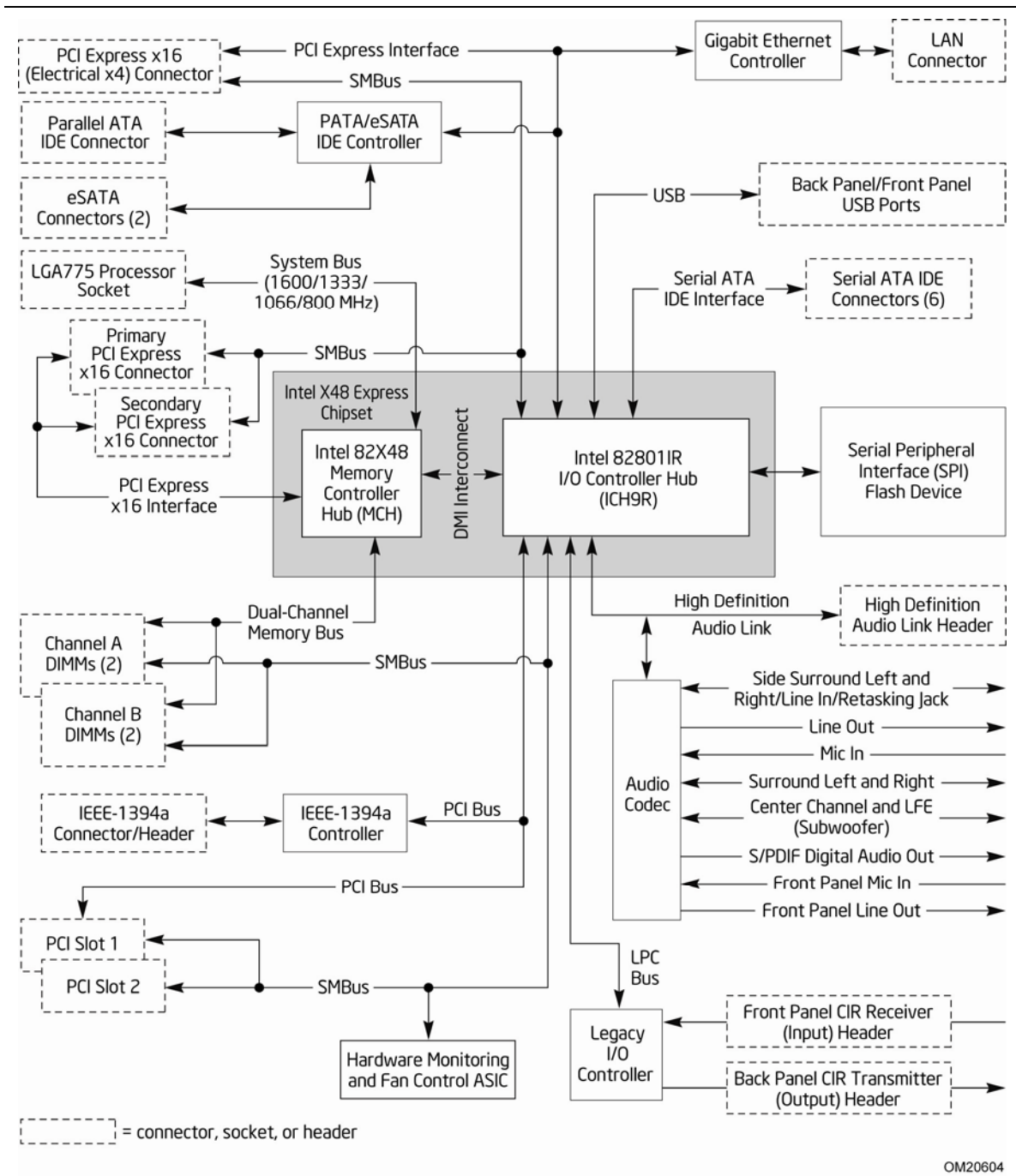
Figure 2. Block Diagram
