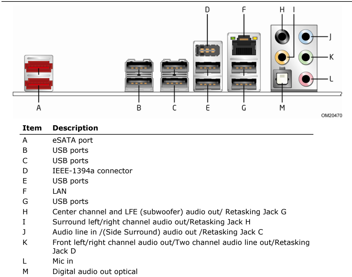
Figure 10. Back Panel Connectors
