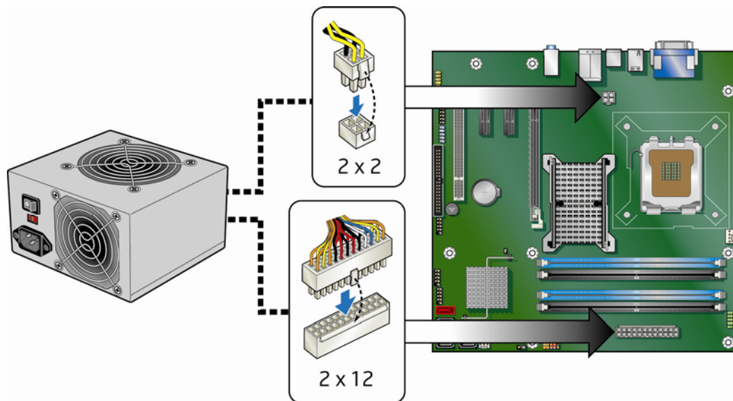
Figure 27. Connecting Power Supply Cables
