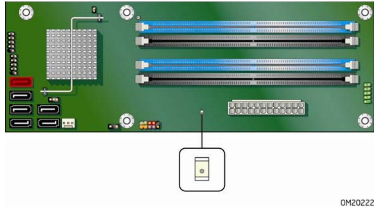
Figure 4. Standby Power Indicator
