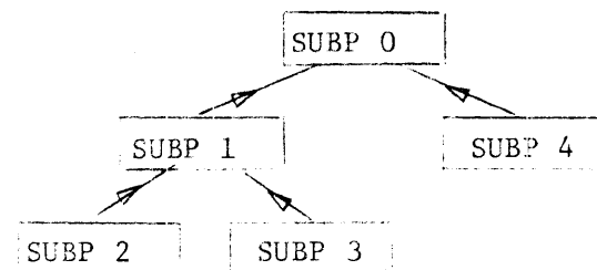
Subprocess Tree
