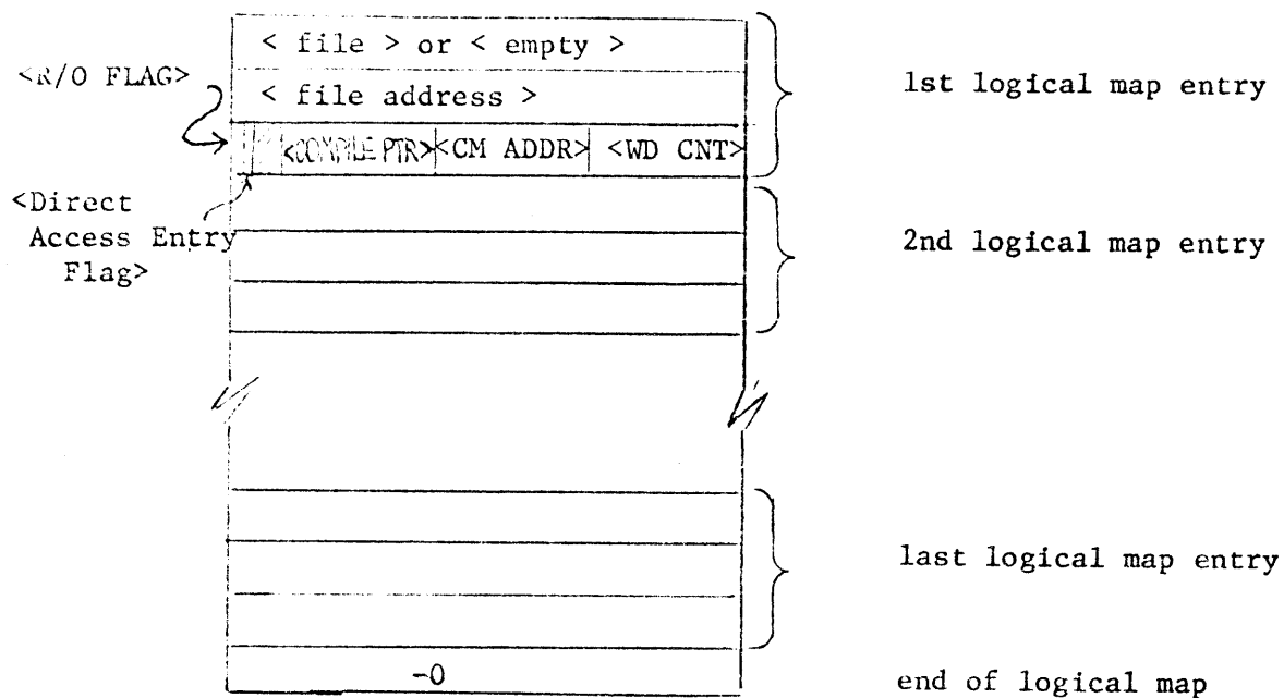
Figure 1 Logical Map
