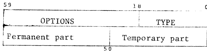
Figure 1. Class Code
