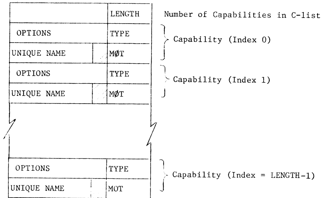
CAPABILITY LIST
