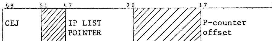
Figure 2 System Call
