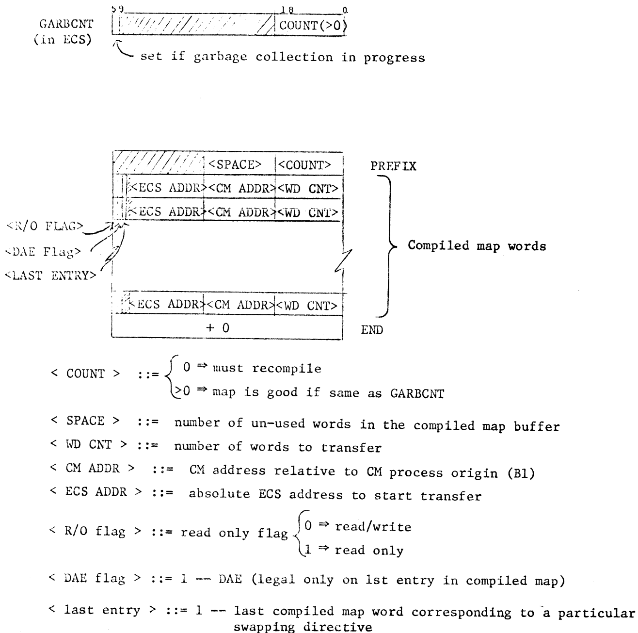
Figure 2 COMPILED MAP
