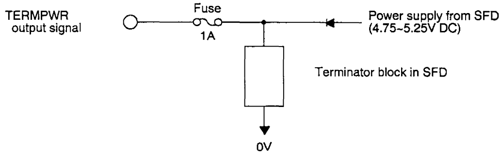
(Fig.11) TERMPWR output circuit
