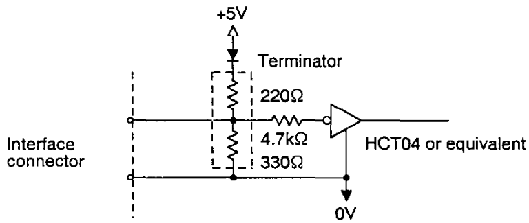
(Fig.8) RESET input circuit
