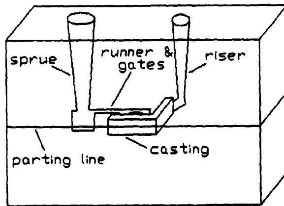
Figure 5: Illustration of sandcasting
