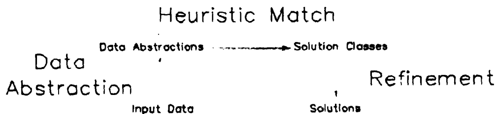
Figure 1: Heuristic Classification
