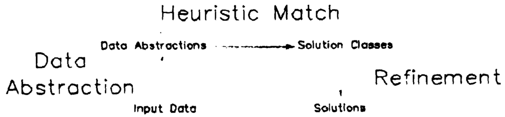
Figure 1: Heuristic Classification
