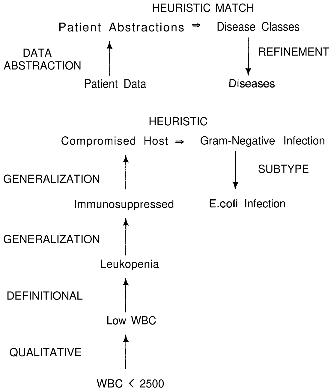
Figure 2- 1: Inference structure of MYCIN
