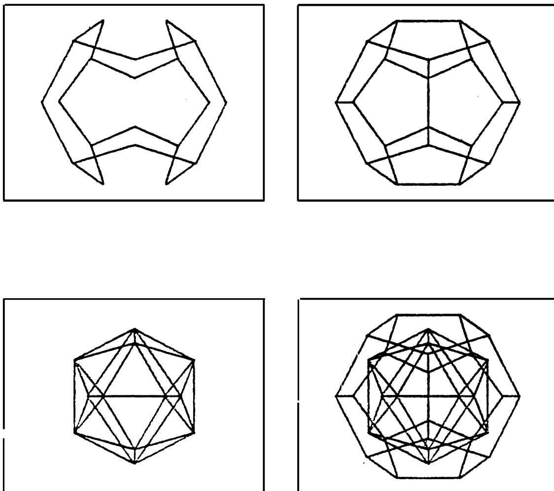
FIGURE 3.8 - Dual of a Dodecahedron.
