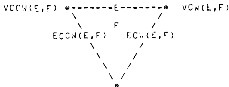
FIGURE 2.5 - Face Perimeter Accessing with respect to edge E.
