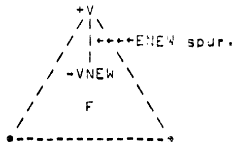
Figure 3.2 - VNEW ← MKEV(F,V);
