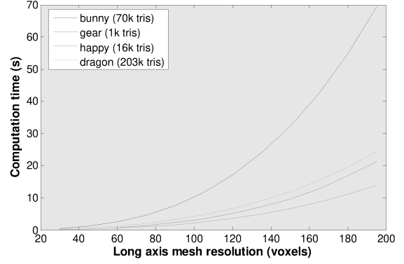
Figure 9. Performance of our distance-map computation approach on all four meshes at a variety of mesh resolutions.
