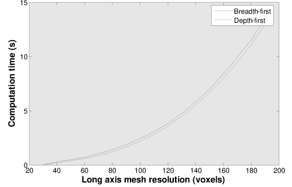
Figure 11. Comparison of depth- and breadth-first search for the “happy” mesh using a TREE_ASCEND_N value of 0 (optimal).
