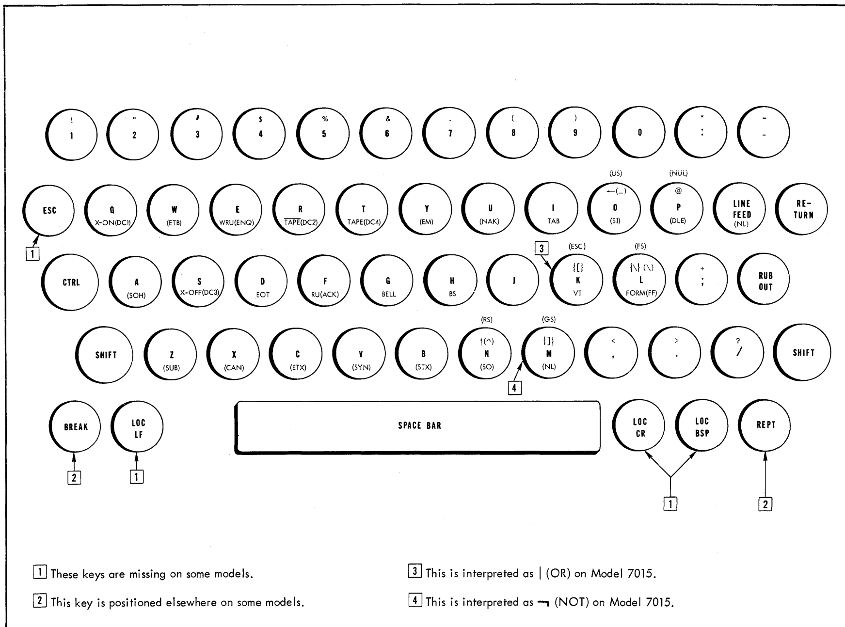
Figure 1. Teletype Keyboard
