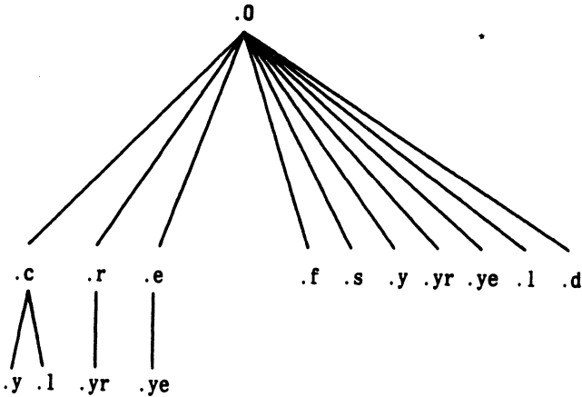
Figure 2-1. Summary of Default Transformation Path
