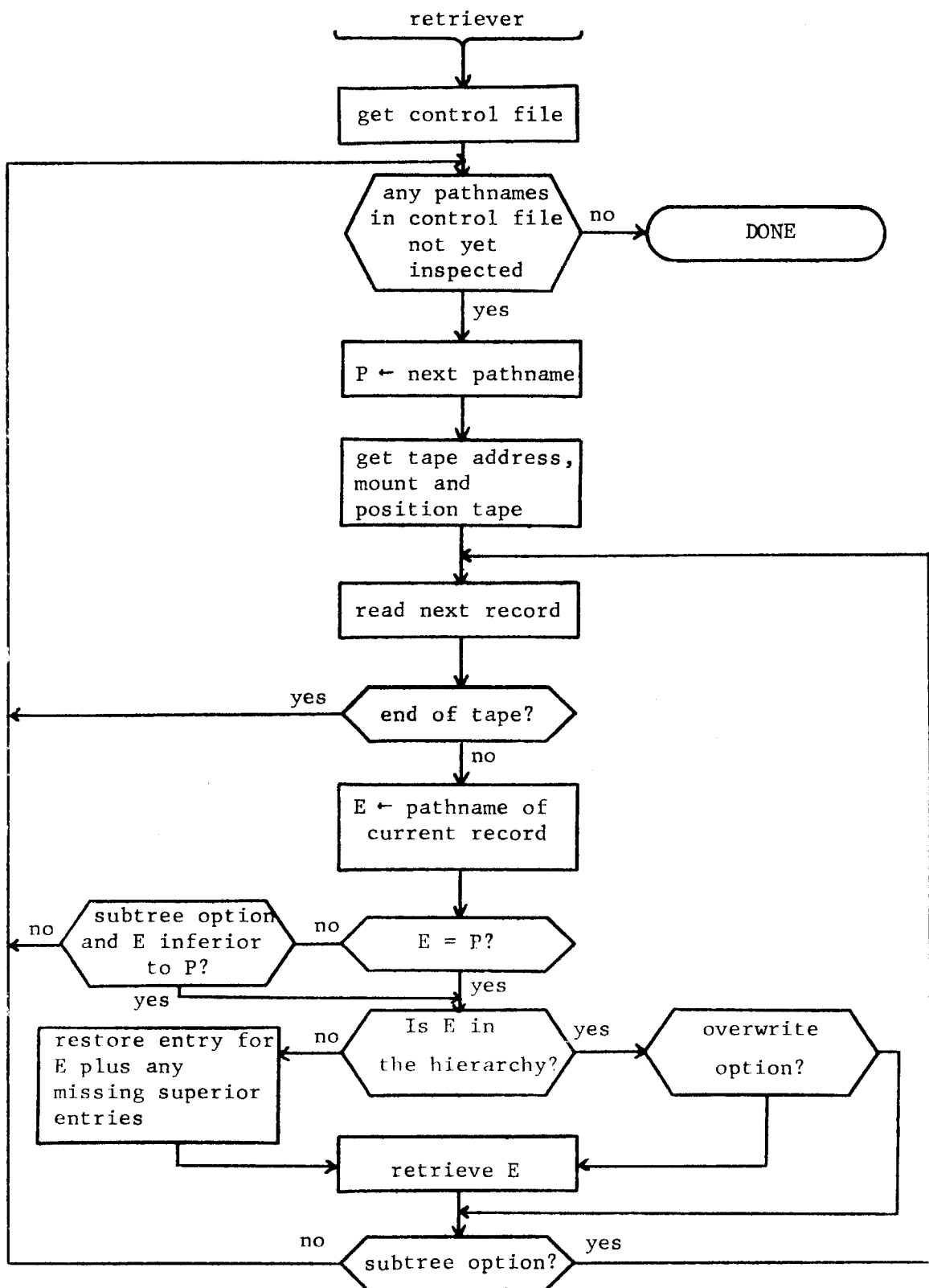
Figure 3.8: The retriever algorithm.
