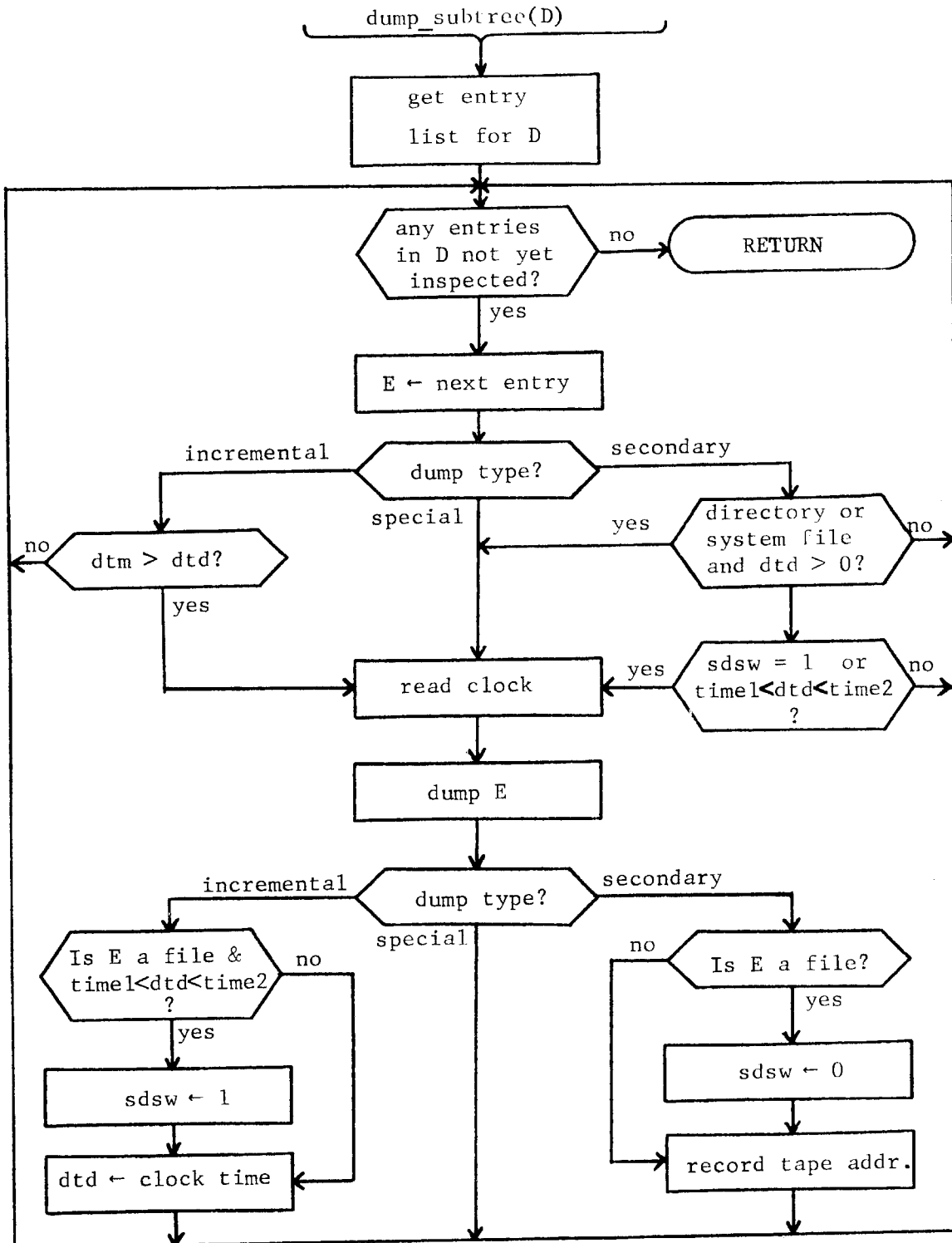
Figure 3.3: The incremental and secondary dumper algorithm (part 2).
