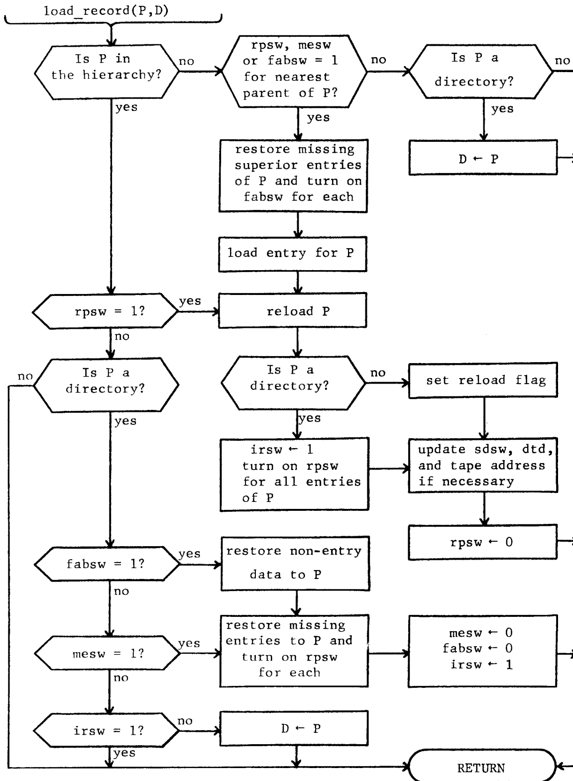
Figure 3.6: The phase 1 reloader algorithm (part 2).
