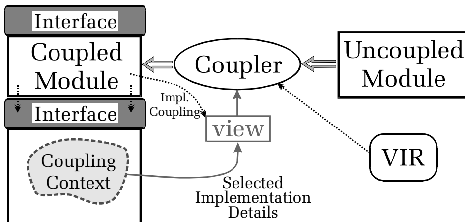
Figure 1-7 - View-Based Abstraction
