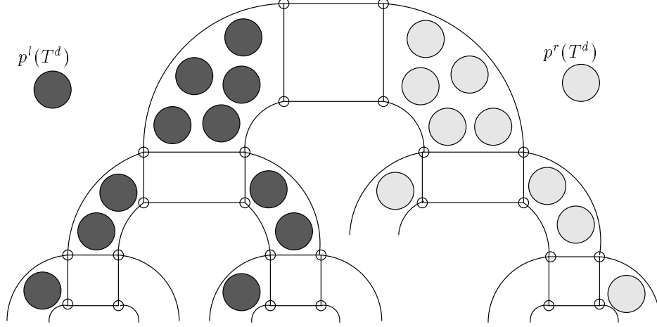
Figure 3-4: Paths used by p_i^l(T^d) and p_i^r(T^d) .
