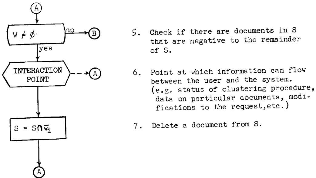
Fig. 5.4. Condition 1 and Deletions.
