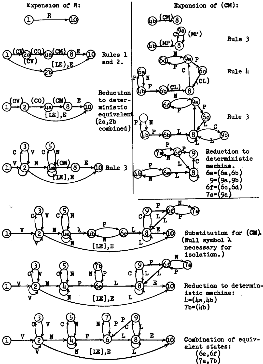
Fig. 8.10. Outline of steps proving equivalence of Backus-normal and finite state descriptions.
