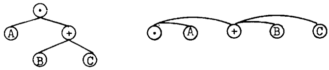
Fig. 7.4. Polish prefix notation.
