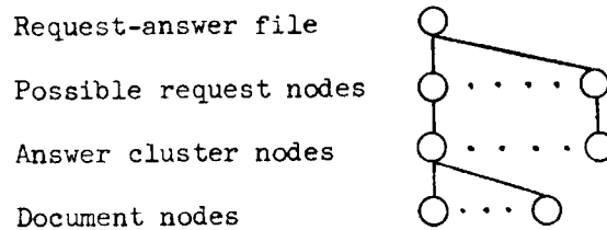
Fig. 7.12. Structure of request-answer file.
