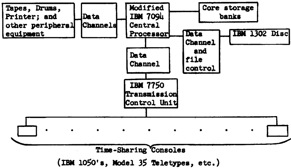
Fig. 6.1. Project MAC Equipment Configuration.
