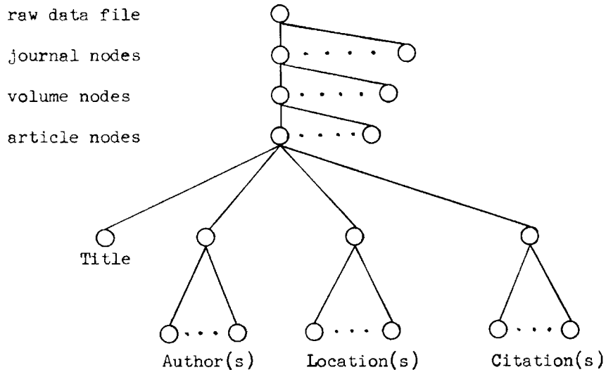
Fig. 7.5. Structure of raw data file.
