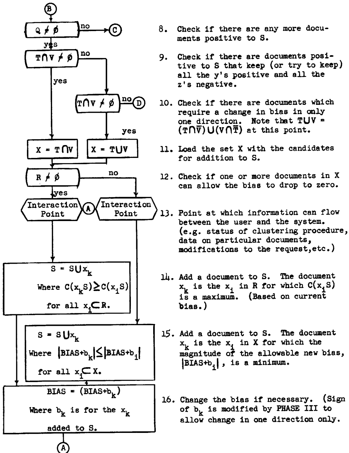
Fig. 5.5. Condition 2 and Additions.
