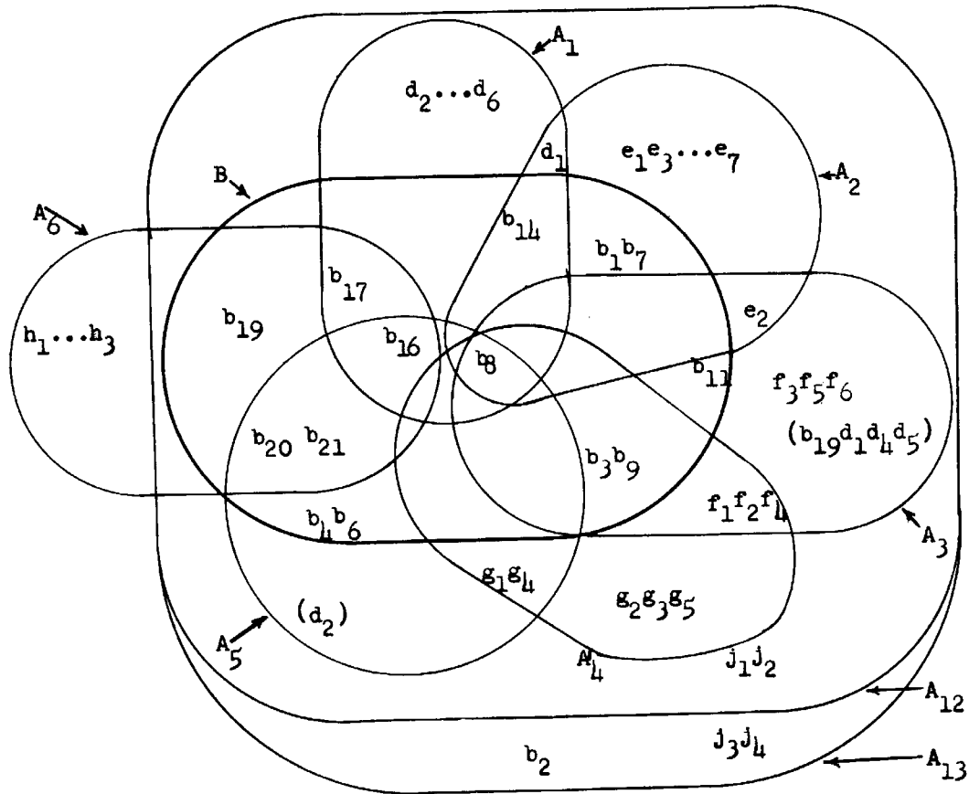
Fig. 9.40. Relationship of Clusters for Langmuir Probe Bibliography (Physicist 2).
