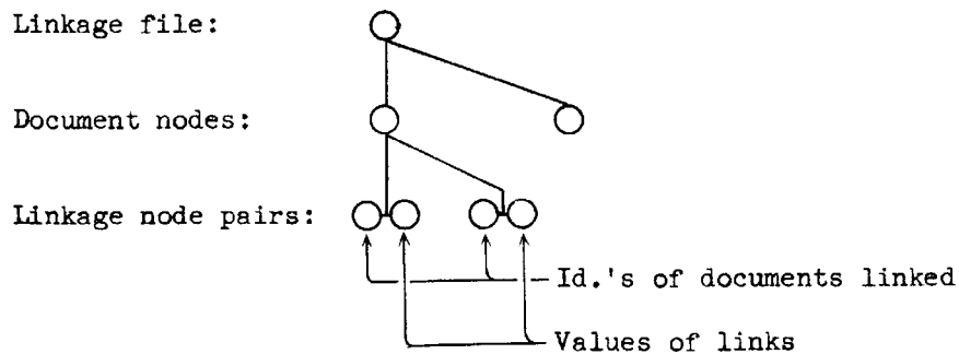
Fig. 7.10. Structure of Linkage File.
