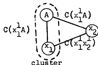
Fig. 5.18. Network for proof of theorem.
