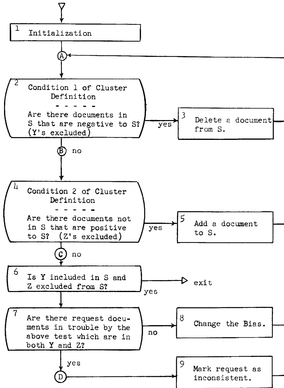
Fig. 5.2. Overall Flow Chart.
