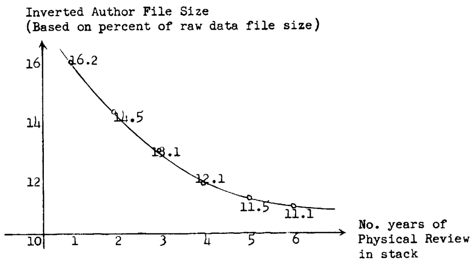
Fig. 7.9. Storage required for inverted author file. (For articles in Physical Review 1959-64)
