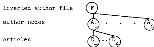
Fig. 7.7. Structure of inverted author file.
