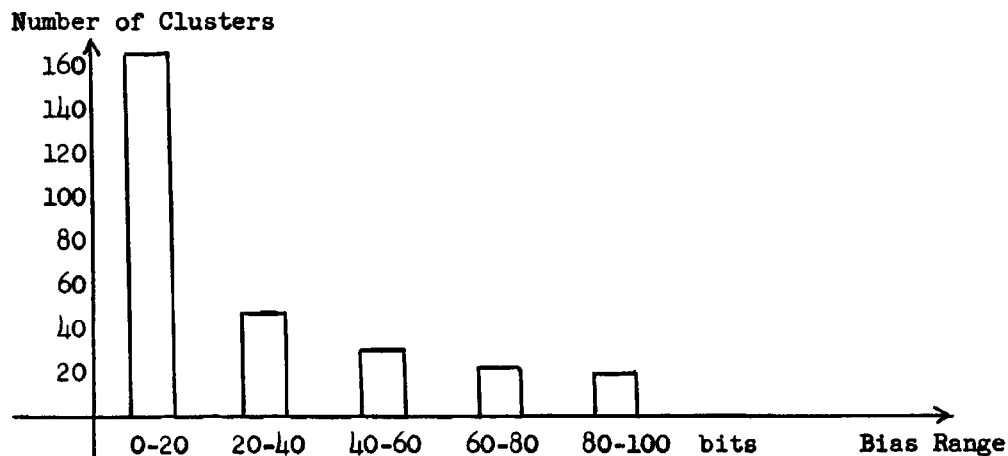
Fig. 9.2. Distribution of clusters by bias for 275 clusters.
