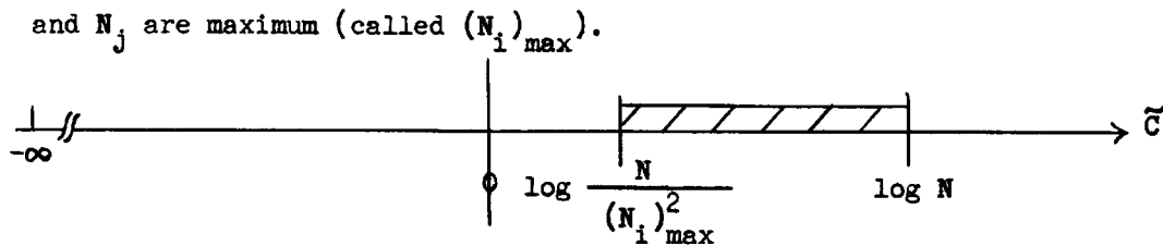
Fig. 3.3. Range of measure of relatedness for test data.
