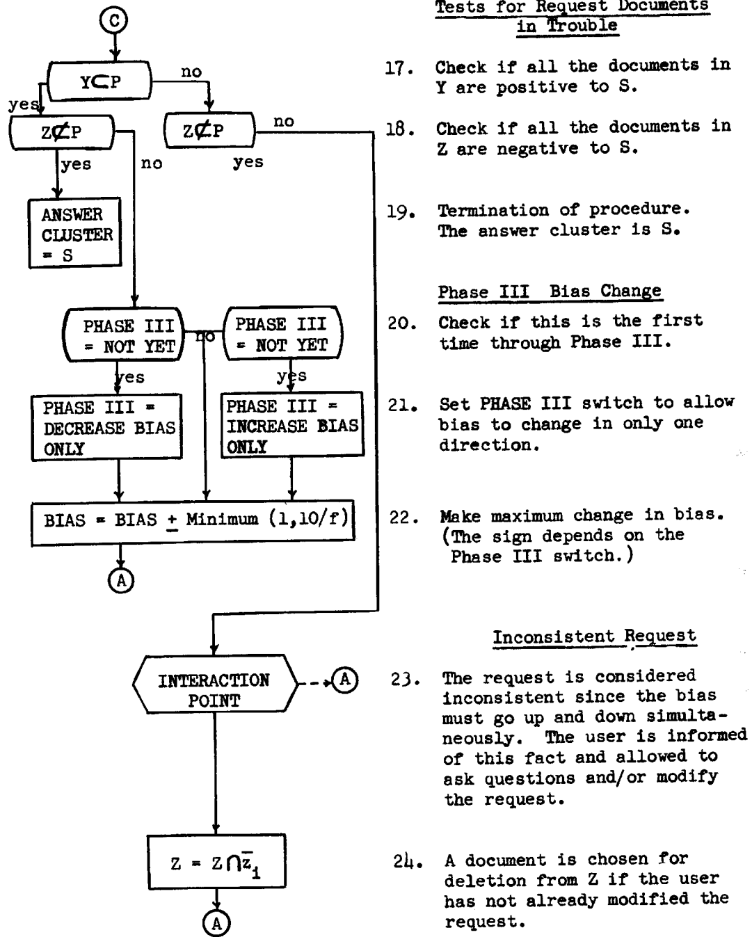
Fig. 5.6. Phase III and other tests.
