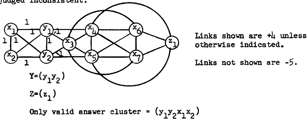
Fig. 5.14. Network illustrating the difficulties involved in knowing which document to add to S on a given iteration.
