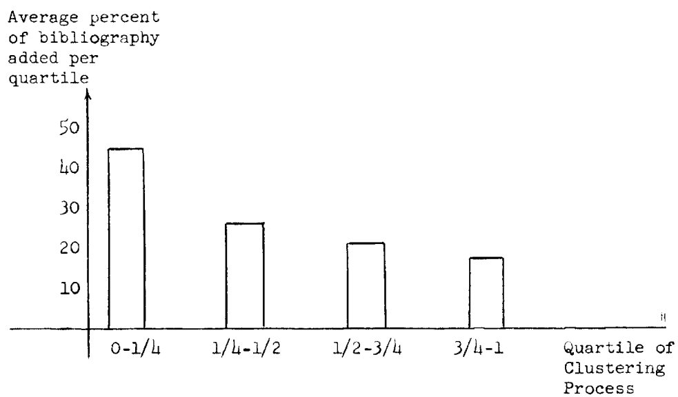
Fig. 9.44. Graph showing average percent of bibliography (or category) articles added during each quartile of the clustering process.
