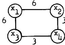
Fig. 4.5. Network containing no subset clusters.
