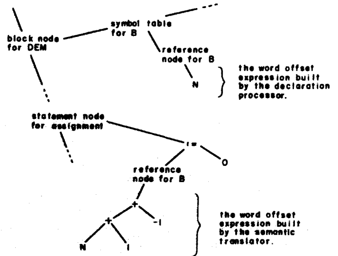
Figure 5—A simplified diagram showing the effects of subscripting
