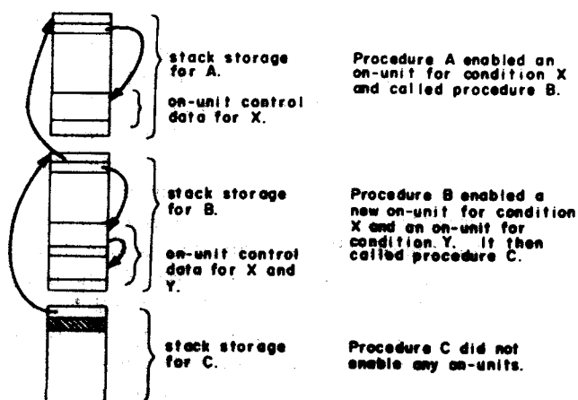
Figure 7—Stack storage and the signal mechanism A signal for condition X causes the signal mechanism to search back through the stack until it finds the first enabled on-unit for condition X.
