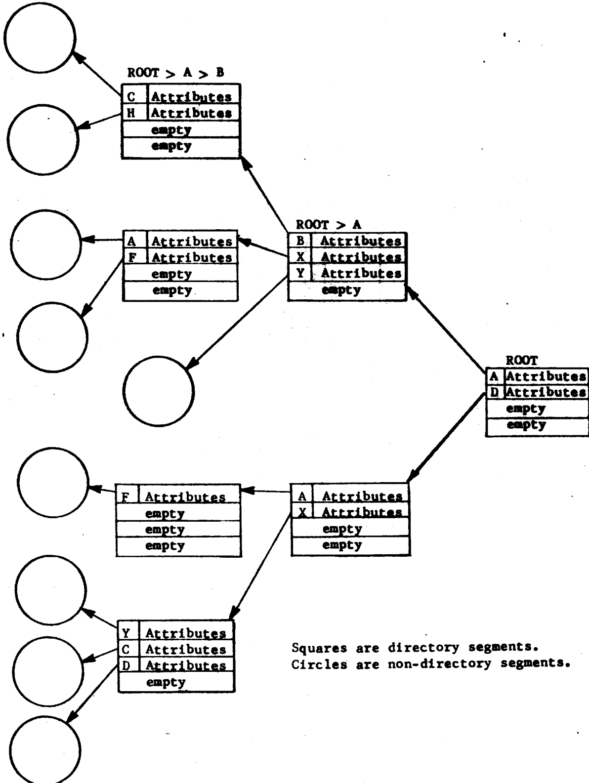
Figure 4. Directory Hierarchy
