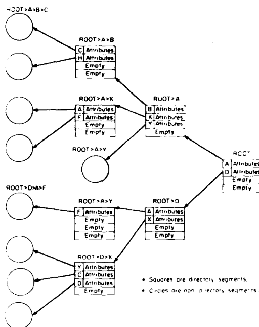
Fig. 4. Directory hierarchy.
