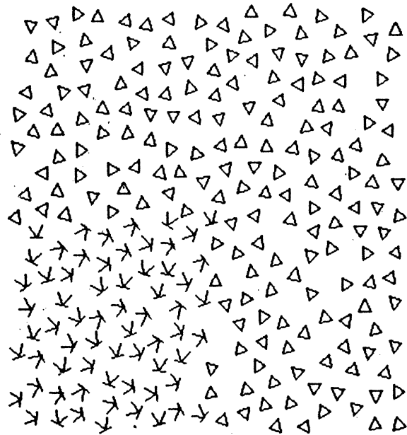
Figure 6.1 A discriminable texture. The lower left region can be seen immediately to have a different texture from the rest of the figure.
