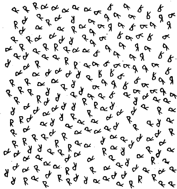
Figure 6.2 An indiscriminable texture. The figure initially appears homogeneous. Close inspection reveals that upper right region is composed of backward R's, while the remainder of figure is composed of forward R's [Julesz 1973].
