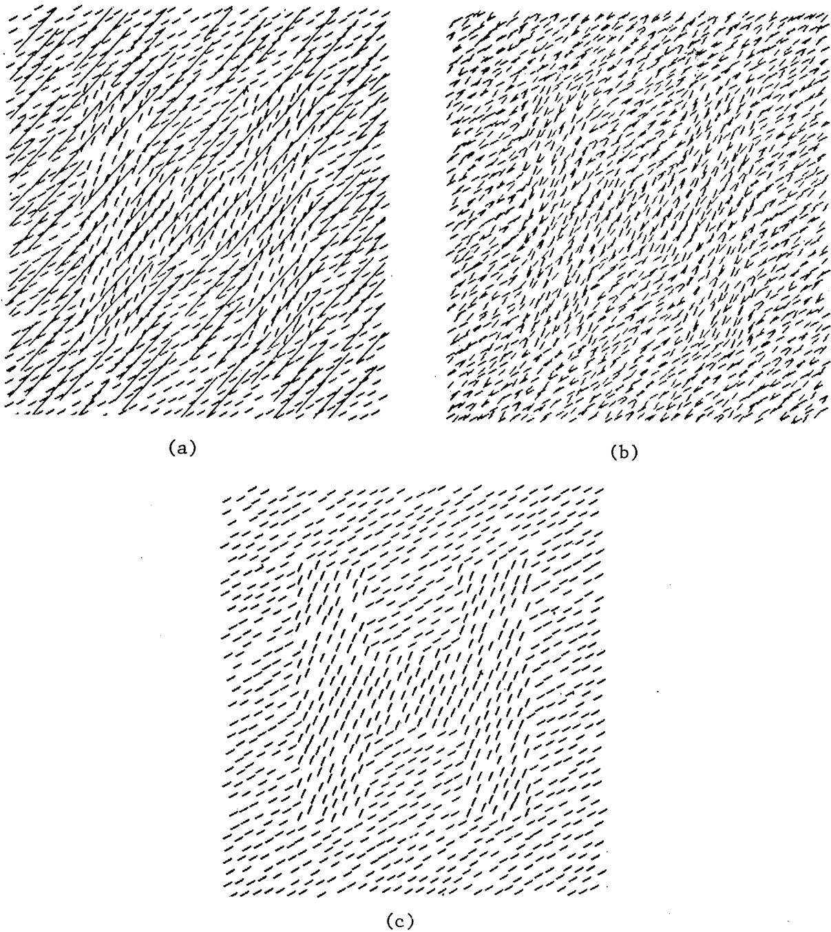
Figure 7.2 The creation of texture patterns (a) and (b) both begin with underlying pattern (c), which has line segments at 65^\circ inside the embedded region and at 25^\circ outside this region. Masking 45^\circ line segments nine times as long as those in pattern (c) and with one ninth the density (number/area) are added to complete pattern (a). Masking 45^\circ line segments of the same length and with the same density as pattern (c) are added to complete pattern (b). The embedded H in pattern (a) is easier to recognize than that in pattern (b); an effect that is accentuated at oblique or distant viewpoints. This result is difficult to explain if the raw intensity changes at various scales are the sole texture tokens.
