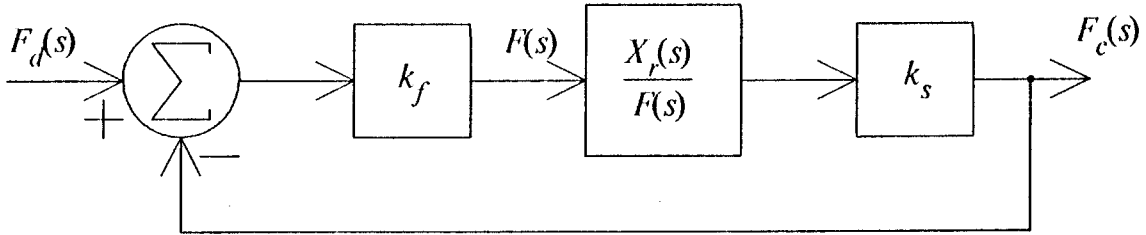
Figure 2: Block diagram for the controller of Figure 1.
