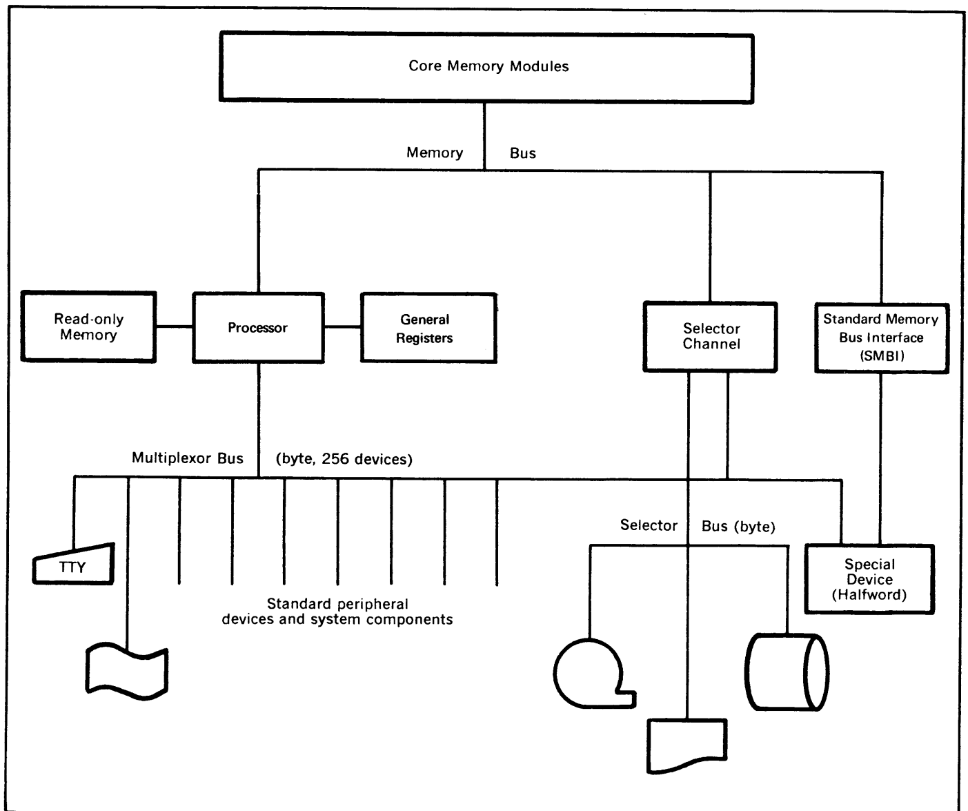
Figure 1-1. INTERDATA Digital Systems, Typical Block Diagram
