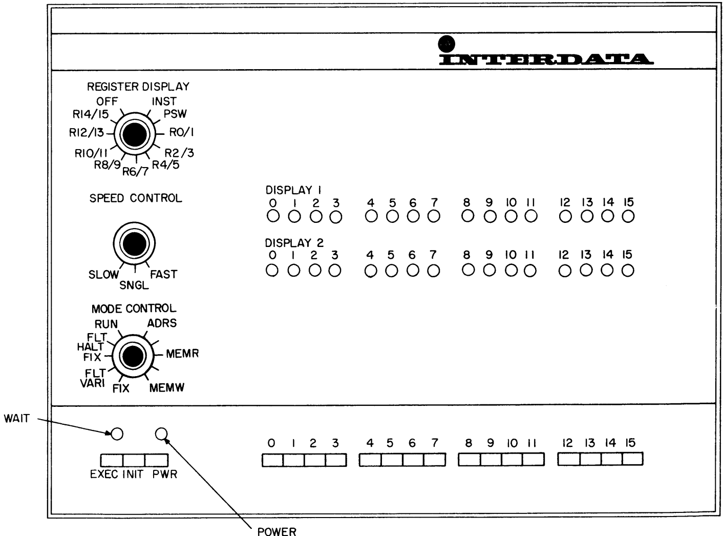
Figure 3-1. Display Panel
