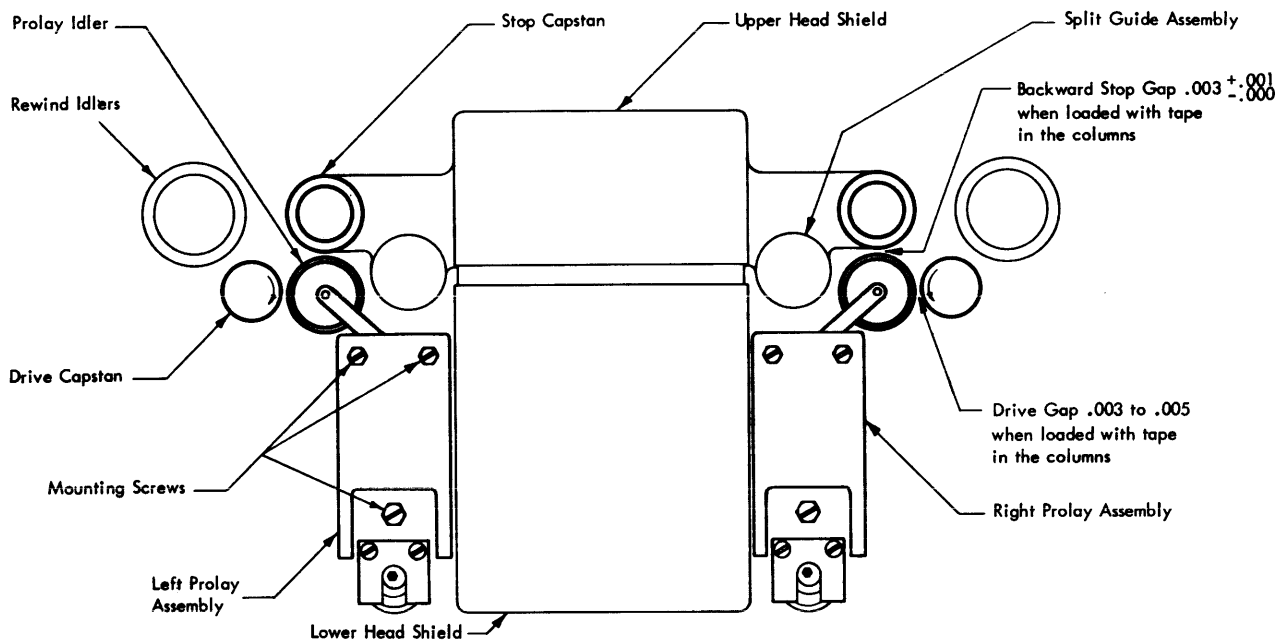
Figure 42. Prolay Drive and Stop Gap Adjustments
