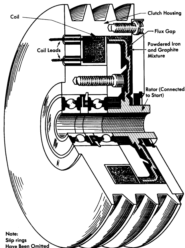
Figure 53. Magnetic Clutch
