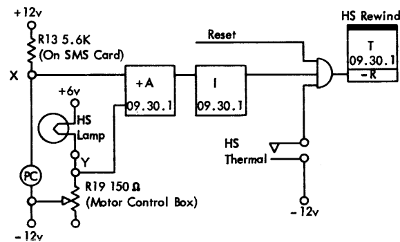
Figure 77. High-Speed Rewind Lamp
