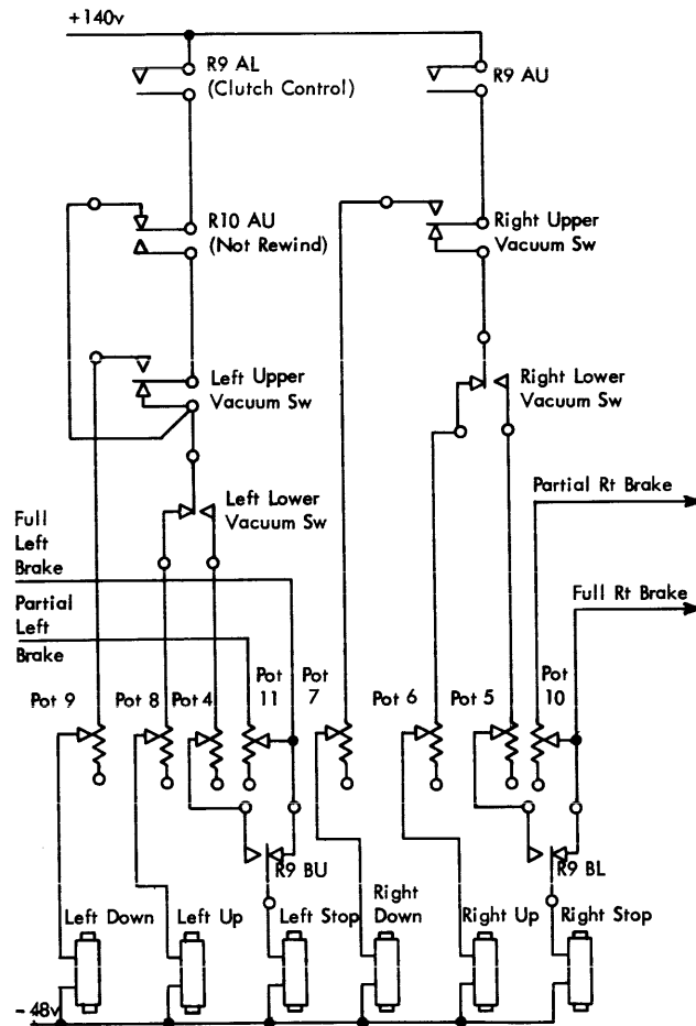
Figure 67. Clutch and Vacuum Control Circuitry
