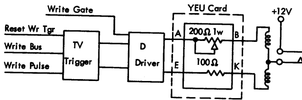
Figure 105. Write Current Compensation
