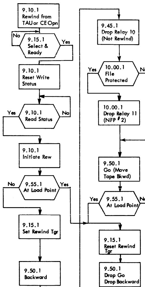
Figure 88. Rewind Flow Chart (Low Speed)
