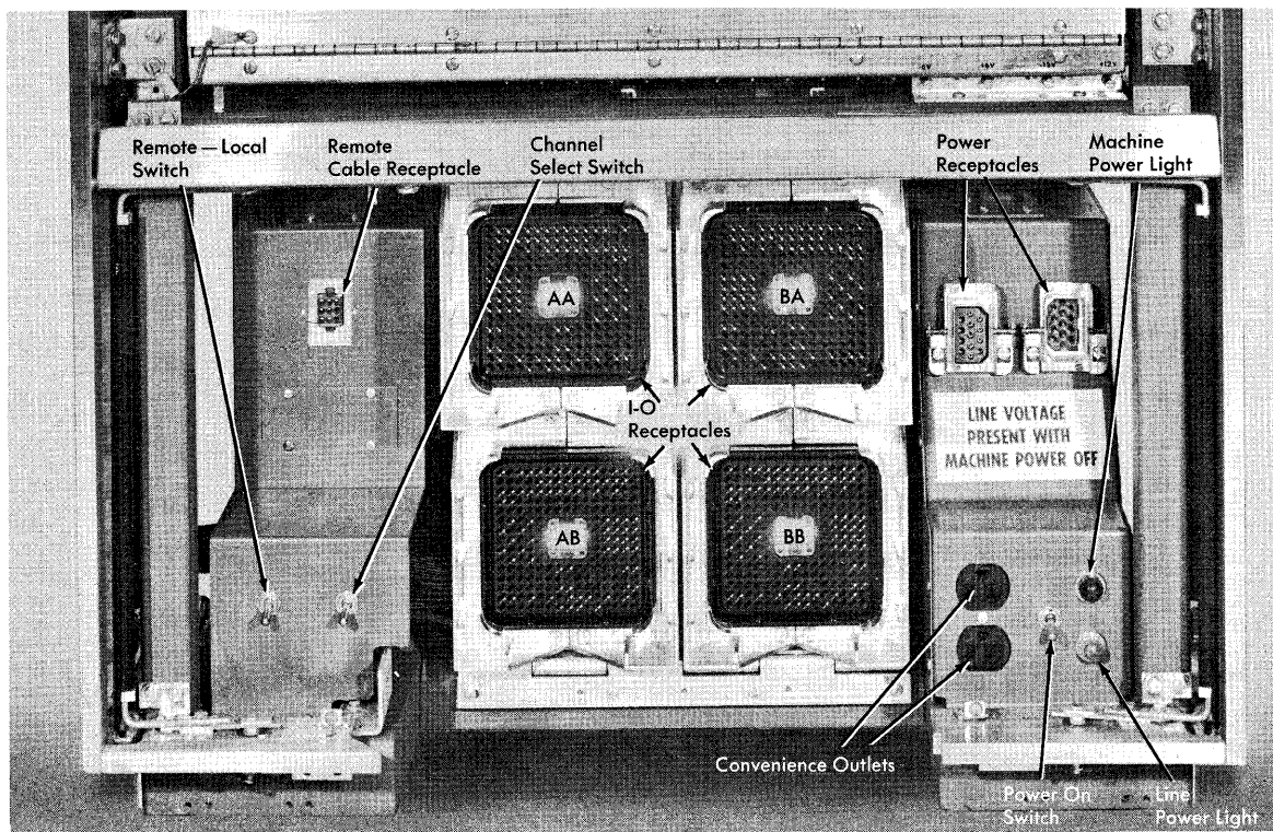
Figure 99. Tape Switching Connectors
