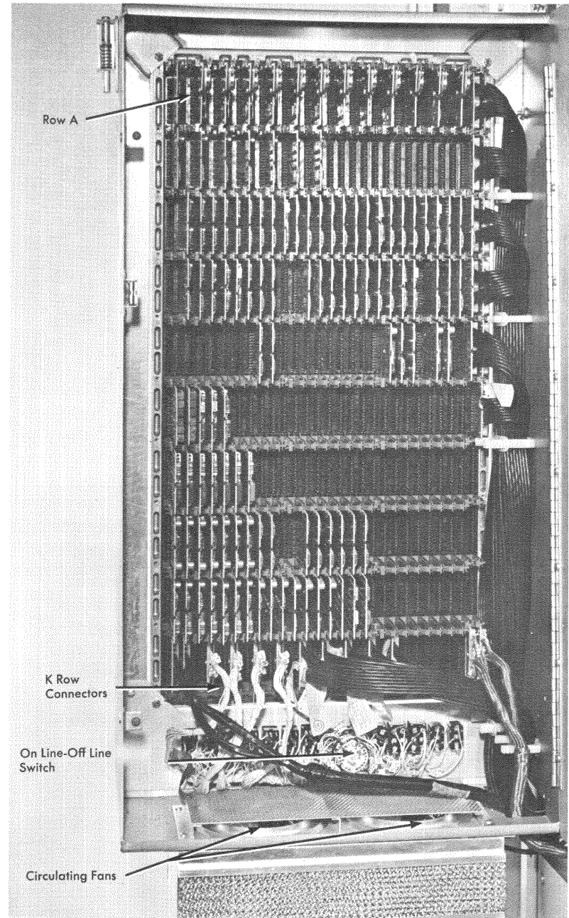
Figure 7A. Read Logic Panel (Card Side)
