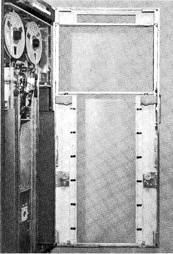
Figure 60. Sliding Glass Assembly
