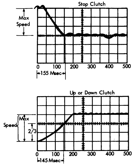
Figure 56. Typical Clutch Response Curves
