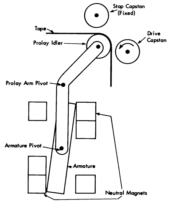
Figure 37. Right Prolay with Neutral Magnets Energized
