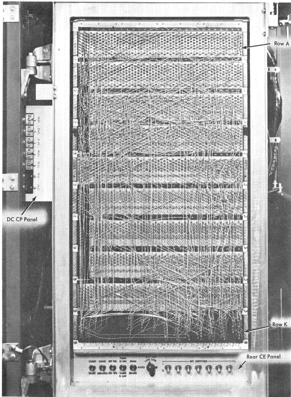
Figure 7. Rear Logic Panel
