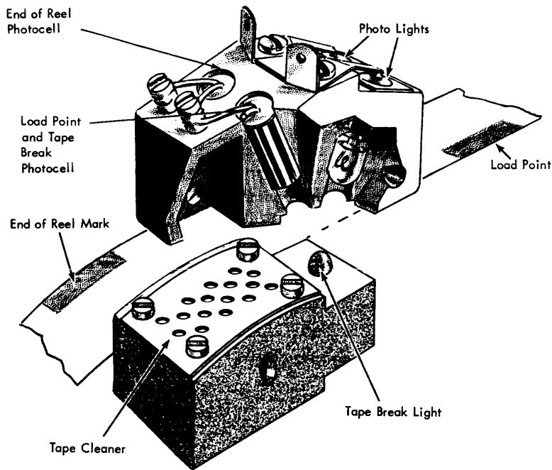
Figure 31. Photocell Sensing
