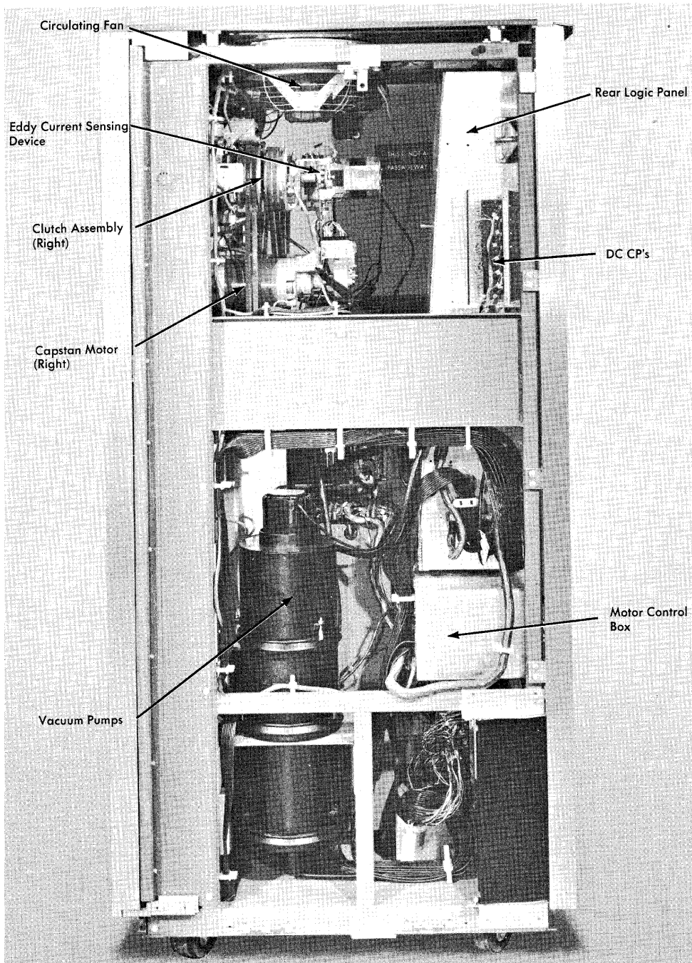
Figure 18. Tape Unit, Right Side
