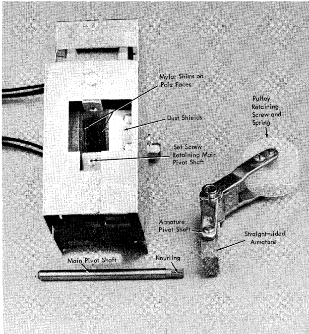
Figure 46. Removable Arm Prolay
