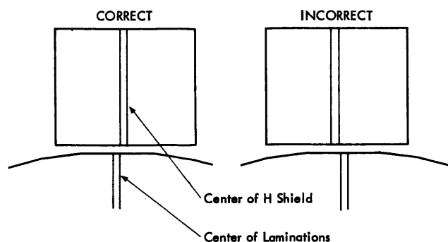
Figure 26. H-Shield Adjustment
