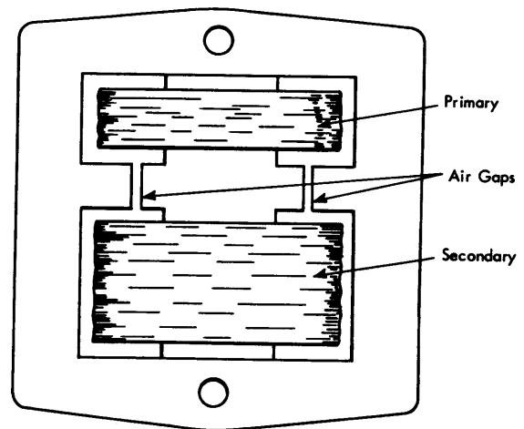
Figure 95. Ferroresonant Regulator Transformer
