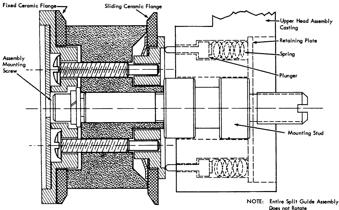
Figure 29. Split Guide Assembly
