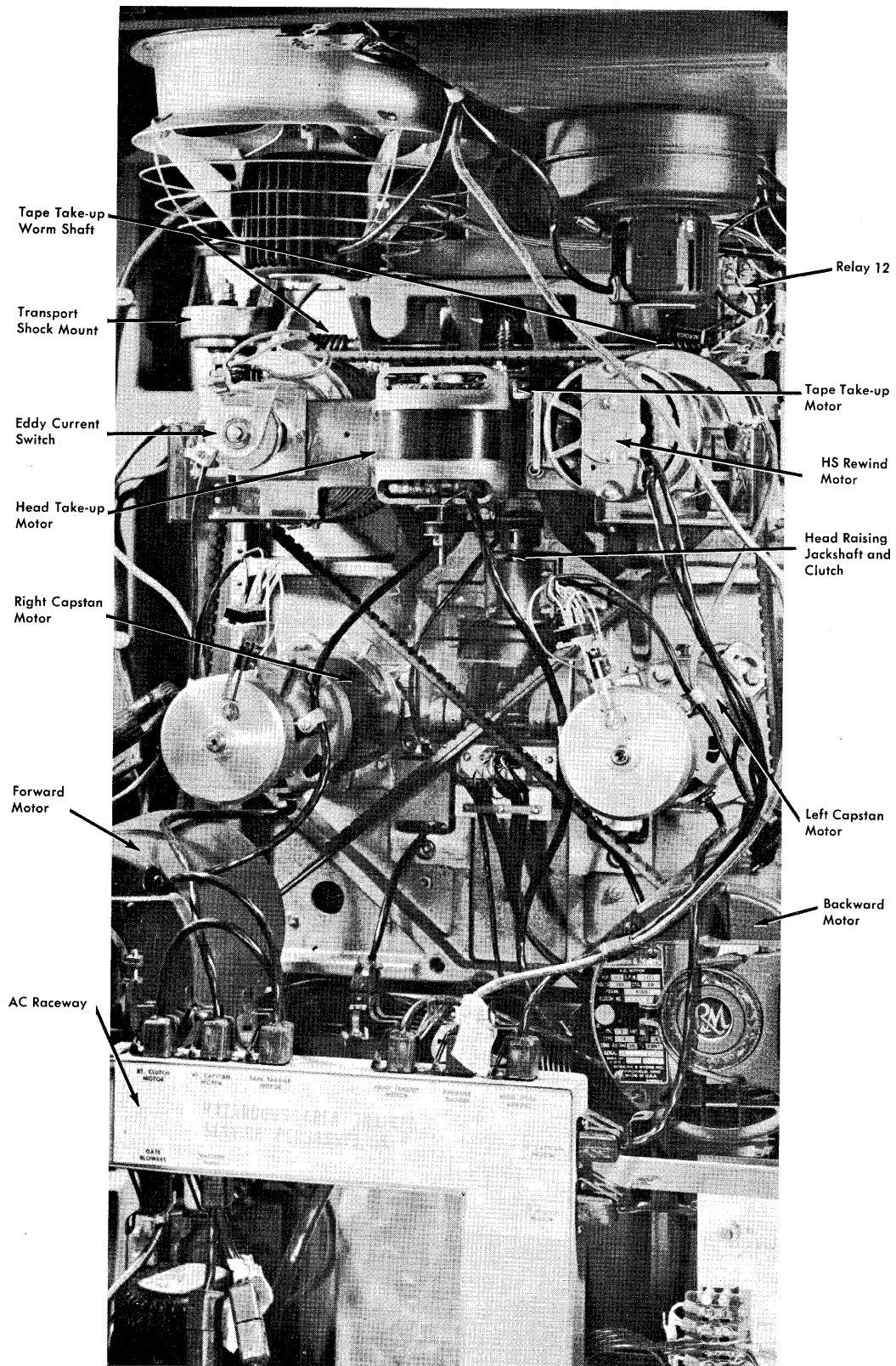
Figure 54. Drive Mechanisms
