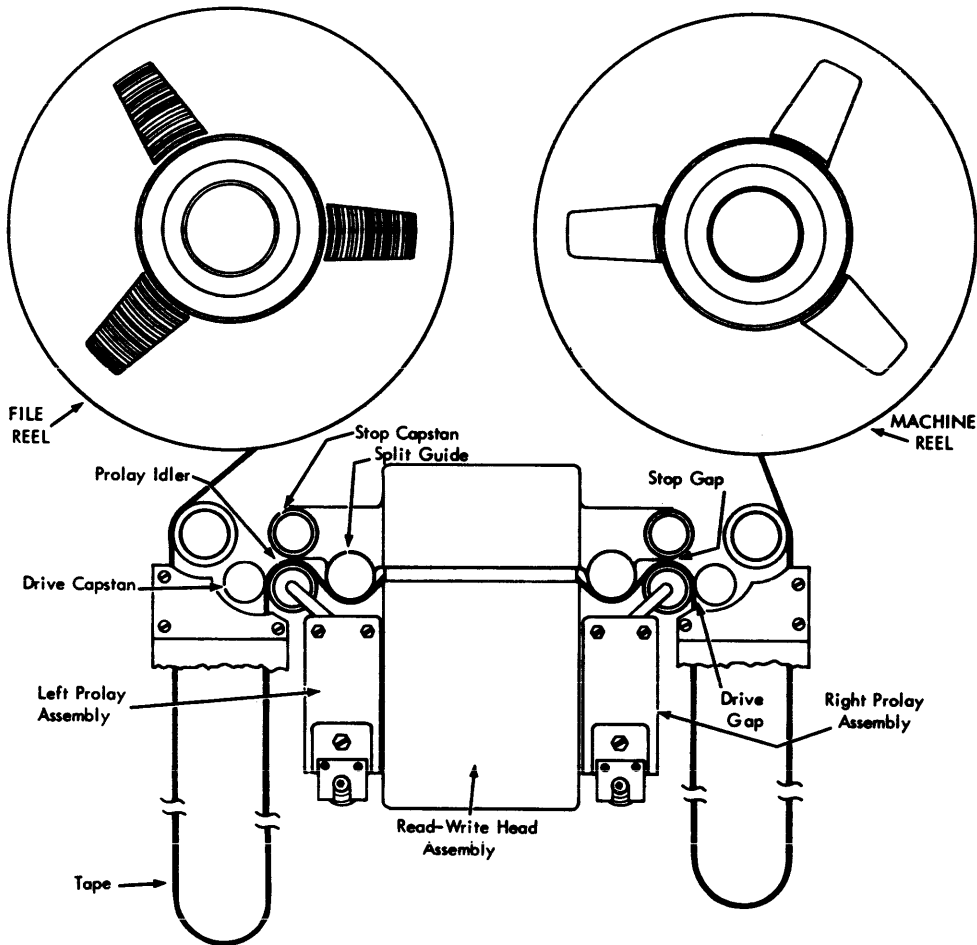
Figure 35. Path of Tape through Magnetic Tape Unit
