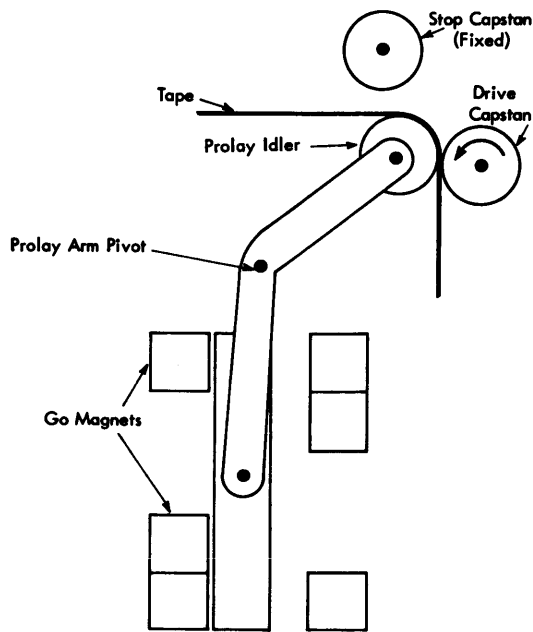
Figure 38. Right Prolay with go Magnets Energized
