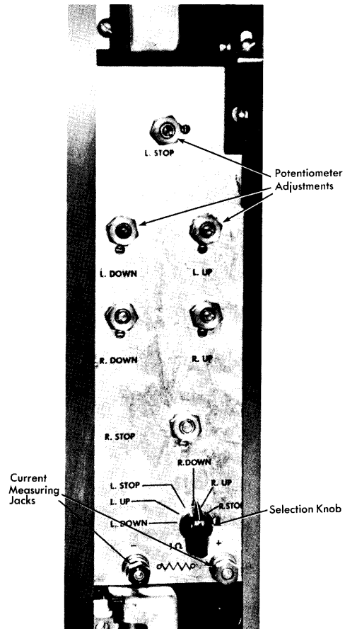
Figure 57. Clutch Adjustment Panel
