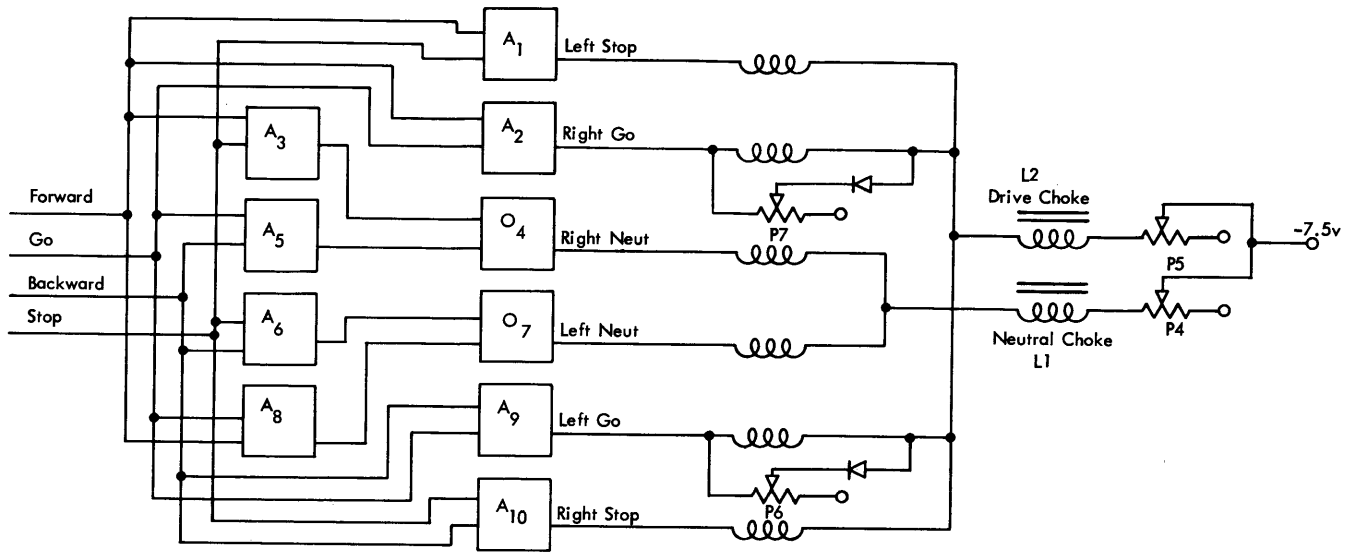
Figure 65. Prolay Control Logic
