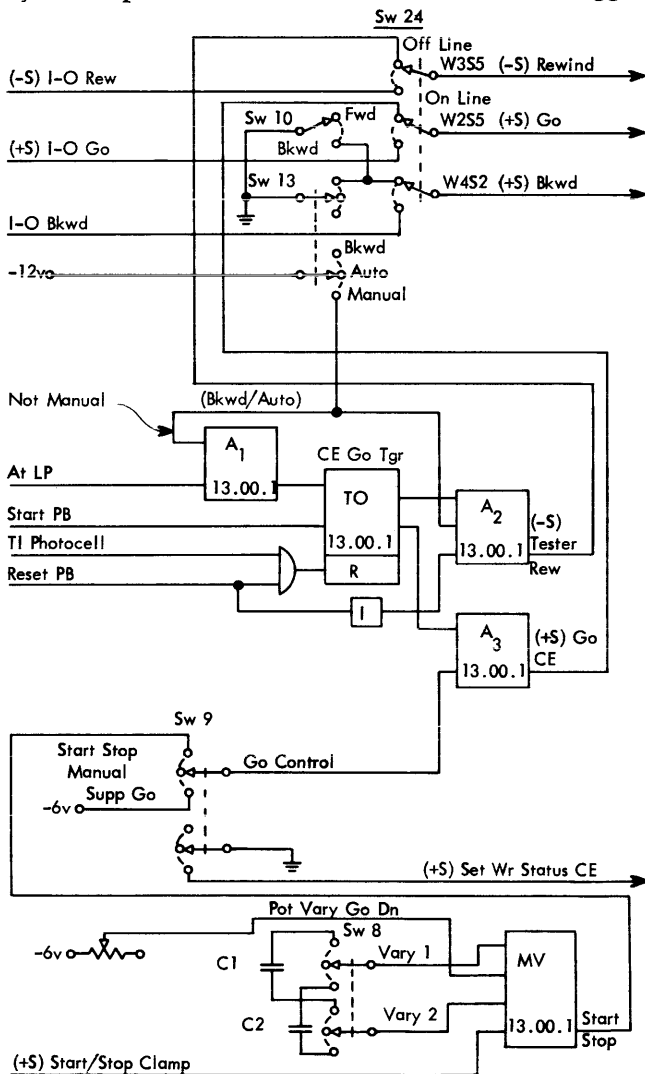
Figure 6. CE Tester Control
