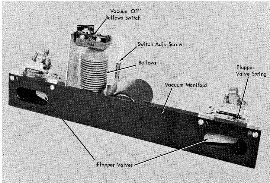
Figure 51. Vacuum Manifold Assembly
