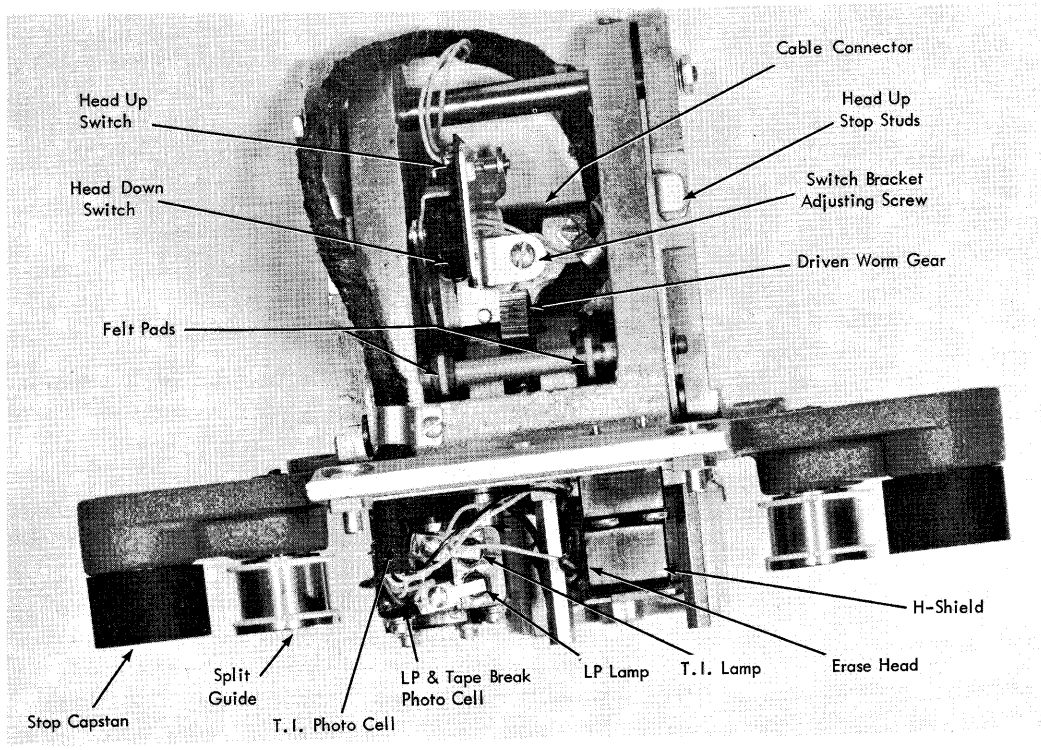
Figure 22. Head Assembly, Top View
