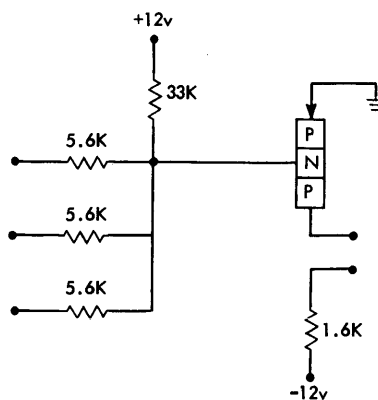
Figure 112. CD— Circuit (Extender)
