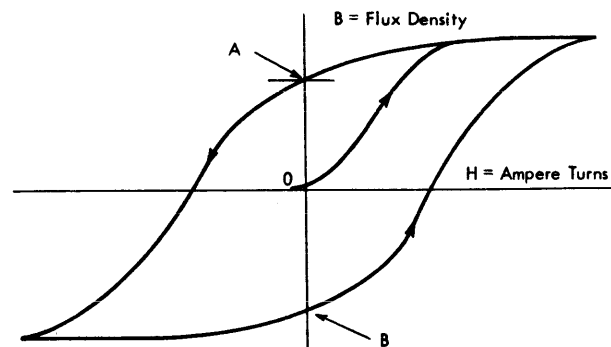
Figure 2. B-H Curve
