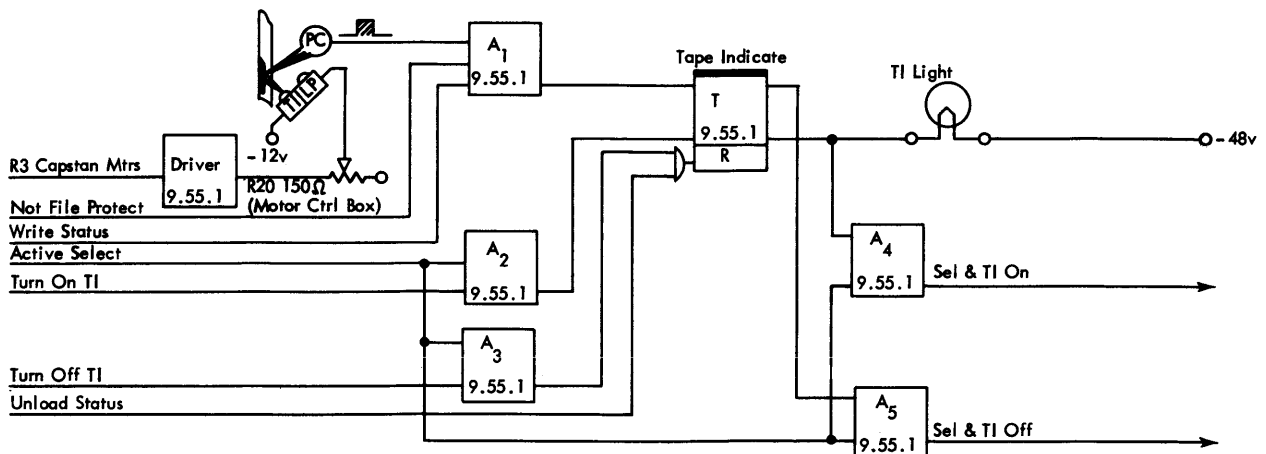
Figure 76. Tape Indicate Logic
