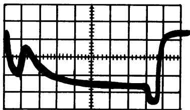
Writing continuous 1's 5v/cm 2 \mu s/cm DC input Internal sync
