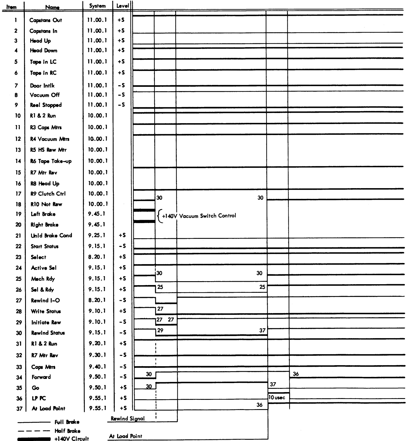
Figure 89. Rewind Sequence Chart (Low Speed)
