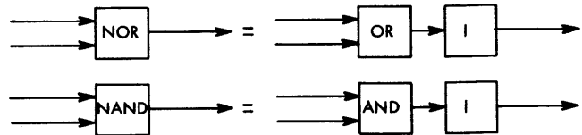
Figure 10. NOR Circuit Equivalents
