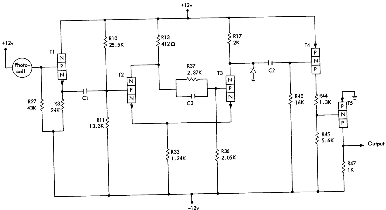
Figure 109. AC Photocell Circuit
