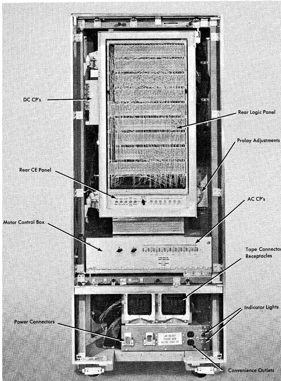
Figure 20. Tape Unit, Rear
