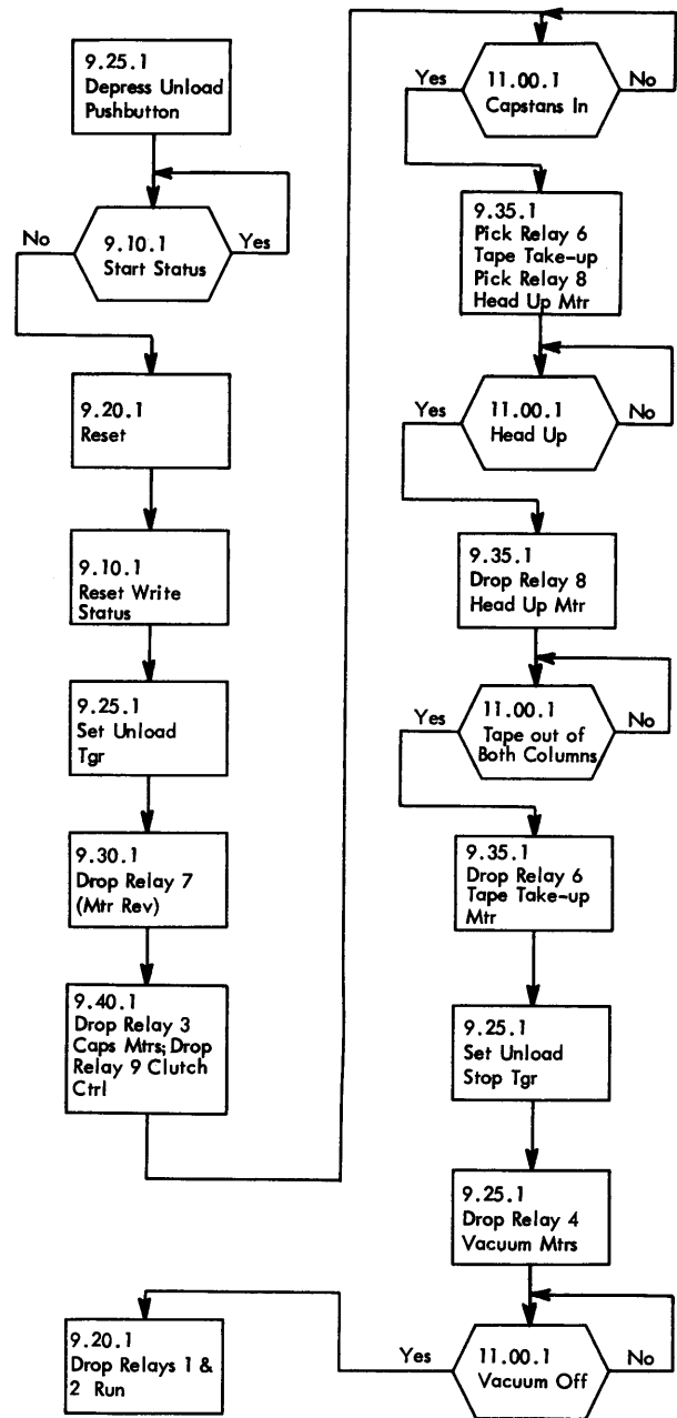
Figure 85. Unload Flow Chart
