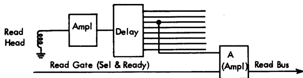
Figure 70. Read Circuit
