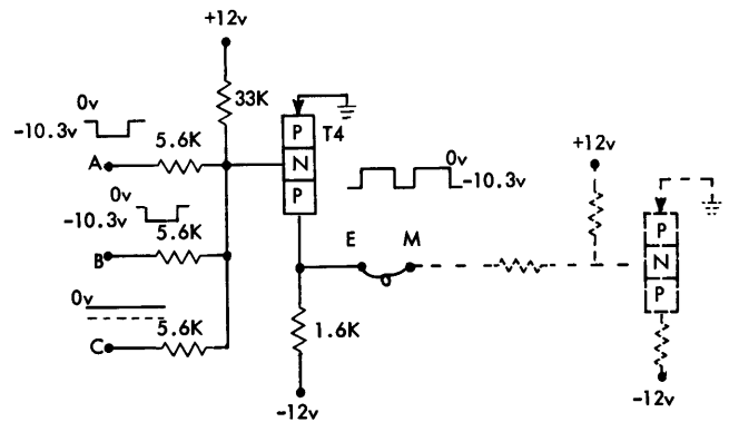
Figure 111. CD— Circuit Configuration
