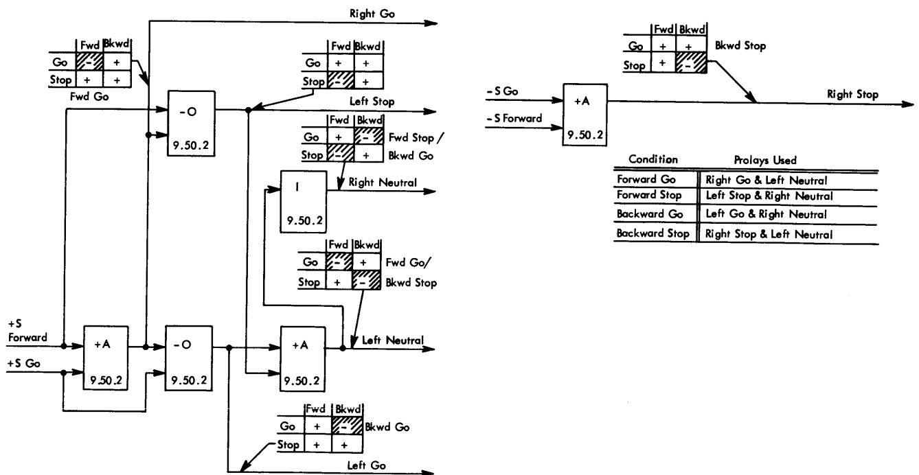
Figure 66. Prolay Control Circuit
