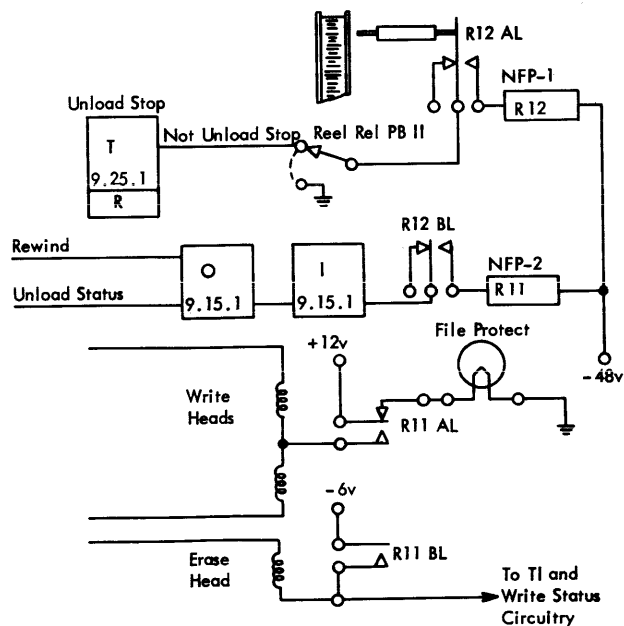
Figure 69. File Protection
