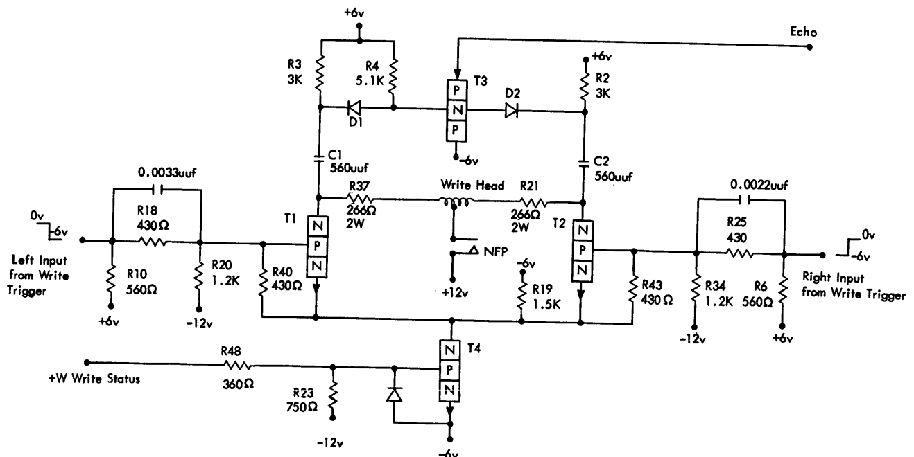
Figure 108. Driver and Echo Pulse Amplifier
