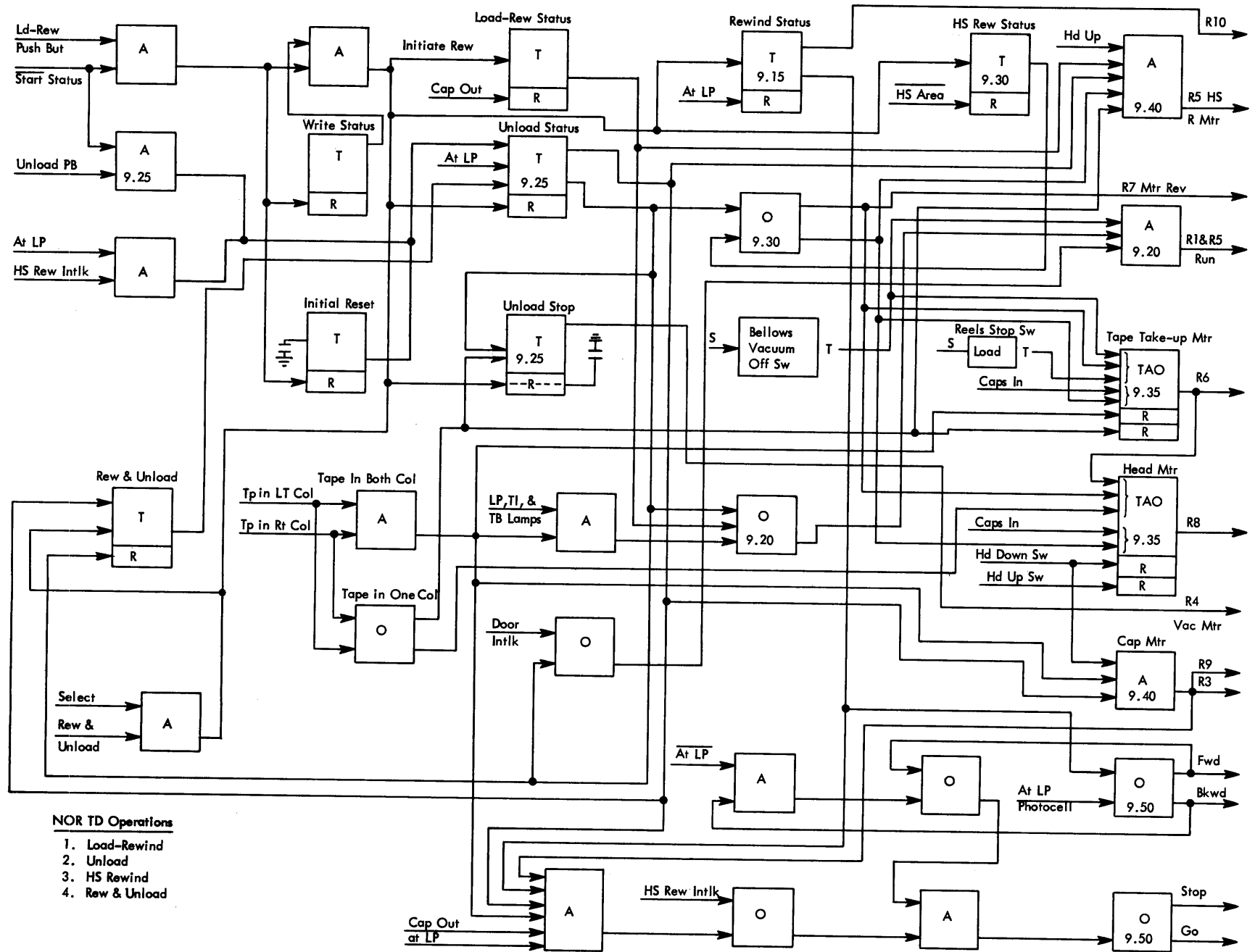
Figure 93. Over-all Condensed Logic
