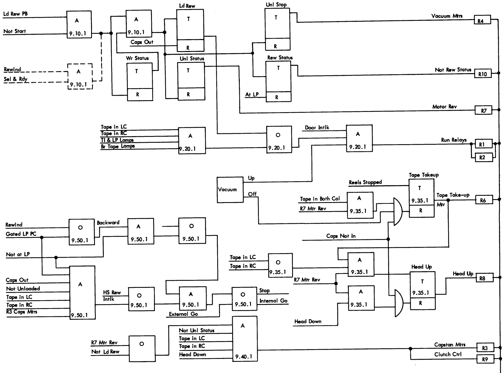
Figure 82. Rewind and Load-Rewind Condensed Logic (Low Speed)
