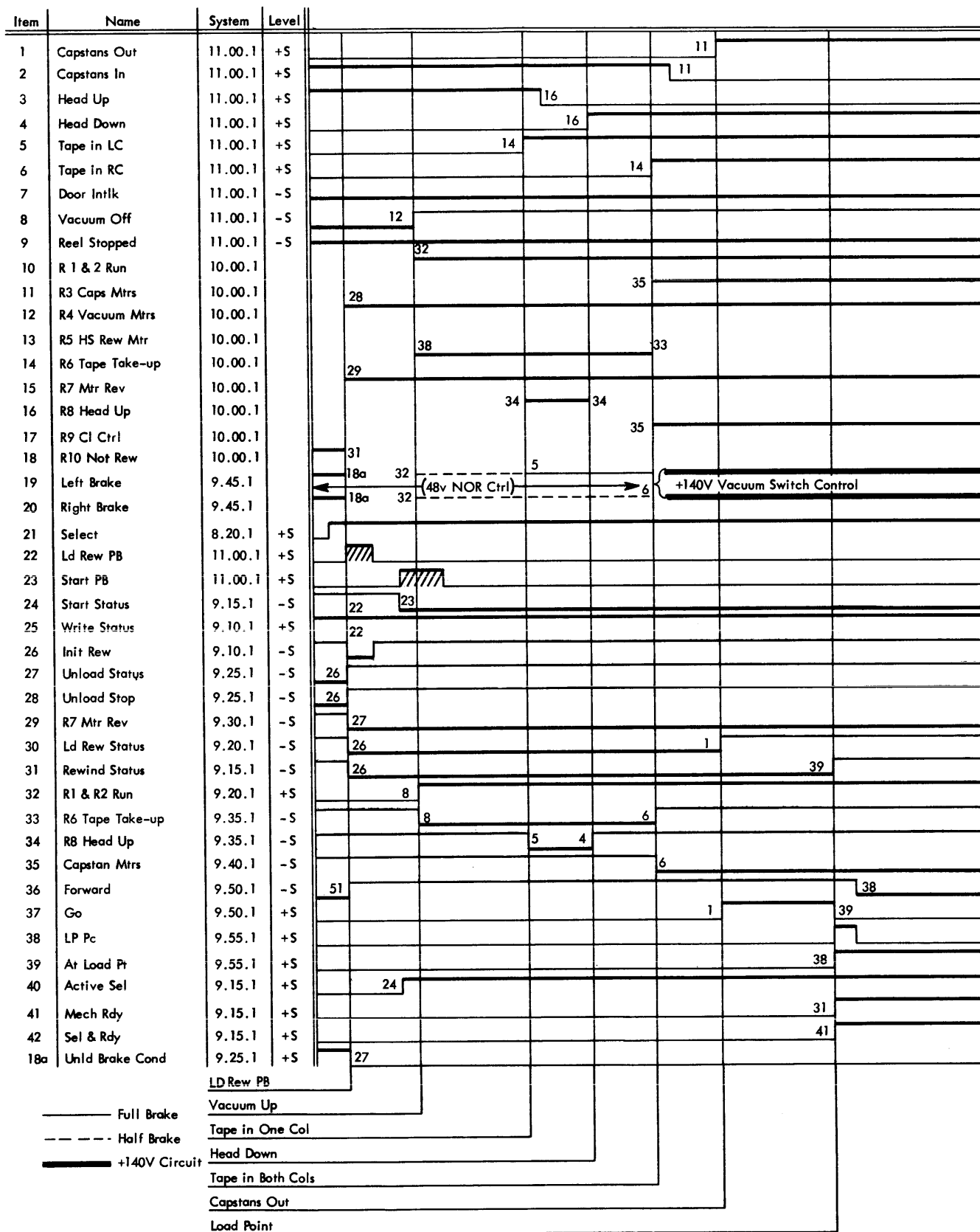
Figure 81. Load-Rewind Sequence Chart (Low Speed)
