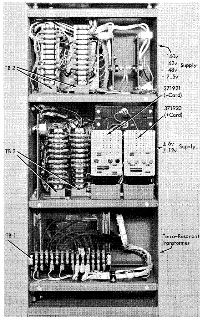
Figure 98. Phase III Power Supply Unit
