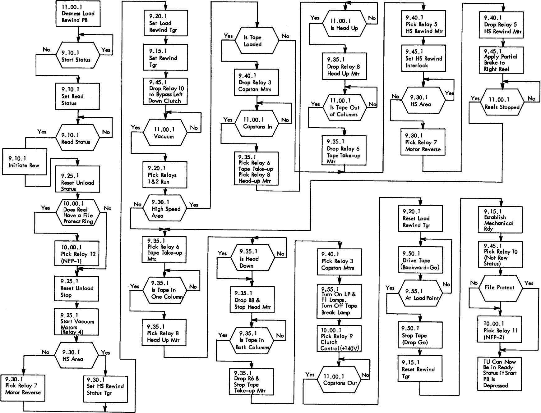
Figure 80. Load-Rewind Flow Chart
