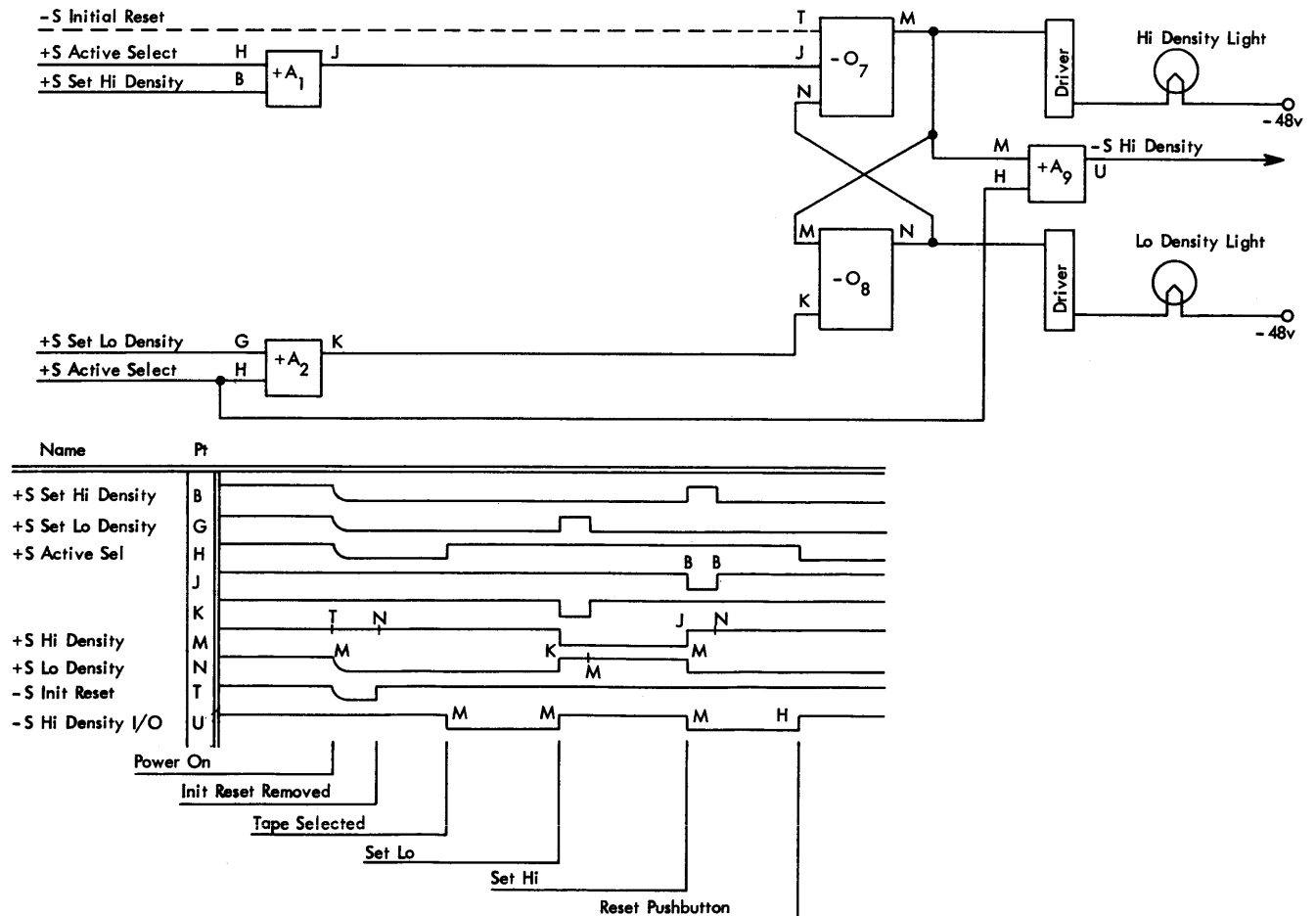
Figure 73. High-Low Density (Reset and External Control)
