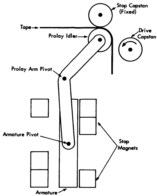
Figure 36. Right Prolay with Stop Magnets Energized
