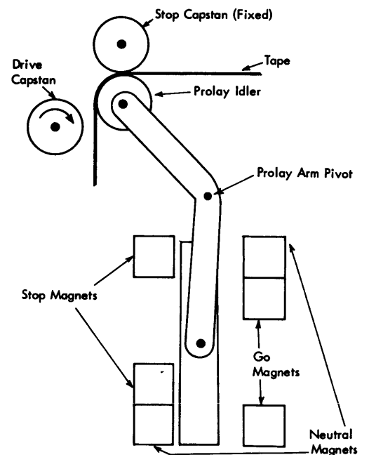
Figure 39. Left Prolay Showing Position of Magnets
