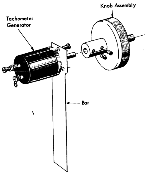
Figure 55. Tachometer Assembly
