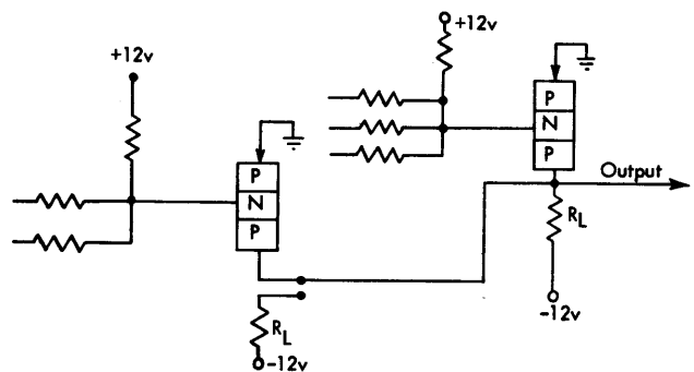
Figure 13. NOR Extender Circuit
