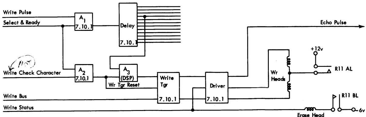
Figure 71. Write Circuit
