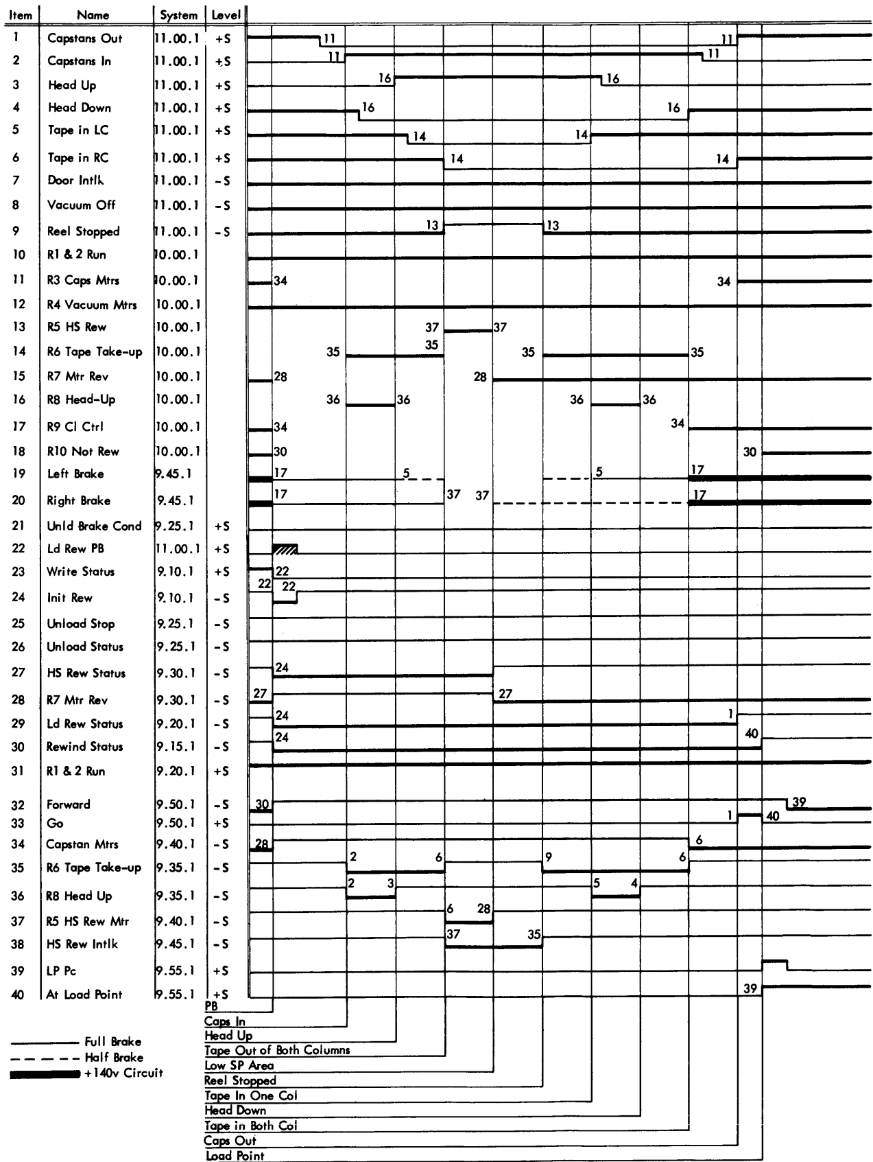
Figure 83. Load-Rewind Sequence Chart (High Speed)
