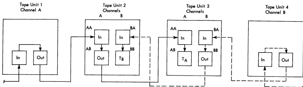
Figure 100. Receptacles and Cable Connectors with Tape Switching
