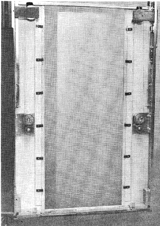
Figure 61. Sliding Drum Spring Drum Assembly
