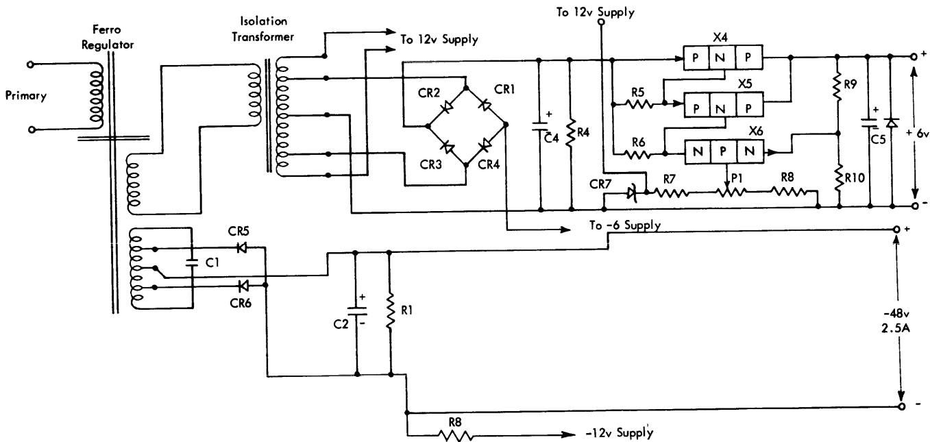
Figure 96. Phase III Power Supply
