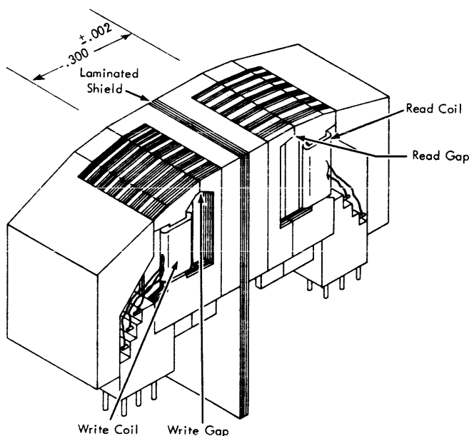
Figure 24. Two-Gap Read-Write Head
