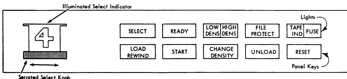
Figure 4. Operator's Panel
