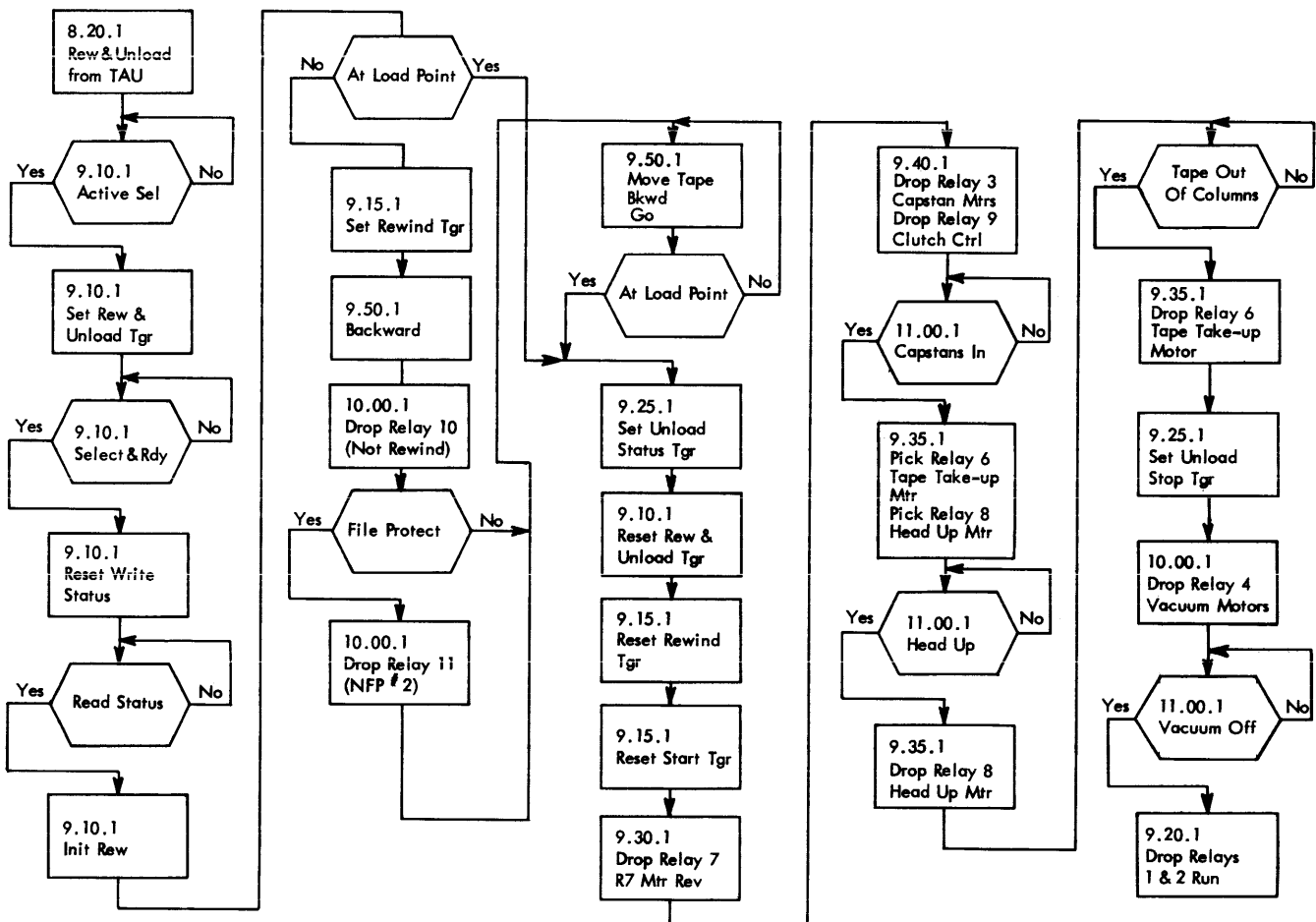
Figure 90. Rewind and Unload Flow Chart (Low Speed)
