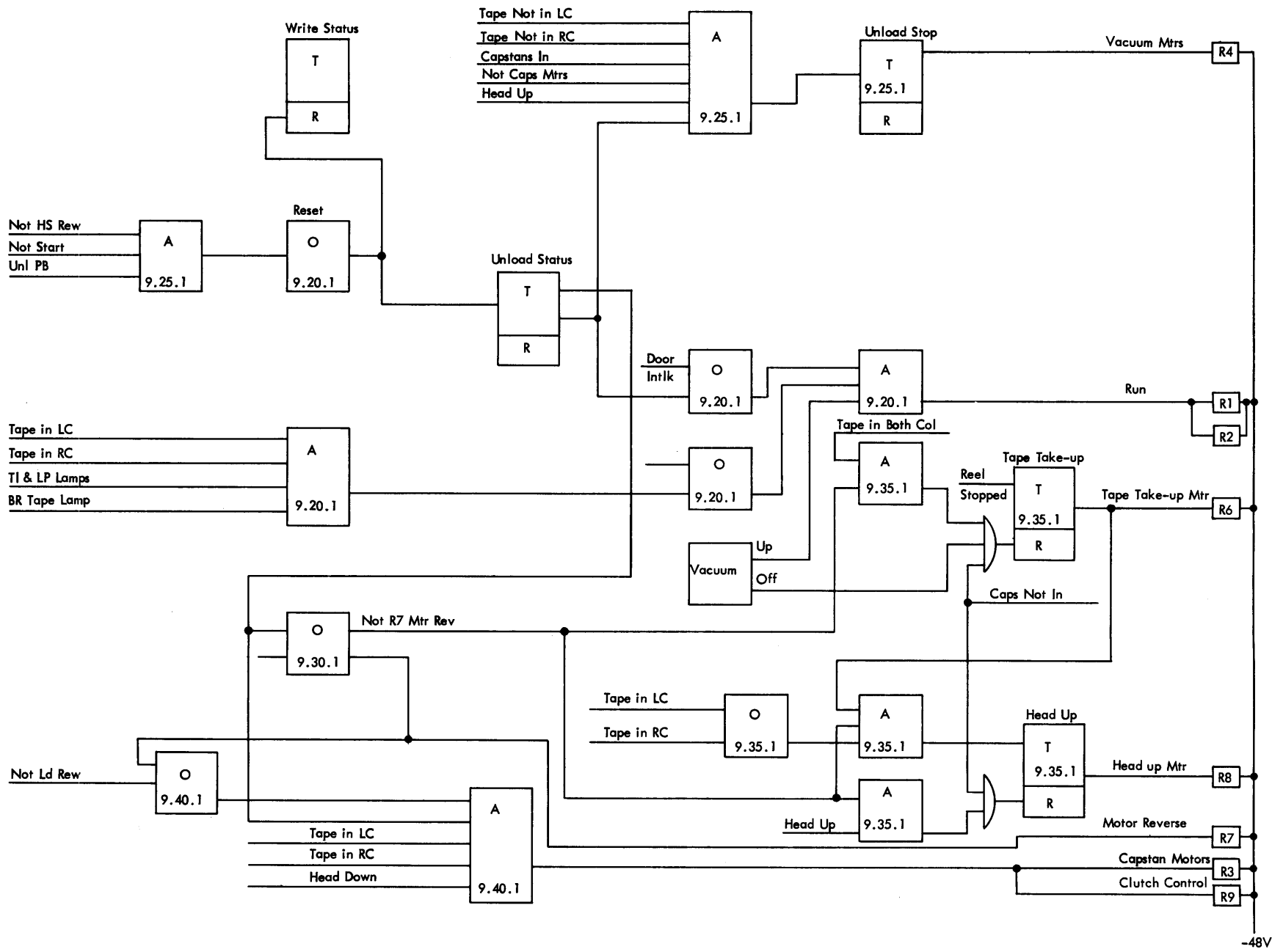
Figure 87. Unload Condensed Logic
