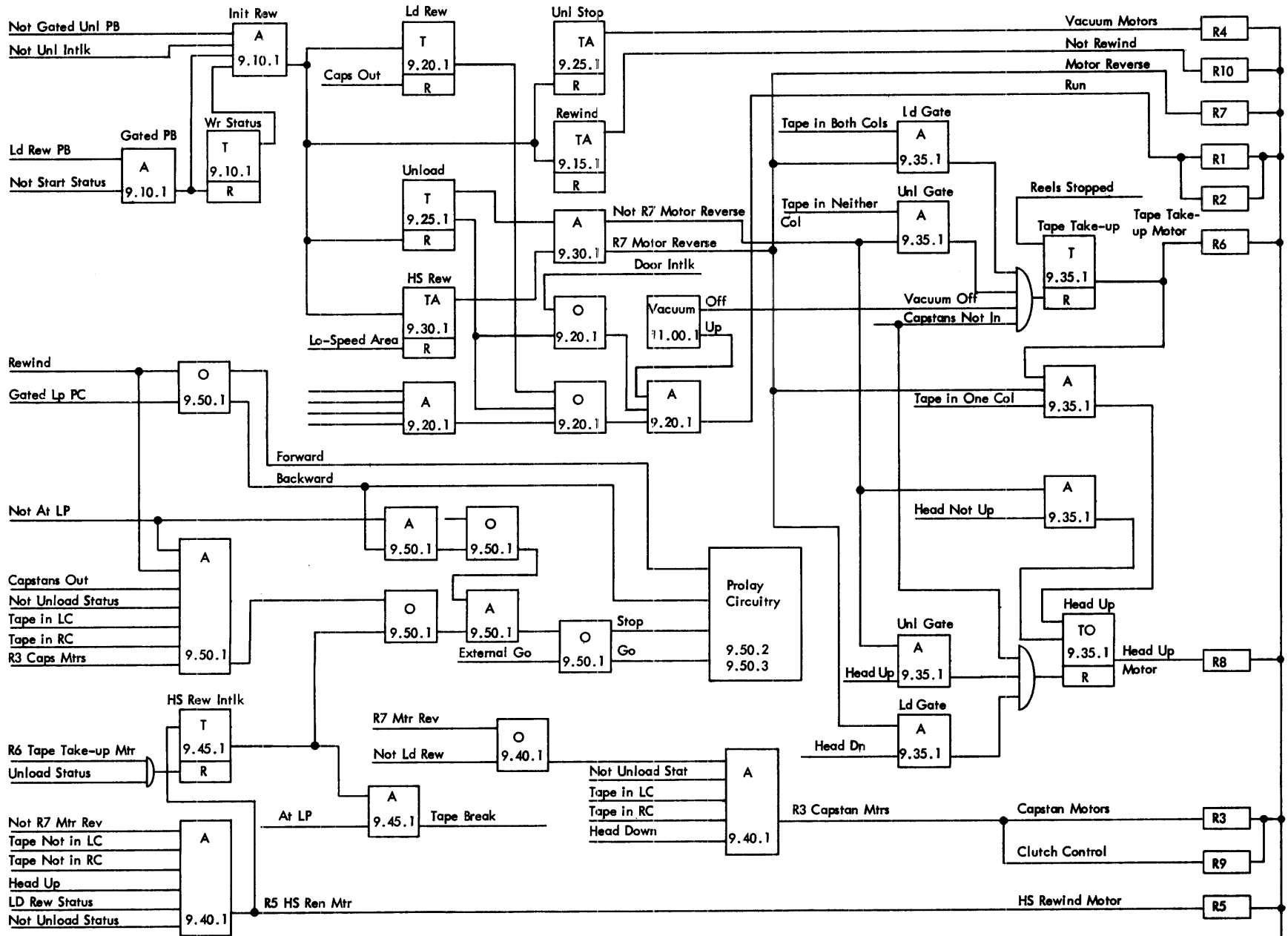
Figure 84. Load-Rewind Condensed Logic (High Speed)
