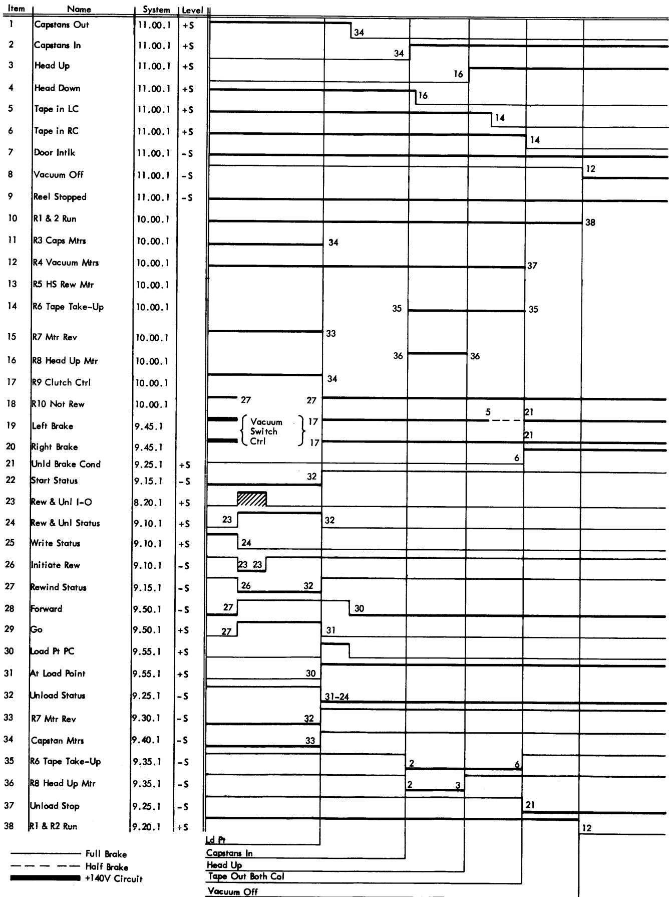
Figure 91. Rewind and Unload Sequence Chart (Low Speed)
