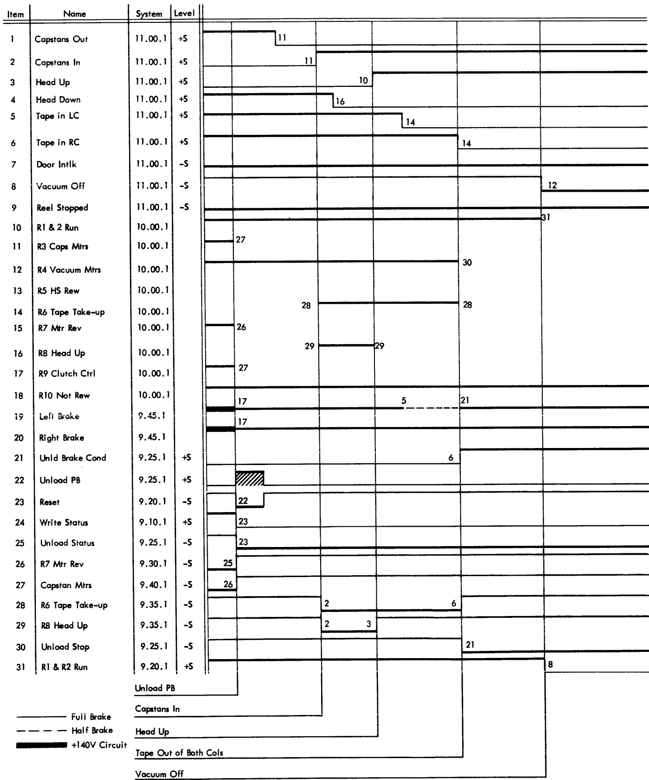
Figure 86. Unload Sequence Chart
