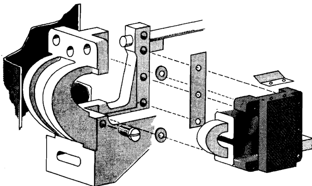
Figure 40. Shimmed Prolay
