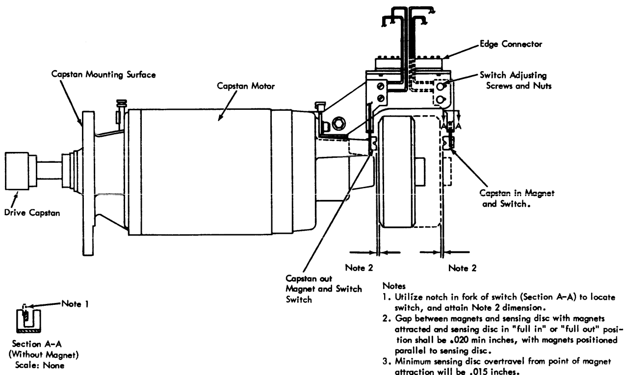
Figure 49. Drive Capstan Assembly
