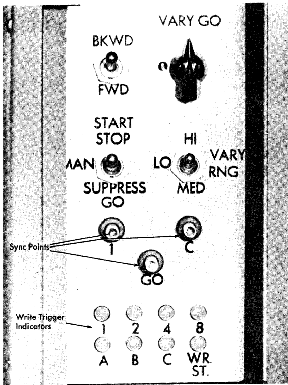
Figure 8. Front CE Panel
