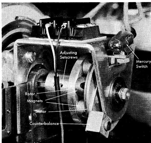
Figure 59. Eddy Current Sensing Device
