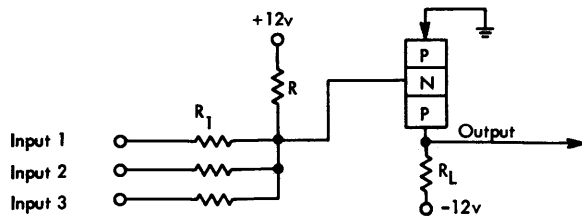
Figure 12. Three-Legged NOR Circuit
