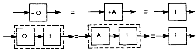
Figure 11. One-Legged NOR Inverter
