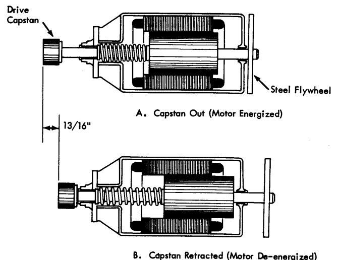
Figure 48. Capstan Drive Motor
