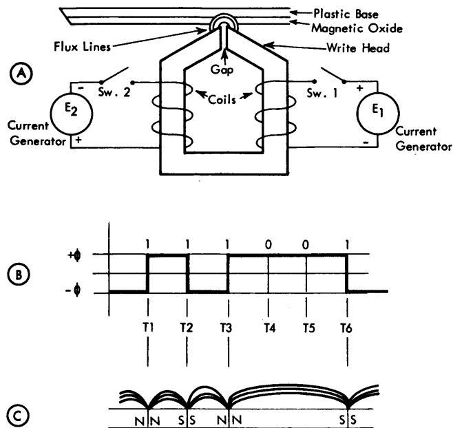
Figure 3. Method of Writing on Magnetic Tape (NRZI)
