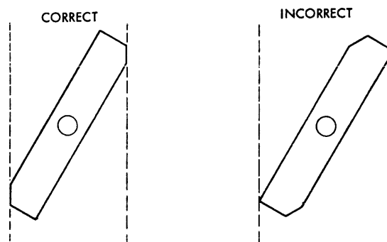
Figure 47. Prolay Armature, Reassembly
