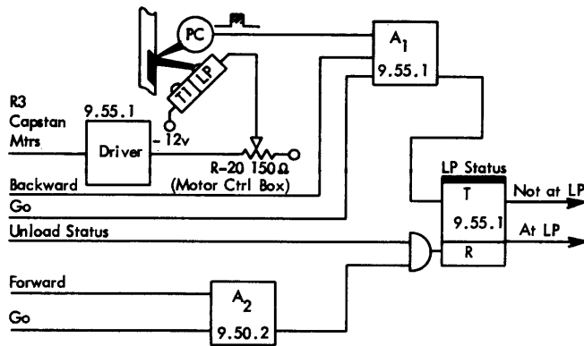
Figure 75. Load Point Logic
