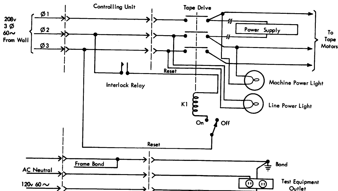
Figure 94. Tape Unit Power
