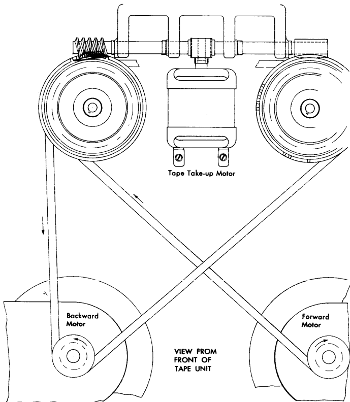
Figure 52. Drive Motors and Pulleys
