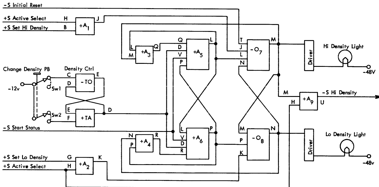
Figure 72. High-Low Density
