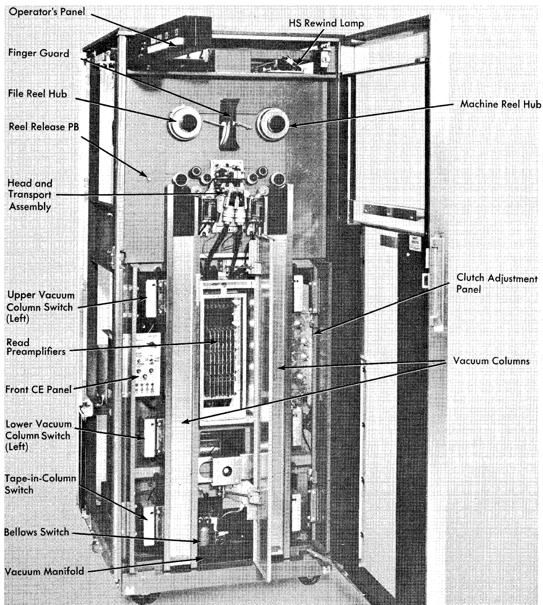
Figure 17. Tape Unit, Front
