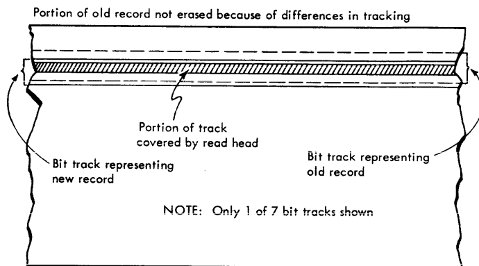
Figure 25. Write-Wide, Read-Narrow Concept
