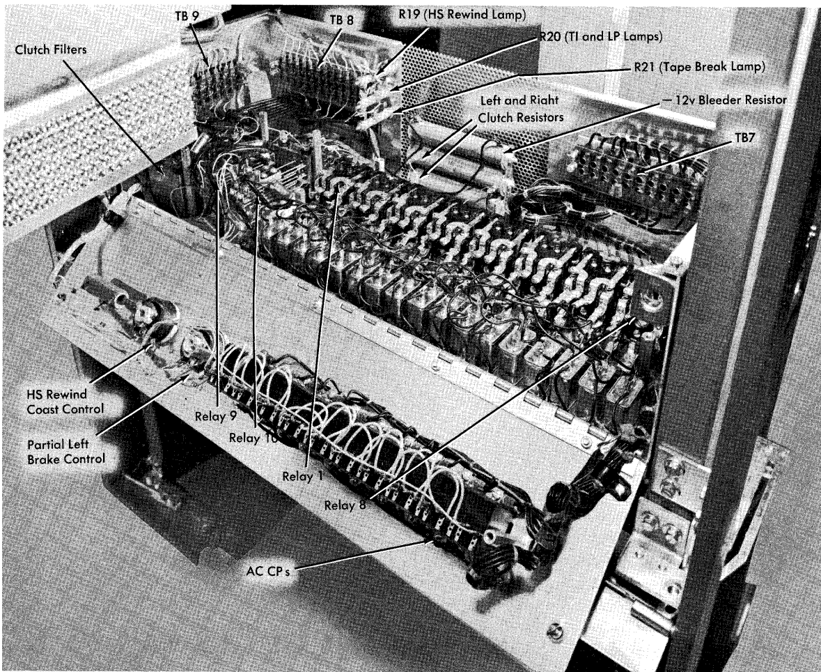
Figure 32. Motor Control Box
