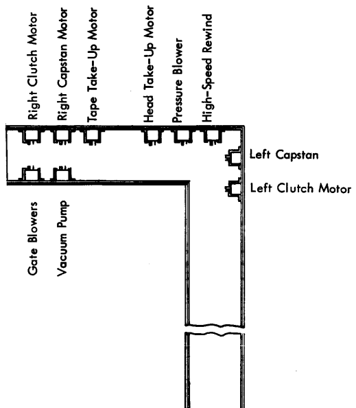
Figure 63. AC Raceway Plug Locations
