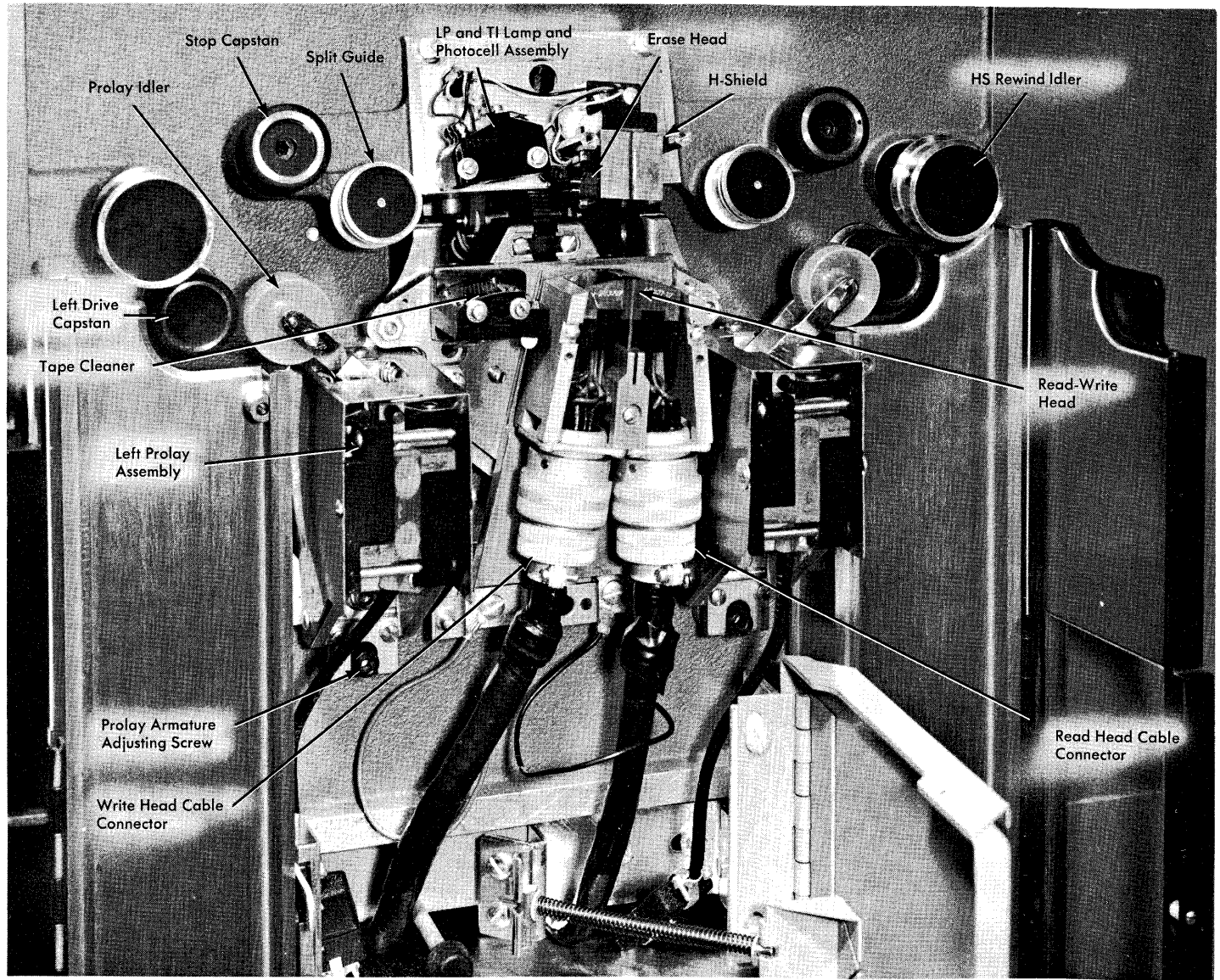
Figure 43. Read-Write Head and Transport Assembly
