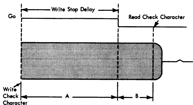
Figure 45. Stop Envelope
