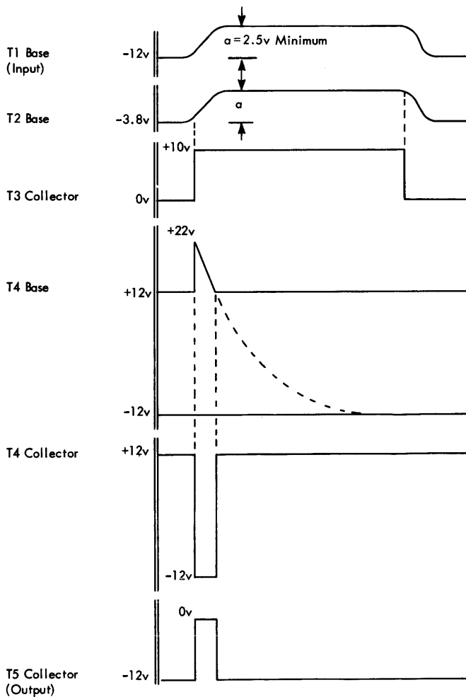
Figure 110. AC Photocell Wave Shapes
