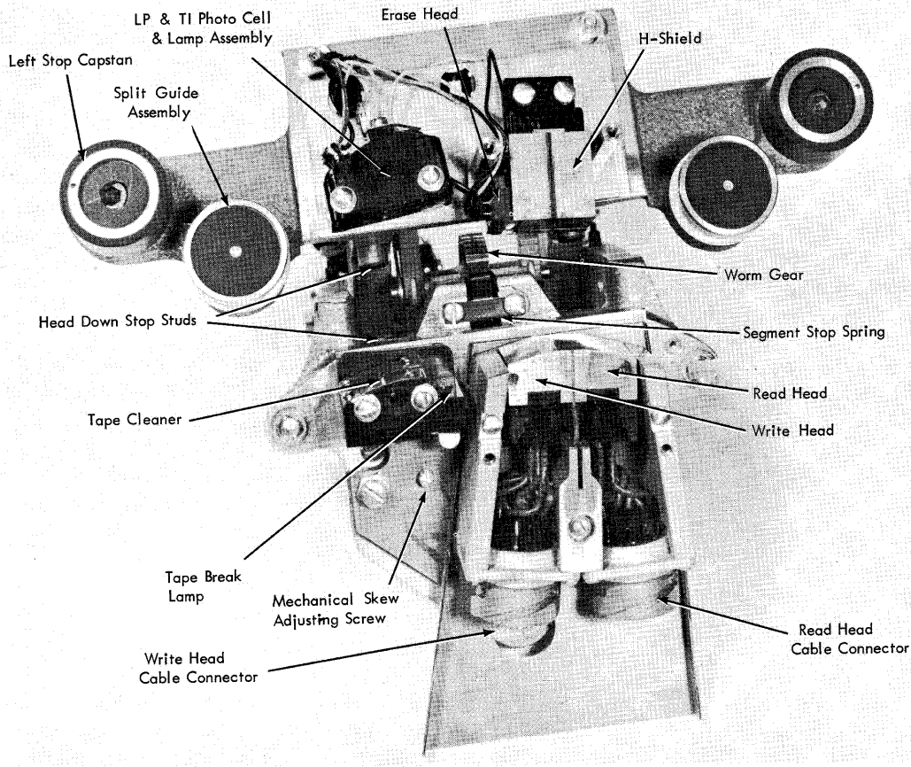
Figure 21. Head Assembly, Front View
