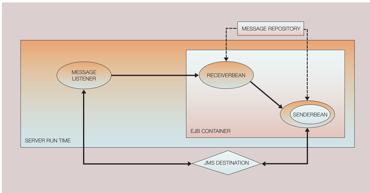
Figure 5 Container-managed messaging
