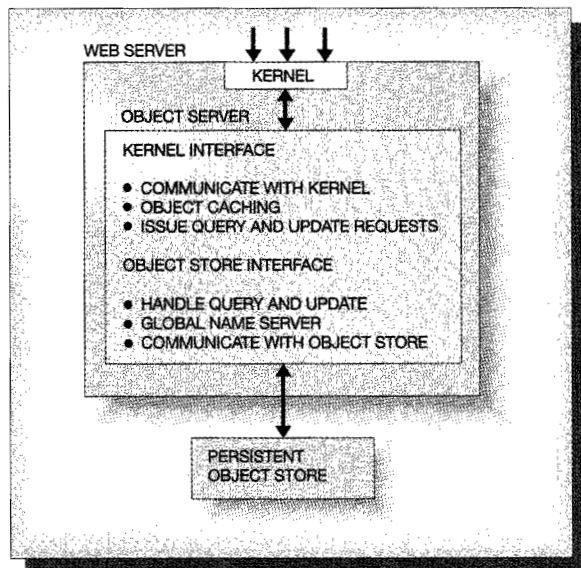
Figure 3 Bookshelf repository subsystems
