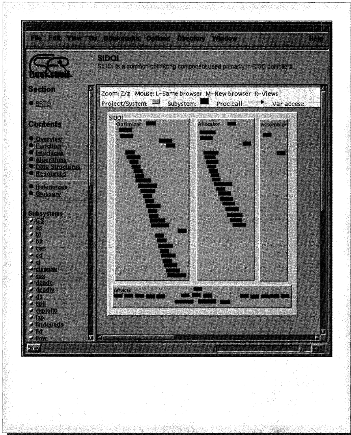
Figure 10 High-level architectural view of the SIDOI system
