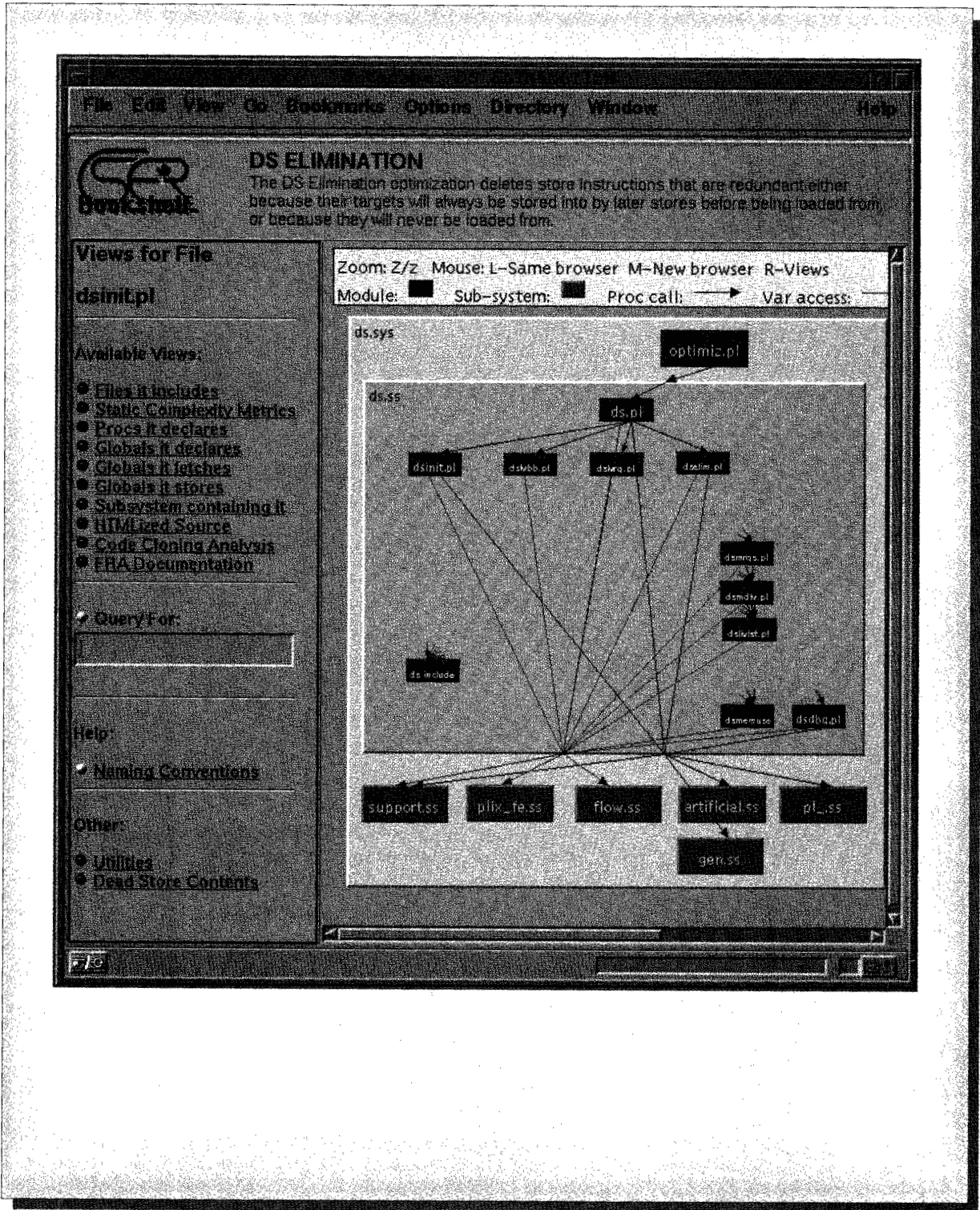
Figure 12 Available views for the dsinit.pl module
