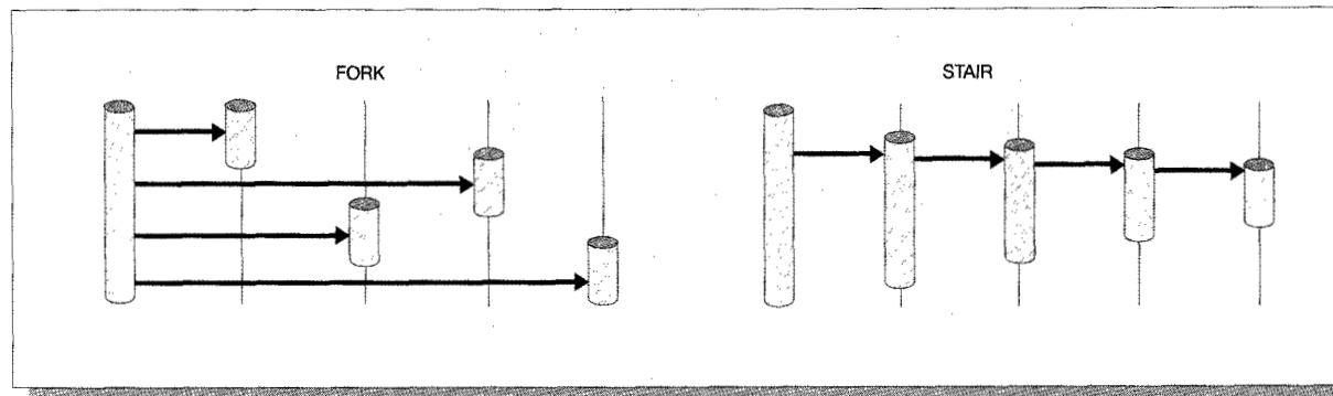
Figure 3 Forks and stairs
