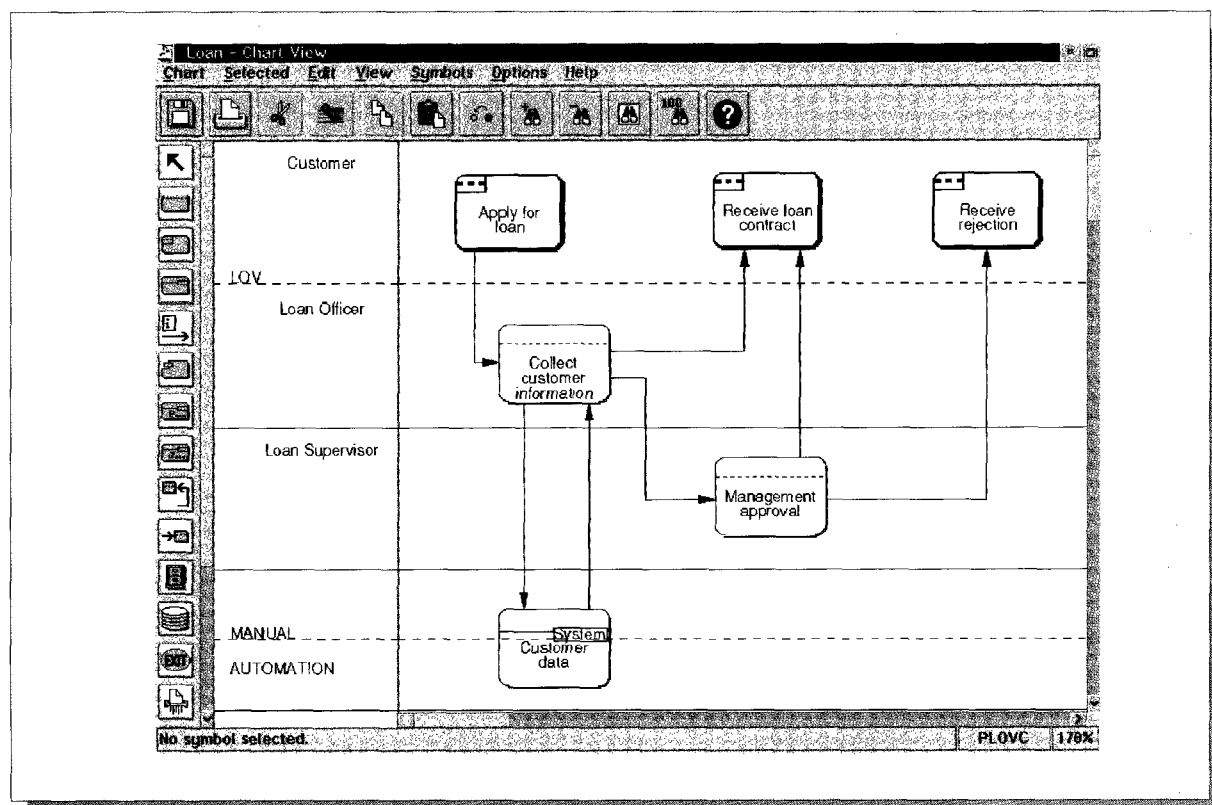
Figure 6 PLOVC of loan application
