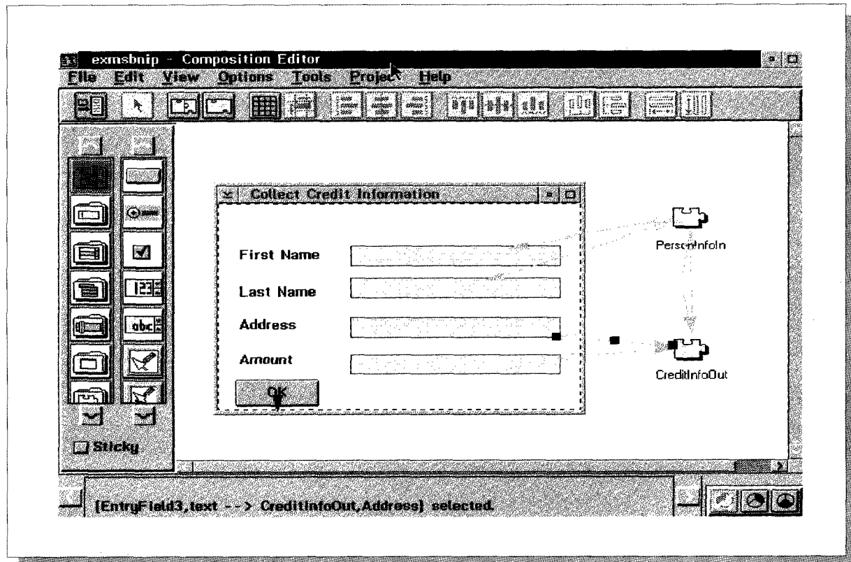
Figure 8 Loan data collection
