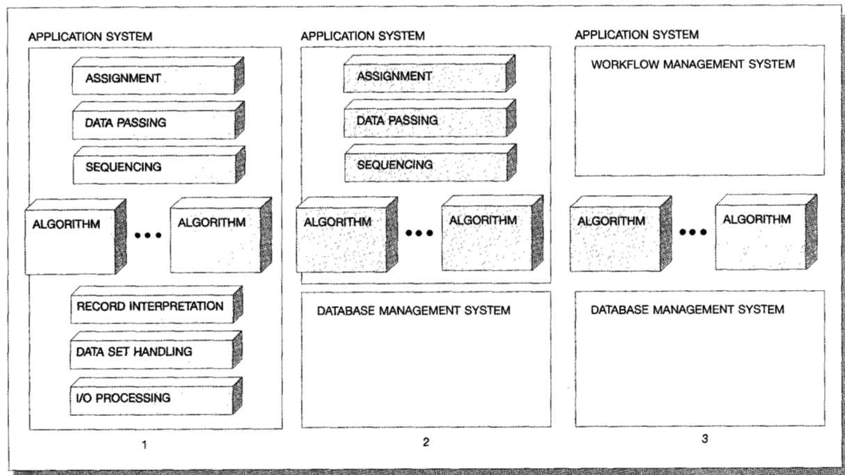
Figure 1 Evolution of application structures
