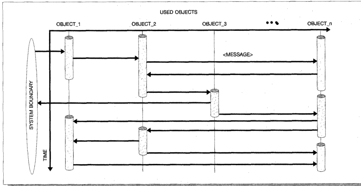
Figure 3 Forks and stairs
