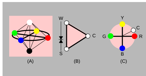
Figure 5 The Natural Color System is based upon Hering's Opponent Color Theory. (A) The system takes as its basic elements: black, white, red, green, blue, and yellow. These colors are taken as absolute "mental" references, from which all other colors are determined by their degree of resemblance. (B) Grays are described by the percentage of black and the percentage of white they contain. (C) Chromatic colors are described in terms of all six components.
