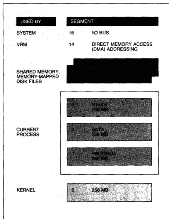
Figure 9 AIX virtual memory segment allocation
