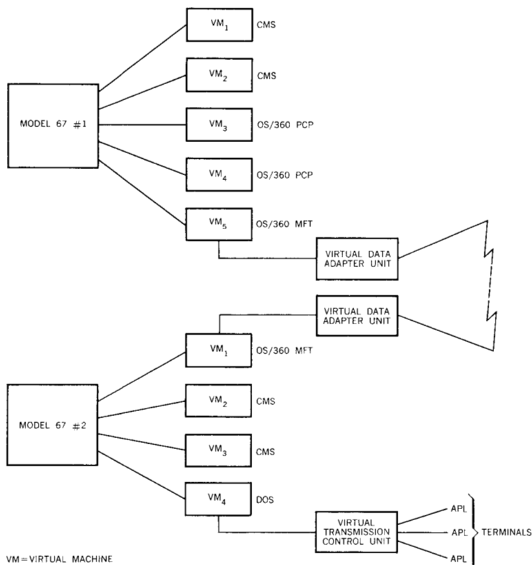
Figure 7 Teleprocessing checkout during normal operation of CP-67
