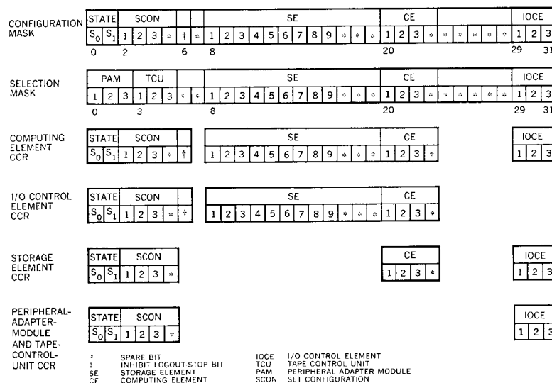
Figure 2 Configuration- and selection-mask formats and configuration contents
