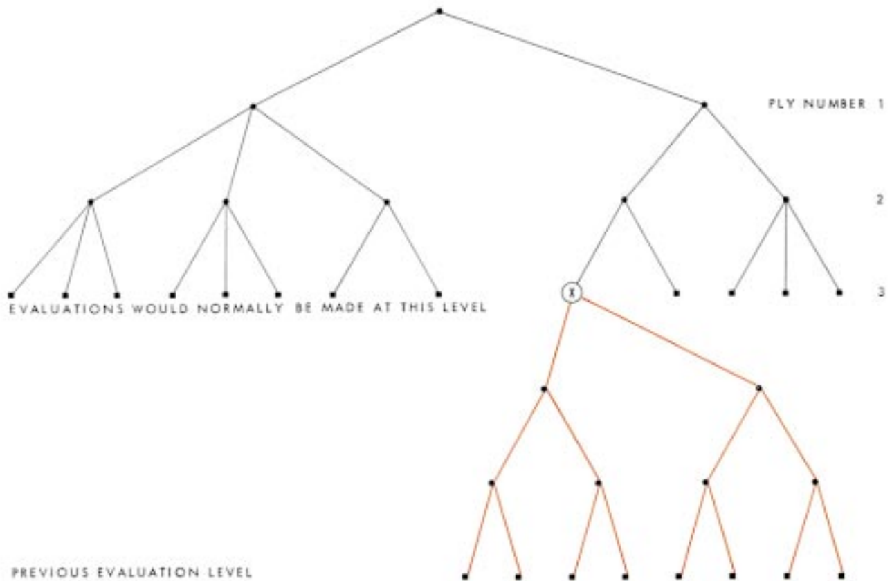
Figure 3 Simplified representation of the rote-learning process, in which information saved from a previous game is used to increase the effective ply of the backed-up score.
