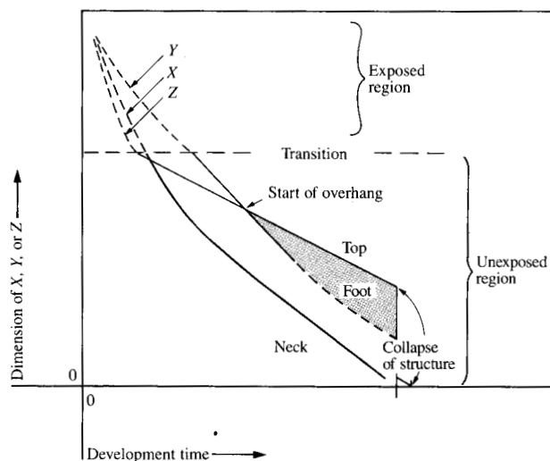
Figure 3 Changes in the development rates for the widths of the top Z , the foot Y , and the neck X as functions of the development time in both exposed and unexposed regions.
