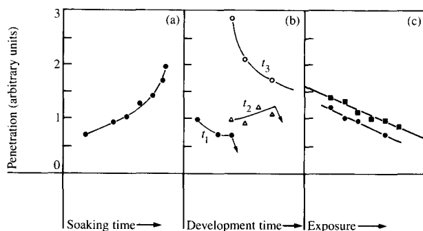
Figure 7 Penetration as a function of (a) soaking time, (b) development time (for different soaking times t_1 < t_2 < t_3 ), and (c) exposure. In (c) the lines refer to two completely different sets of processing parameters, in which the soaking times, baking temperatures, and development times all differ.
