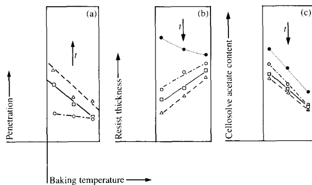
Figure 12 (a) Penetration, (b) resist thickness, and (c) ^{\circ}\text{C} ellosolve acetate content as functions of the baking temperature for a series of soaking times t , where t_0 = 0 (●) < t_1 (○) < t_2 (□) < t_3 (△).
