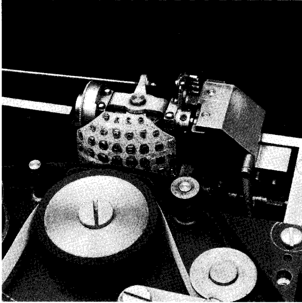
Figure 3 "Mushroom" print element mounted on double gimbal.
