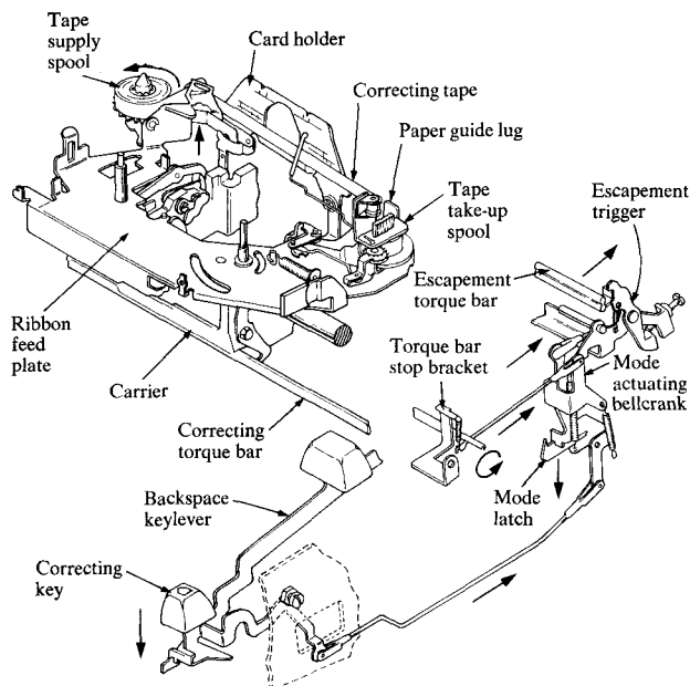
Figure 11 Correcting mechanism.
