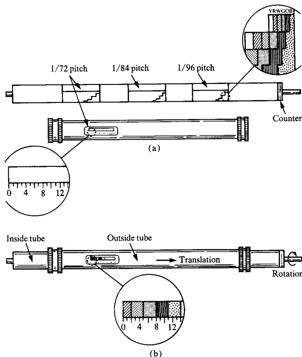
Figure 9 Indicating mechanism as used in Composer.
