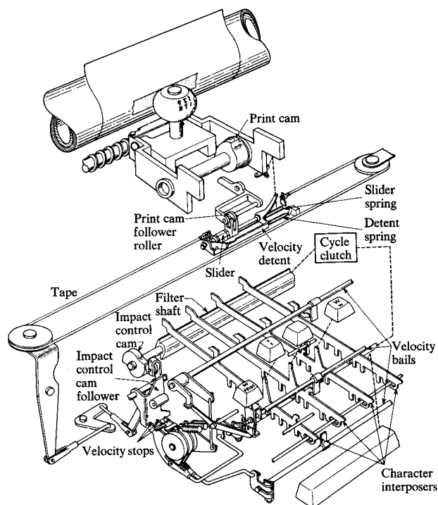
Figure 10 Impact selection system.
