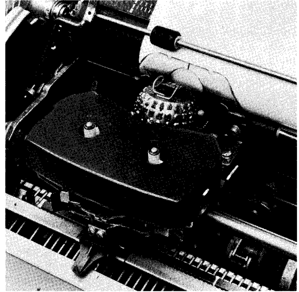
Figure 4 Typehead-carrier-paper relationship.
