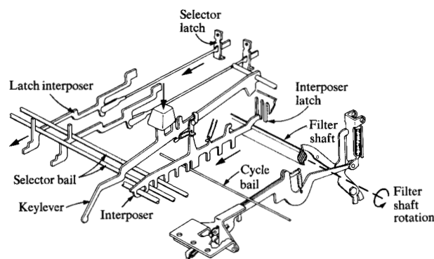
Figure 7 Keyboard and character selection mechanism.
