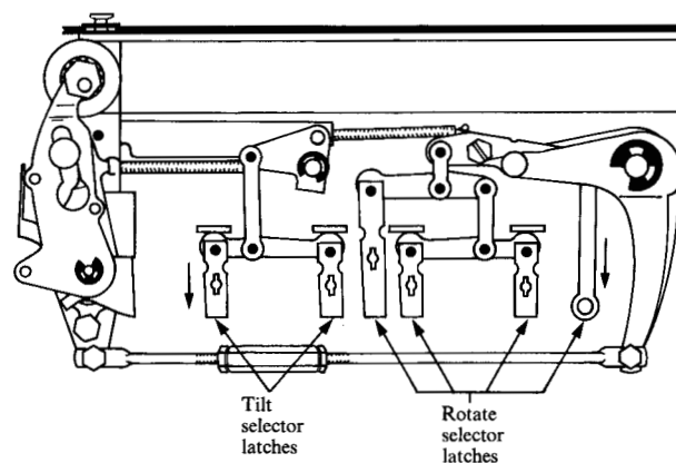
Figure 6 Tilt-and-rotate selector system.
