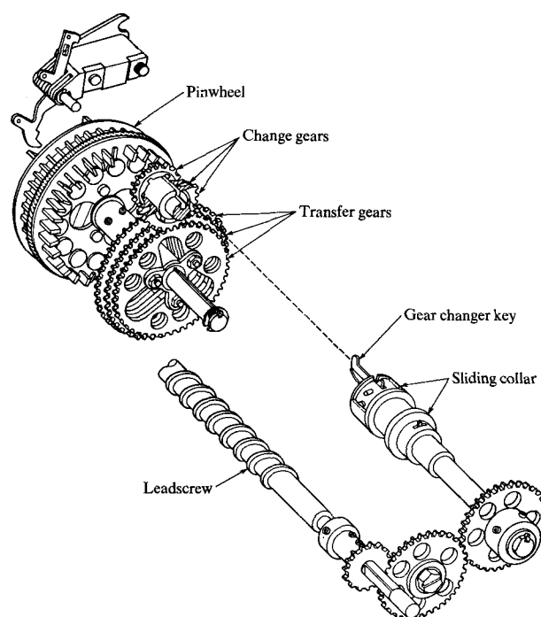
Figure 8 Simplified illustration of leadscrew, variable gear train, and pinwheel.
