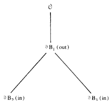
Figure 9 Tree of 2-cycles.
