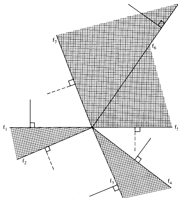
Figure 10 Finding virtual blocks—an edge's perspective.
