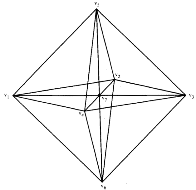
Figure 7 A regular octahedron after Stage 4 with cutting edges inserted.
