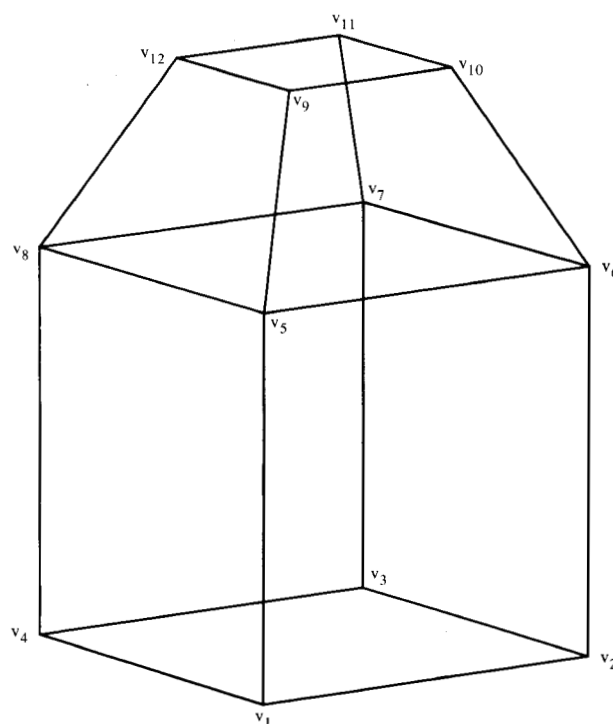
Figure 8 An example of a pseudo-face.
