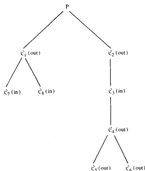
Figure 5 Tree of 1-cycles.
