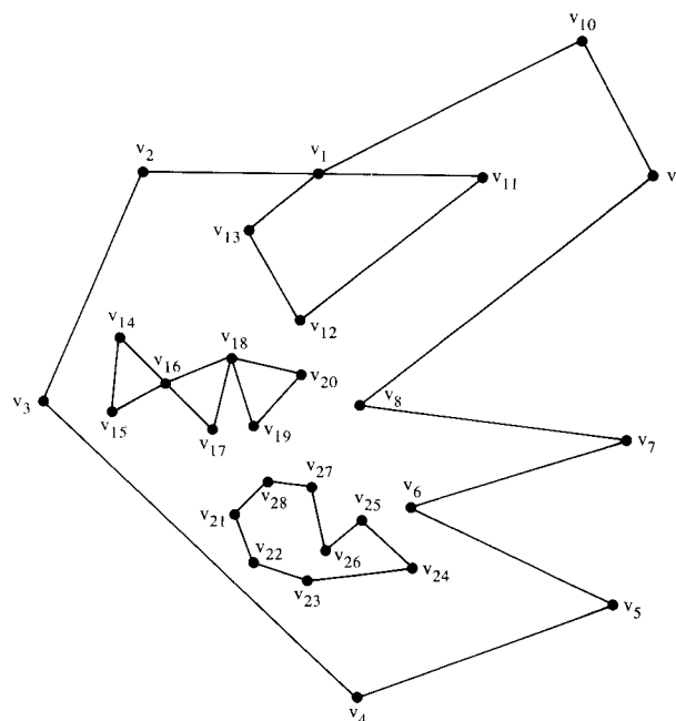
Figure 2 A typical face.
