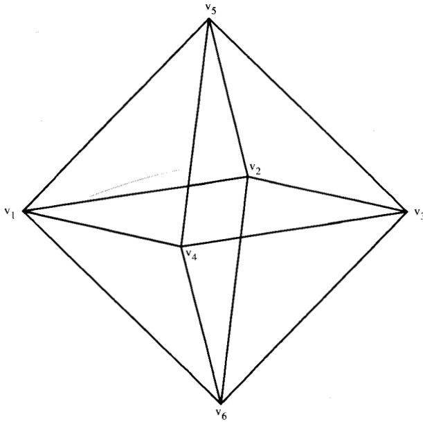
Figure 6 A regular octahedron exhibits many type II intersections.
