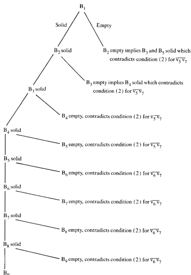
Figure 11 A decision tree for the regular octahedron.
