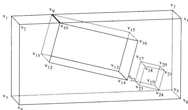
Figure 3 A typical primitive object.
