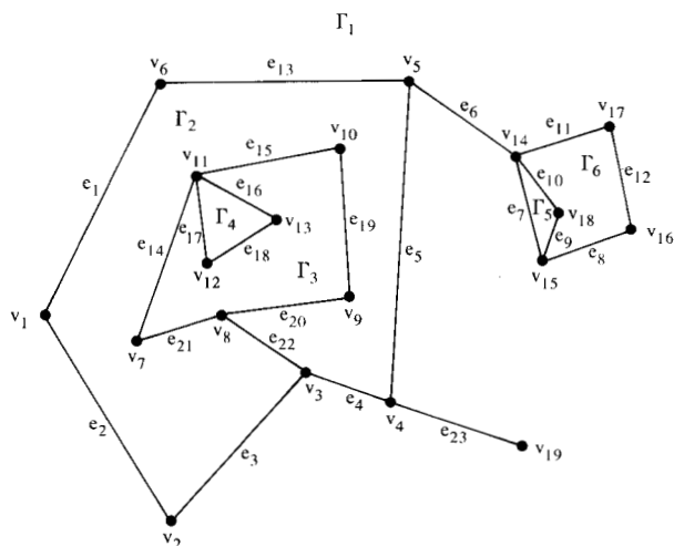
Figure 4 A typical graph in a plane.
