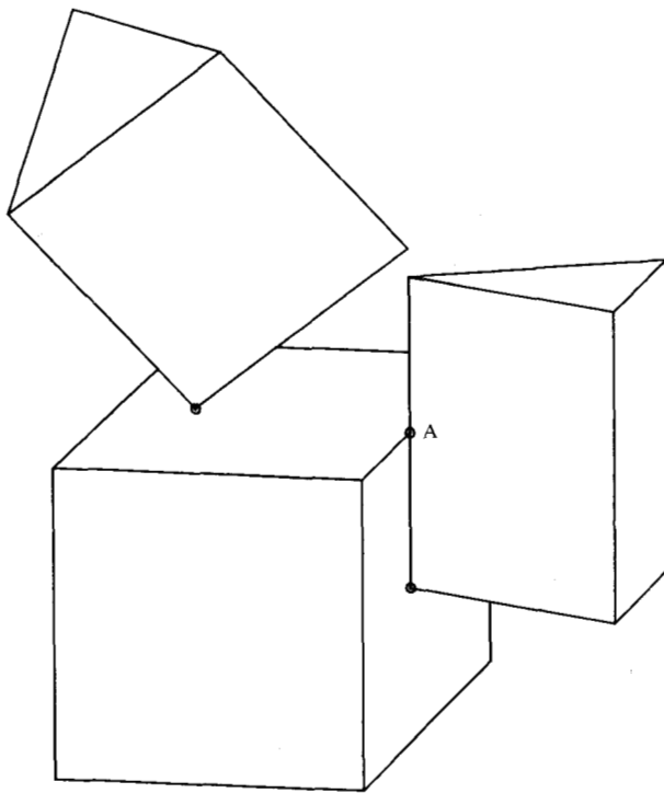
Figure 1 An object exhibiting various kinds of intersections.
