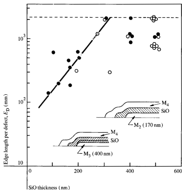
Figure 7 Edge length per insulator defect versus SiO thickness for M_2/I_{3b}/M_4 (●) and M_3/I_{3a} + I_{3b}/M_4 (○) crossings. The dashed line gives the total testable edge length per wafer. The insets show cross sections of structure edges.
