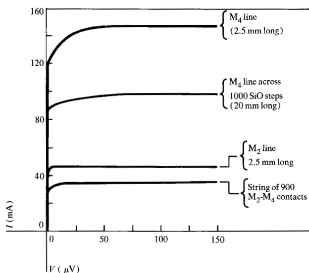
Figure 6 I - V characteristics of typical lines ( 7\ \mu\text{m} wide) and a series-connected string of superconducting contacts.
