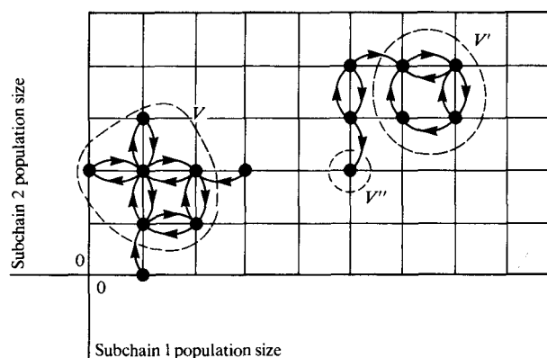
Figure 3 A queueing network in \mathcal{N}^* with general loss and trigger functions.
