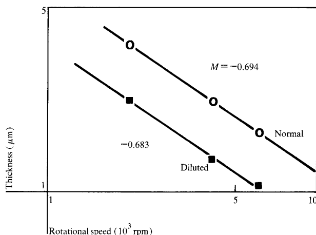
Figure 8 Spin coating thickness of normal (14 percent solids) and diluted (11.5 percent solids) DuPont RC5057; data of Zielinski on silicon wafers [21], M_{calc} = -0.667 .
