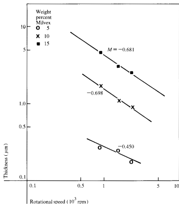
Figure 5 Spin coating thickness of a Milvex 4000-iso-amyl alcohol mixture on a 20.3-cm \times 25.4-cm glass plate for three concentrations; M_{\text{calc}} = -0.667 .
