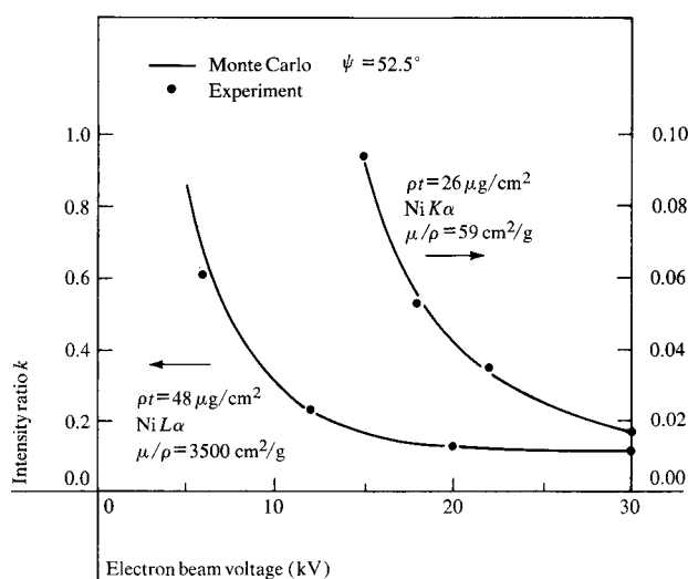
Figure 6 Comparison of Monte Carlo theory with experiment for Ni films on SiO_2 .
