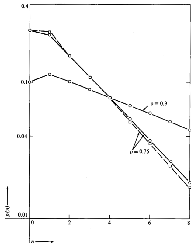
Figure 5 The queue size distribution (in logarithmic scale) for the E_2/M/1 , i.e., C_a = 0.5 . For \rho = 0.9 the diffusion approximation solution (dashed lines) and the exact solution (solid lines) are indistinguishable.
