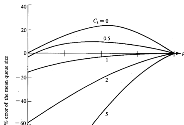
Figure 2 Relative error of the mean queue size e_r vs the server utilization \rho in the M/G/1 system, e_r = (E[n] - E[\hat{n}])/E[n] , where the parameter is C_s , the squared coefficient of variation of service time.
