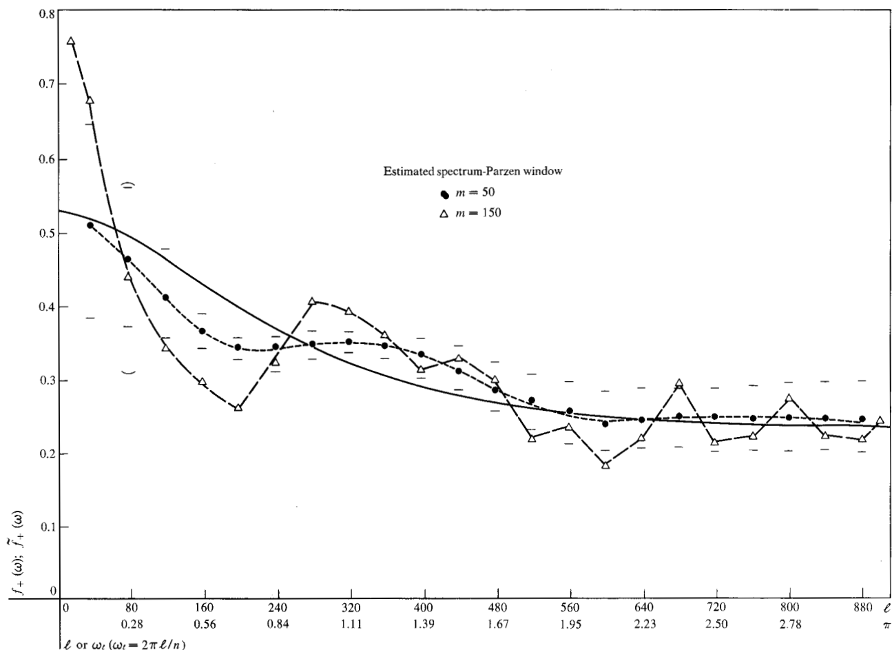
Figure 2 Fitted semi-Markov spectrum of intervals for page exception process for tape A with LRU replacement algorithm. Page size 4K, capacity = 76, n = 1807 . Theoretical (solid line) spectrum for semi-Markov process with estimated parameters \hat{\pi}_1 = 0.066 , \hat{k} = 0.45 , \hat{\gamma} = 0.950 , \hat{\alpha}_2 = 0.962 , \hat{\alpha}_1 = 0.458 , \hat{\mu}_1 = 45,715 , \hat{\mu}_2 = 1,973.1 .
