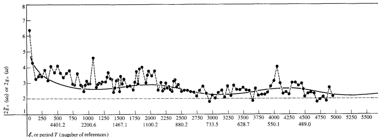
Figure 3 Fitted semi-Markov spectrum of counts for page exception process for tape A with LRU replacement algorithm. Page size 4K, capacity = 76, n = 1807 . Smoothed spectrum, average of four sections, each smoothed with quadratic window. 50 points (dashed line). Theoretical spectrum (solid line) for semi-Markov process with estimated parameters \hat{\gamma} = 0.950 , \hat{k} = 0.45 , \hat{p}_2 = 0.99977748 , \hat{p}_1 = 0.99997813 , \hat{\alpha}_1 = 0.458 , \hat{\alpha}_2 = 0.962 .
