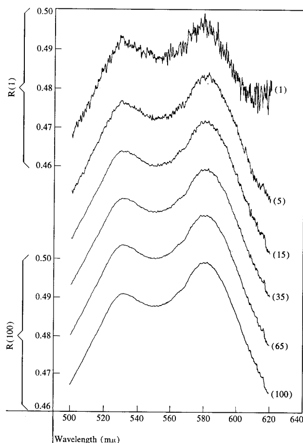
Figure 11 Reflectivity spectrum of the germanium A spin-orbit doublet. This figure represents the average of up to 100 scans at signal/noise intervals of approximately 2, 4, 6, 8, and 10. The total number of equally spaced points per scan is 601. All curves are plotted to the same scale, but only those for the first and one-hundredth are shown in proper perspective. The amplitude resolution is judged to be about 0.001 and does not necessarily represent an ultimate figure.
