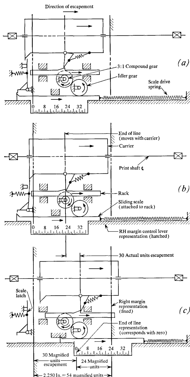
Figure 3 Simplified sketch of sliding-scale indicator.
