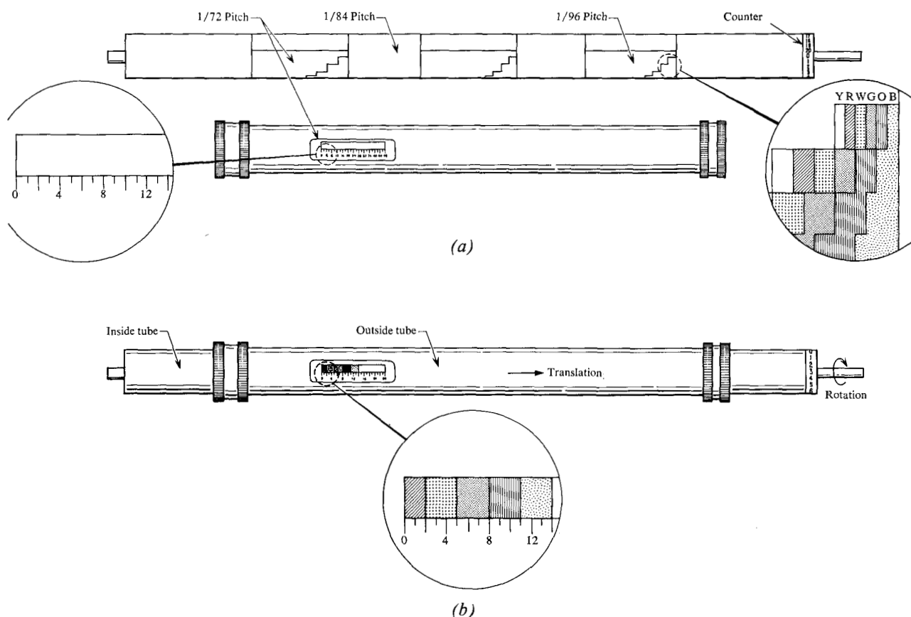
Figure 7 Indicating mechanism as used in composer.
