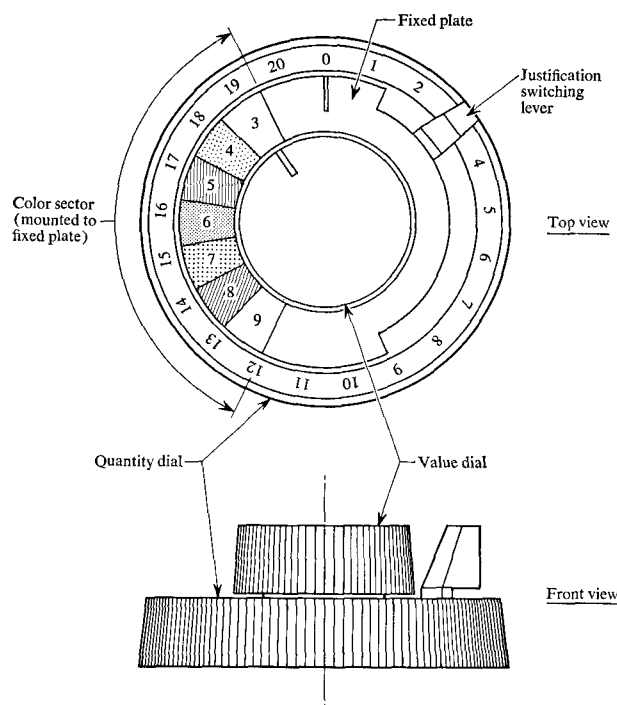
Figure 8 Selection dials.
