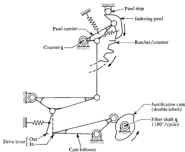
Figure 4 Ratchet counter mechanism.
