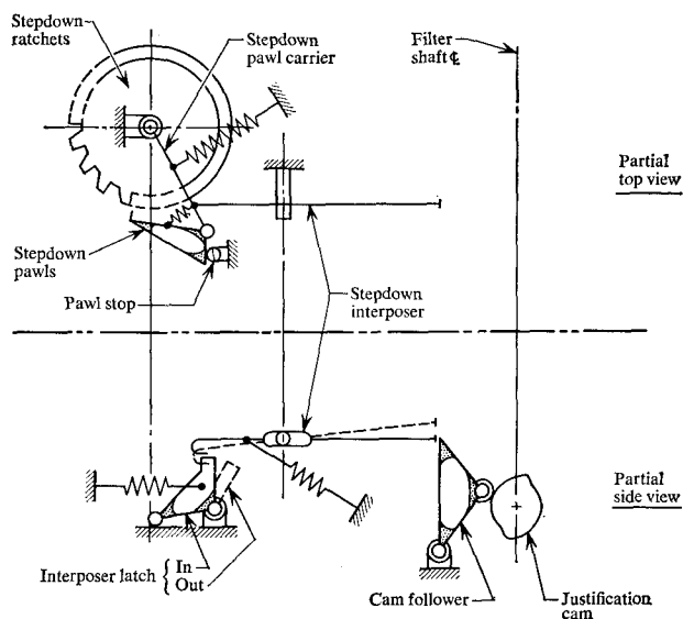
Figure 9 Spacebar stepdown mechanism.
