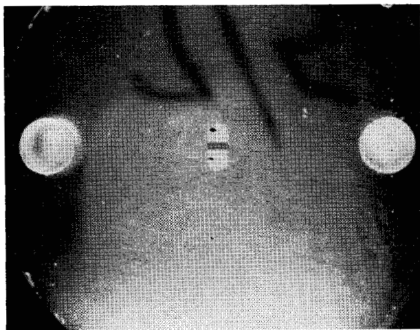
Figure 2d Typical "short" specimen of GaAs after encapsulation.
