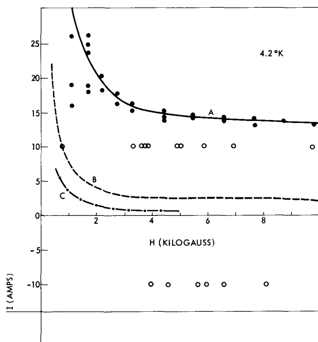
Figure 1 Training phenomena and anomalous resistive transitions in an unannealed Mo-Re wire at 4.2°K. The curves and points are explained in the text.
