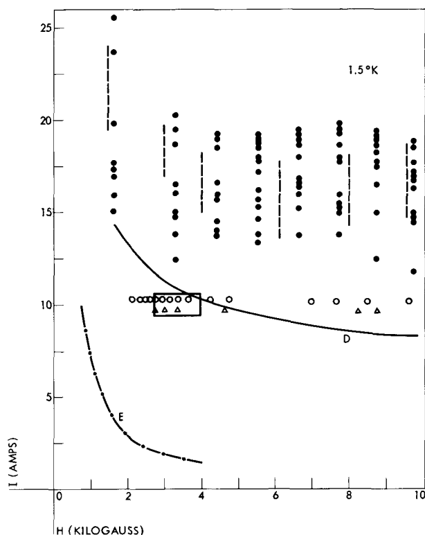
Figure 2 Training phenomena in an unannealed Mo-Re wire at 1.5°K. The curves and points are discussed in the text.
