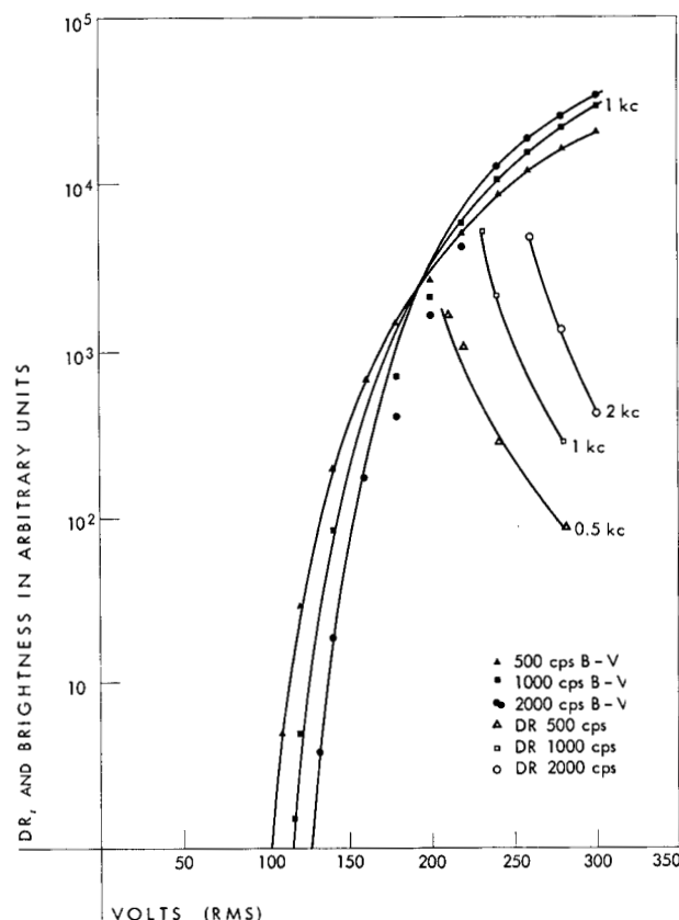
Figure 4 Brightness/voltage and discrimination-ratio/voltage for three frequencies.
