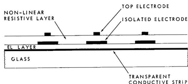
Figure 2 x-y panel, transverse section.
