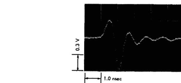
Figure 8 Transverse switching signal shows oscillation of the magnetization for coherent rotation of the magnetization. Film 138a; 80/20 Ni-Fe; 1300 Å; H_c=1.75 oe; H_k=2.5 oe.
