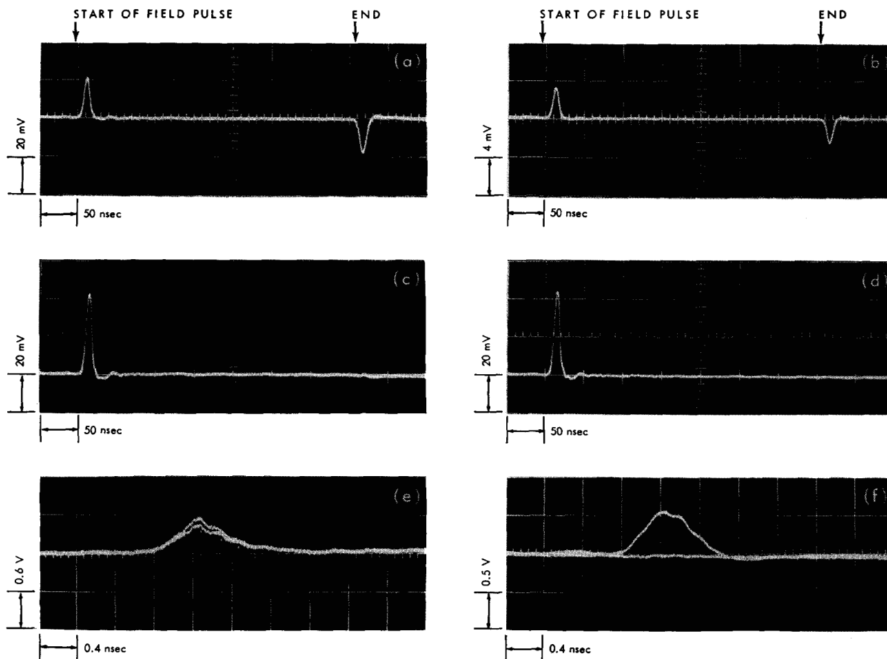
Figure 7 Longitudinal (a), (c), (e) and transverse (b), (d), (f) switching signals for pulse fields H_s in the hard direction with zero transverse field H_r . (Film 215 B2). (a, b) Reversible rotation for H_s < H_K . H_s = 1.6 oe. (c, d) Splitting up of initial single domain for H_s > H_K . H_s = 7.0 oe. (e, f) Comparison of first pulse for single and split-up domain. H_s = 7.0 oe.
