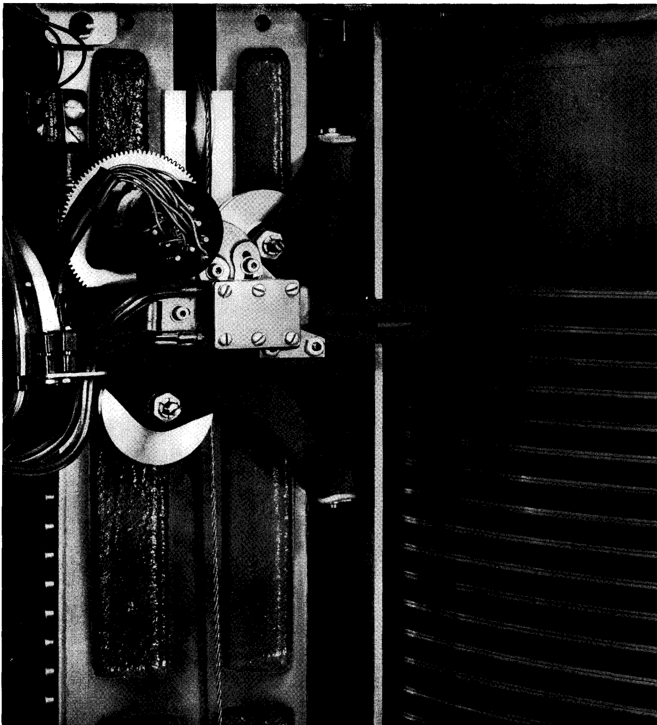
Figure 1 Access mechanism of the IBM Type 350 magnetic-disk, random-access memory.
