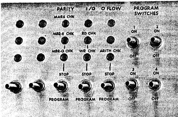
Figure 10. Indicator Displays and Switches
