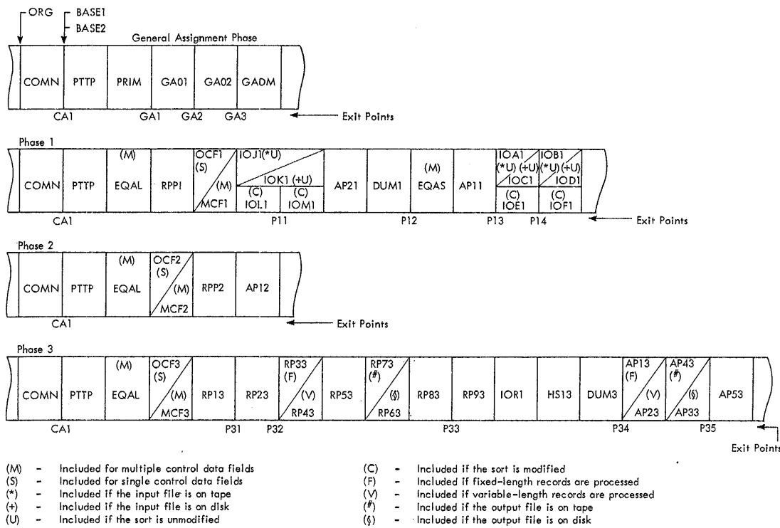
● Figure 7. Generalized Disk Sort Memory Map, Showing the Subroutines that May be Used in Each Phase
