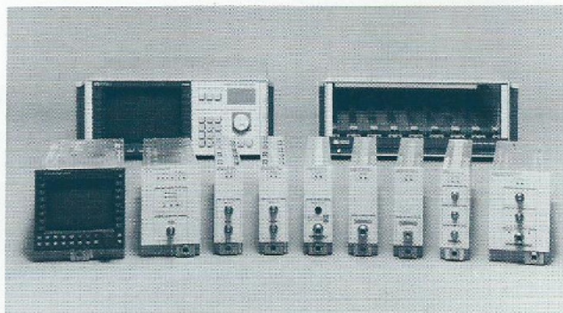
The HP 71000 Modular Spectrum Analyzer family includes 11 components that can be configured for a wide variety of signal analysis applications. Both custom and factory-configured systems are available.
