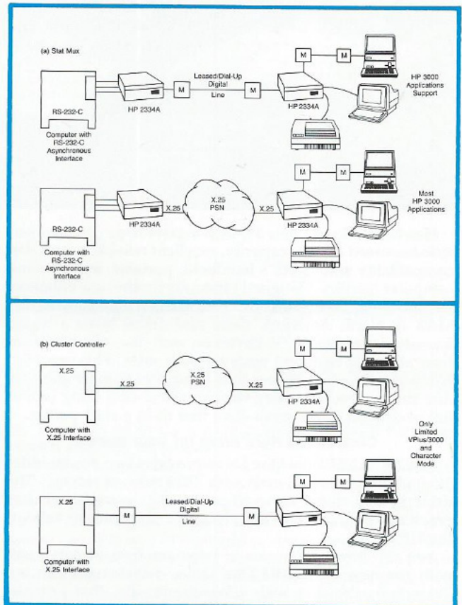
Fig. 1. Comparison of configurations for using the HP 2334A MULTIMUX as (a) a stat mux and (b) a cluster controller.
