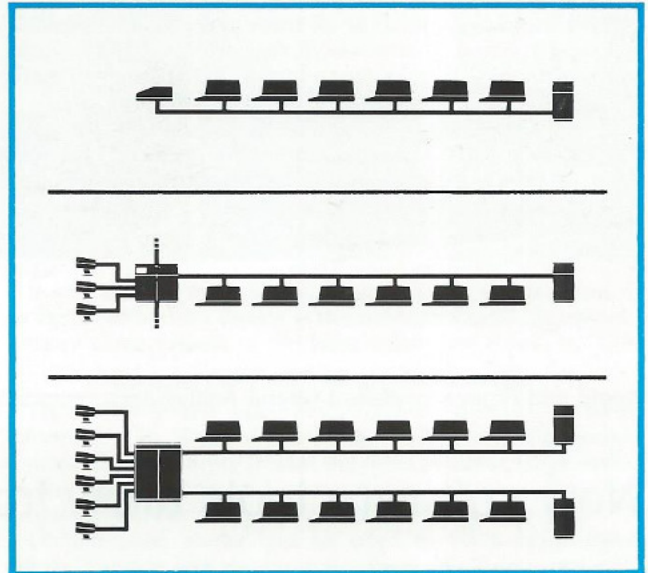
The addition of a host computer to the HP 64000 Logic Development System lets you cluster development stations, hard discs, and terminals to serve large software design teams. A system can be reconfigured at any time to meet changing needs.
