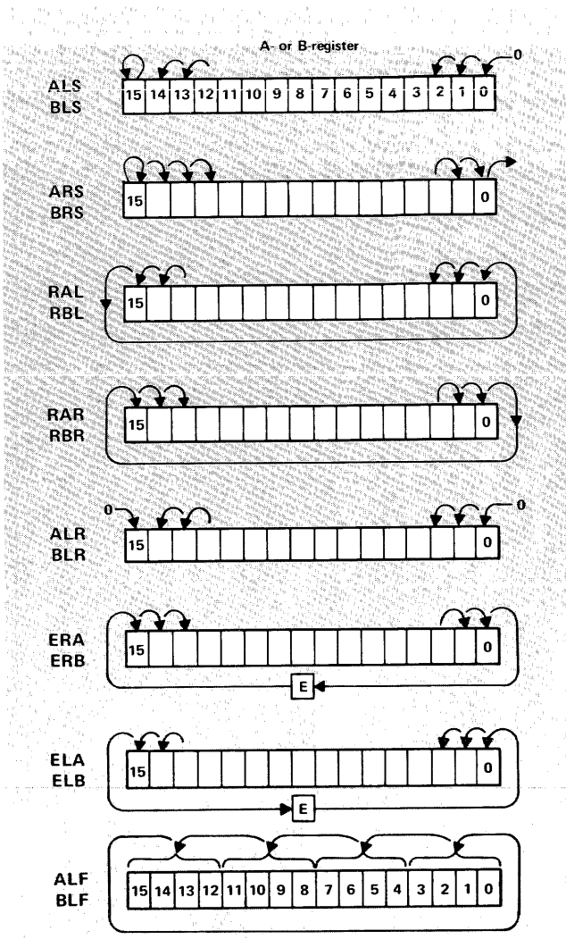
Figure 6. Shift and Rotate Functions
