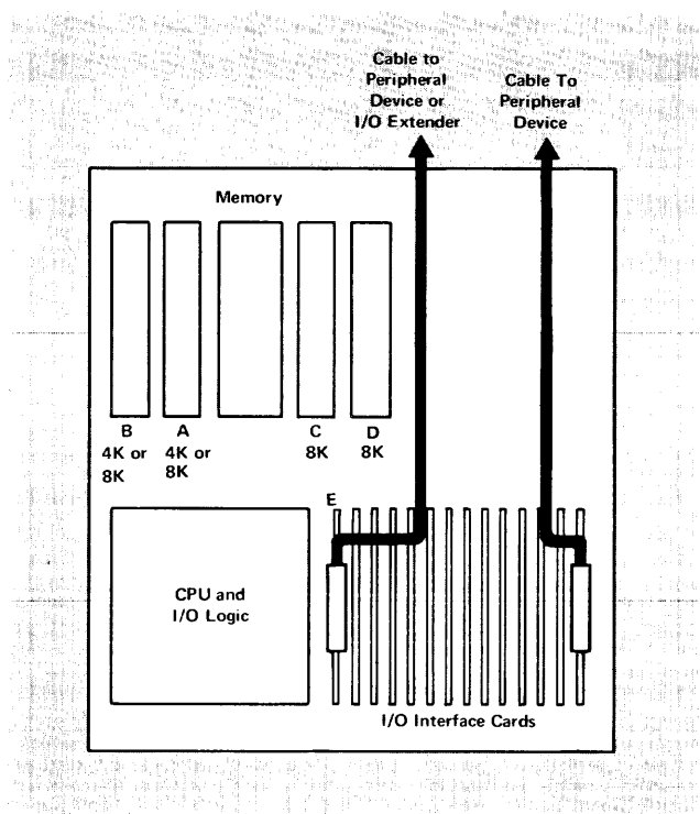
Figure 2. Internal Configuration
