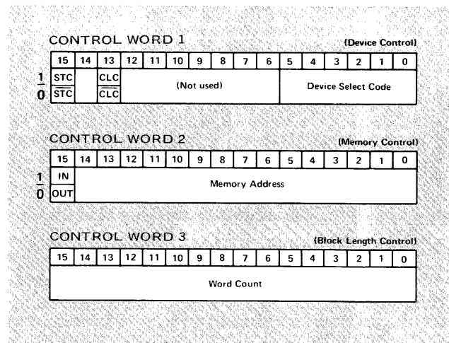
Figure 14. DMA Control Word Formats
