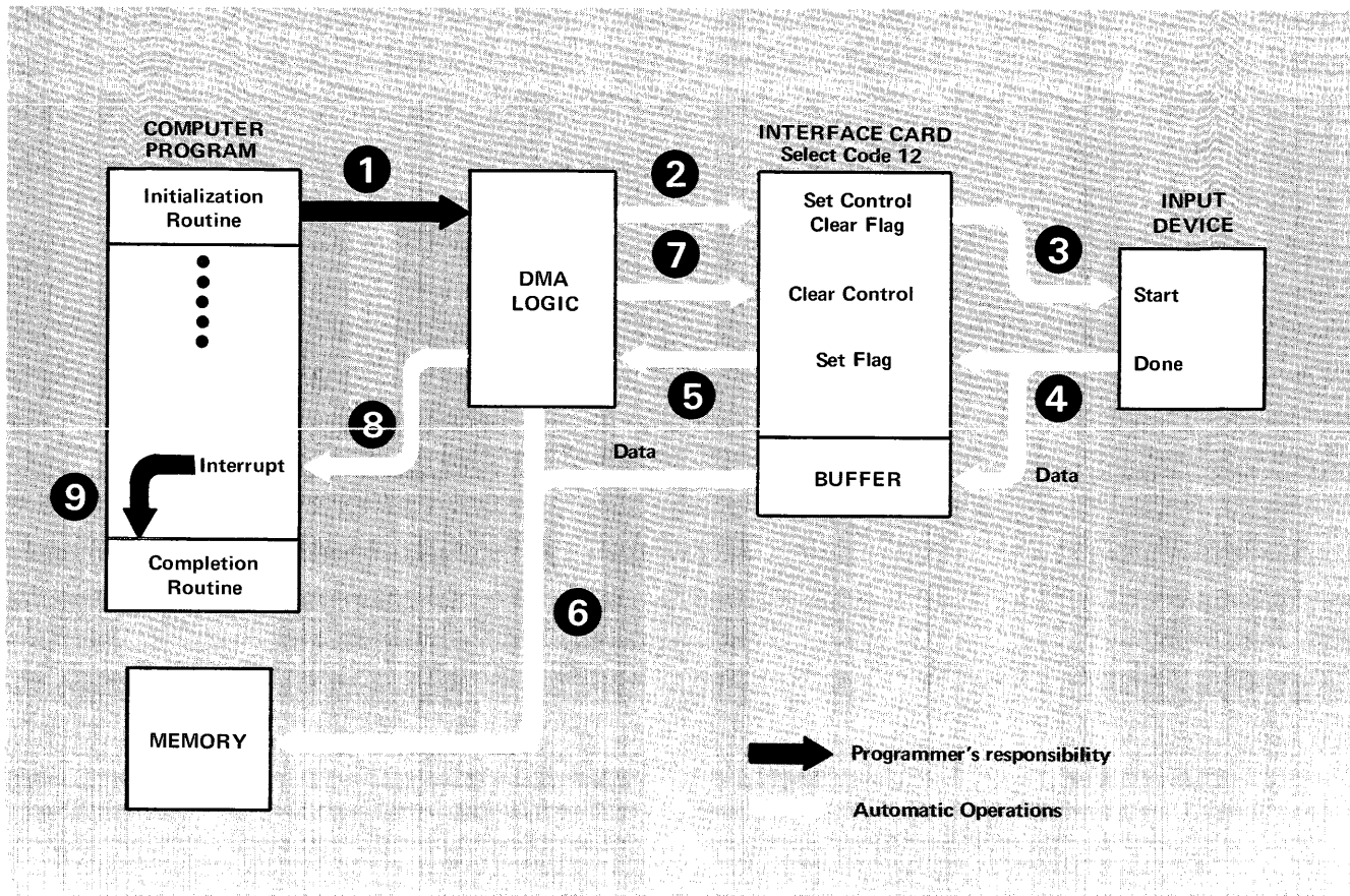
Figure 13. DMA Transfers
