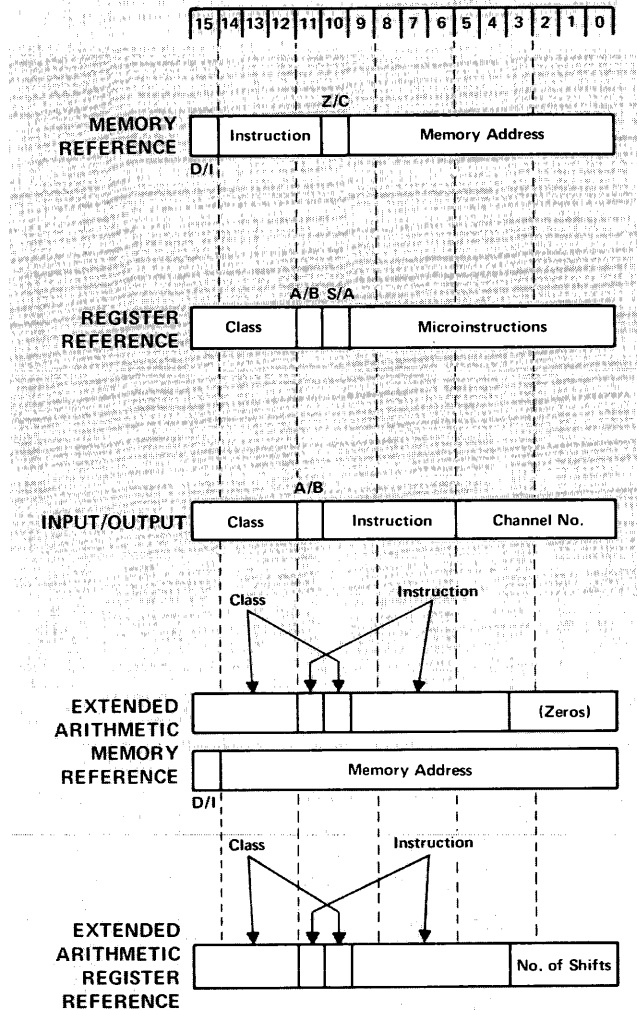
Figure 4. Instruction Formats
