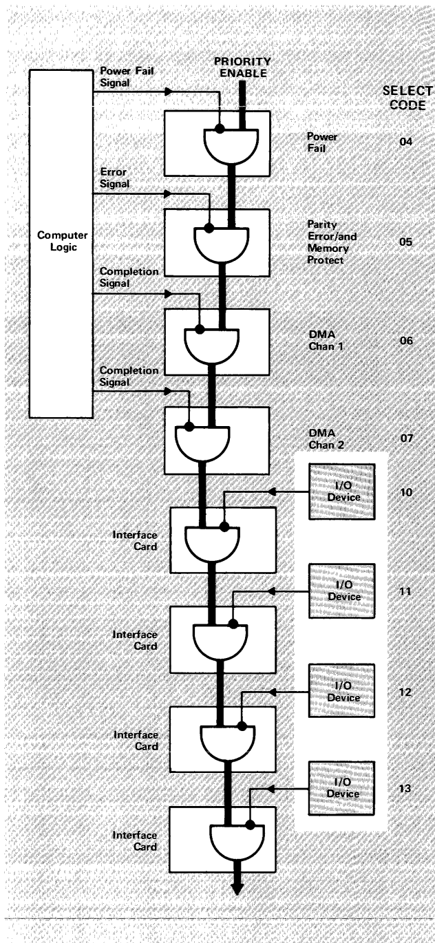
Figure 10. Priority Linkage
