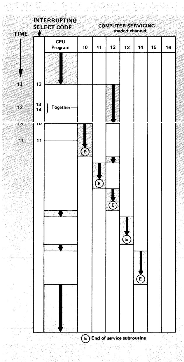
Figure 11. Interrupt Sequences
