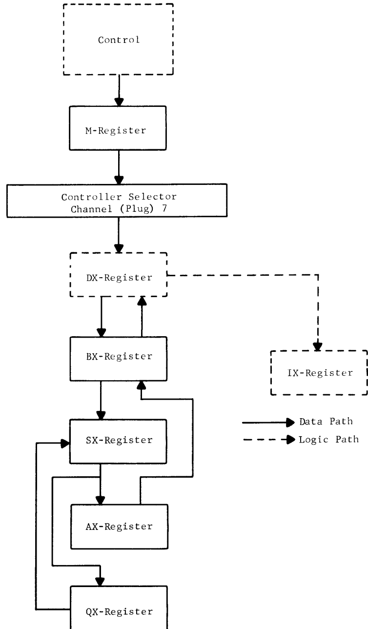
Figure 1. Major Registers and Functional Logic Diagram
