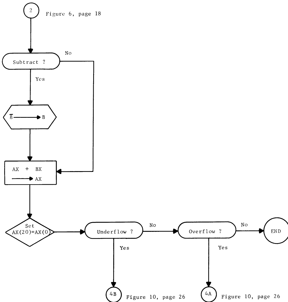
Figure 7. Fixed-Point FAD, FSU
