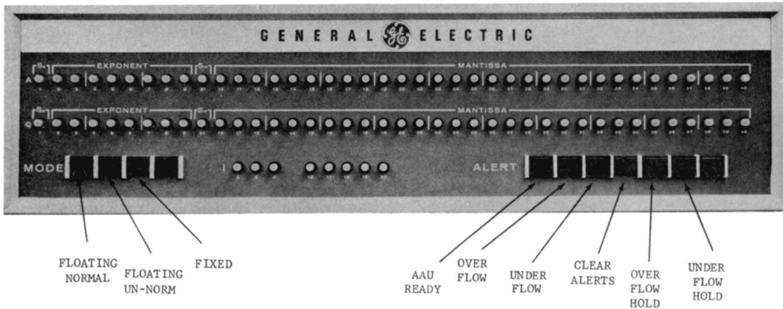
Figure 18. AAU Control and Indicator Panel
