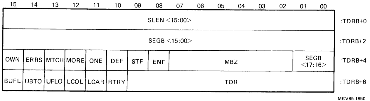
Figure 4-23 Format of an Entry in the Transmit Descriptor Ring
