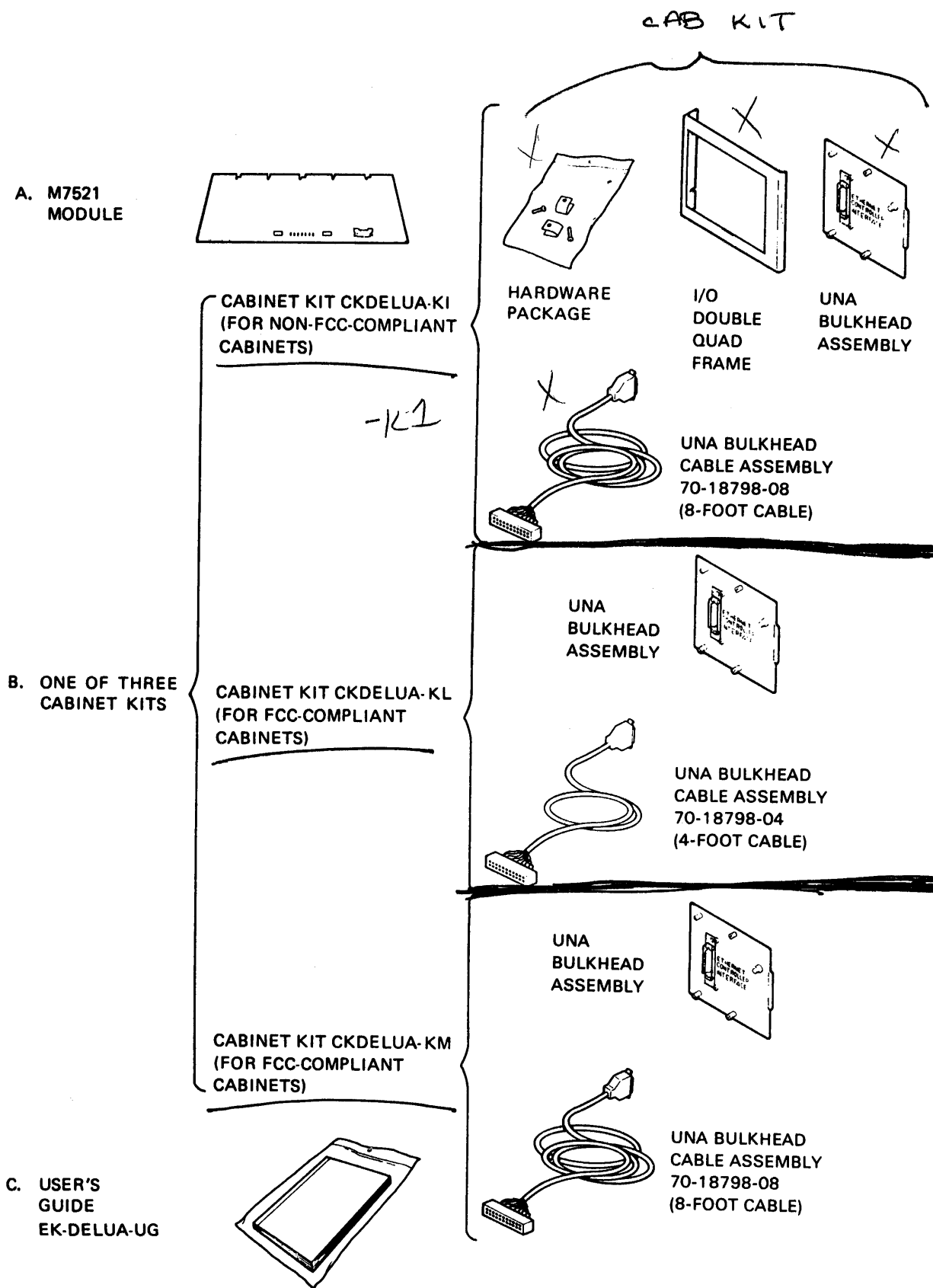
Figure 2-1 DELUA Component Parts
