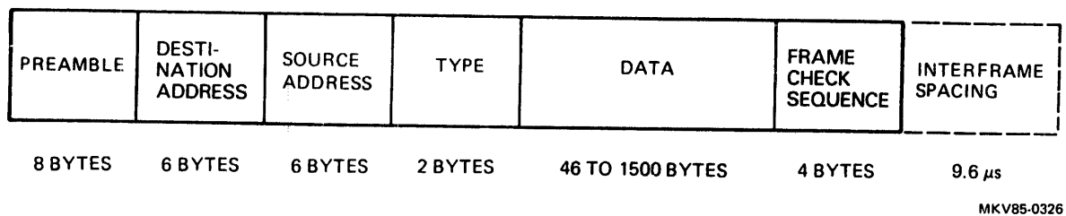
Figure 1-4 Format of a Data Frame
