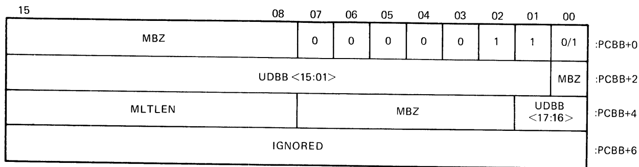
Figure 4-10 Read/Write Multicast Address List, Ancillary Function Codes 6/7 Bit Format
