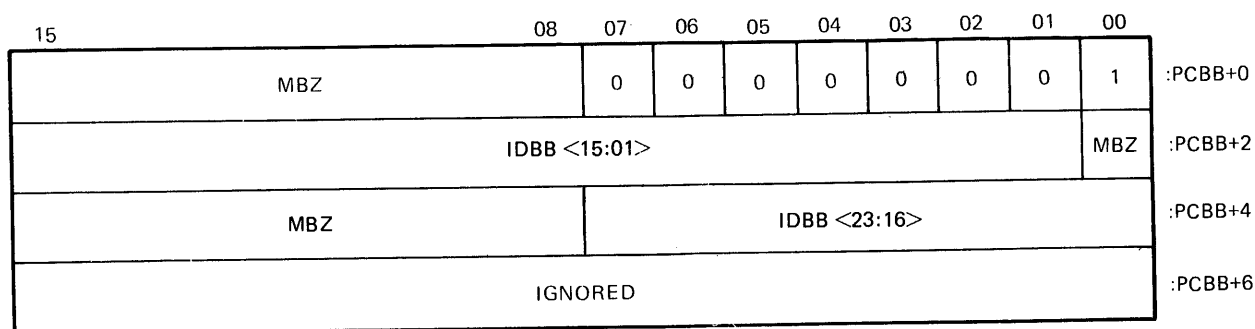
Figure 4-7 Start Microaddress, Ancillary Function Code 1 Bit Format
