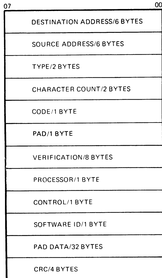
Figure 5-1 Boot Frame Format
