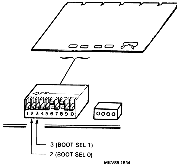
Figure 2-6 Boot Function Switches
