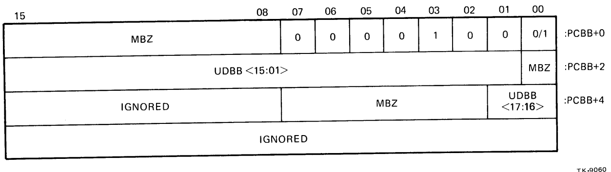
Figure 4-12 Read/Write Descriptor Ring Format, Ancillary Function Codes 10/11 Bit Format
