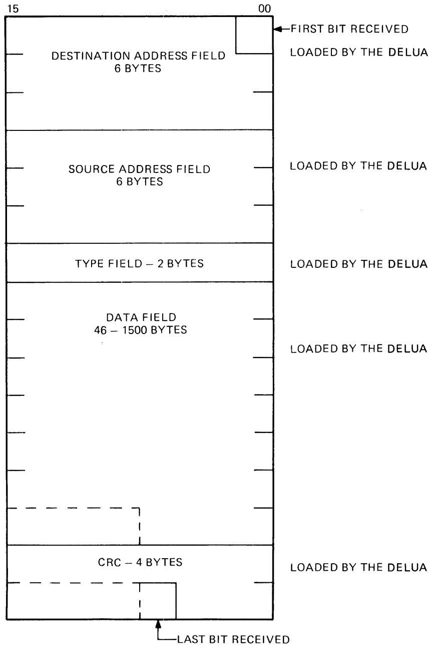
Figure 4-27 Receive Data Buffer Format
