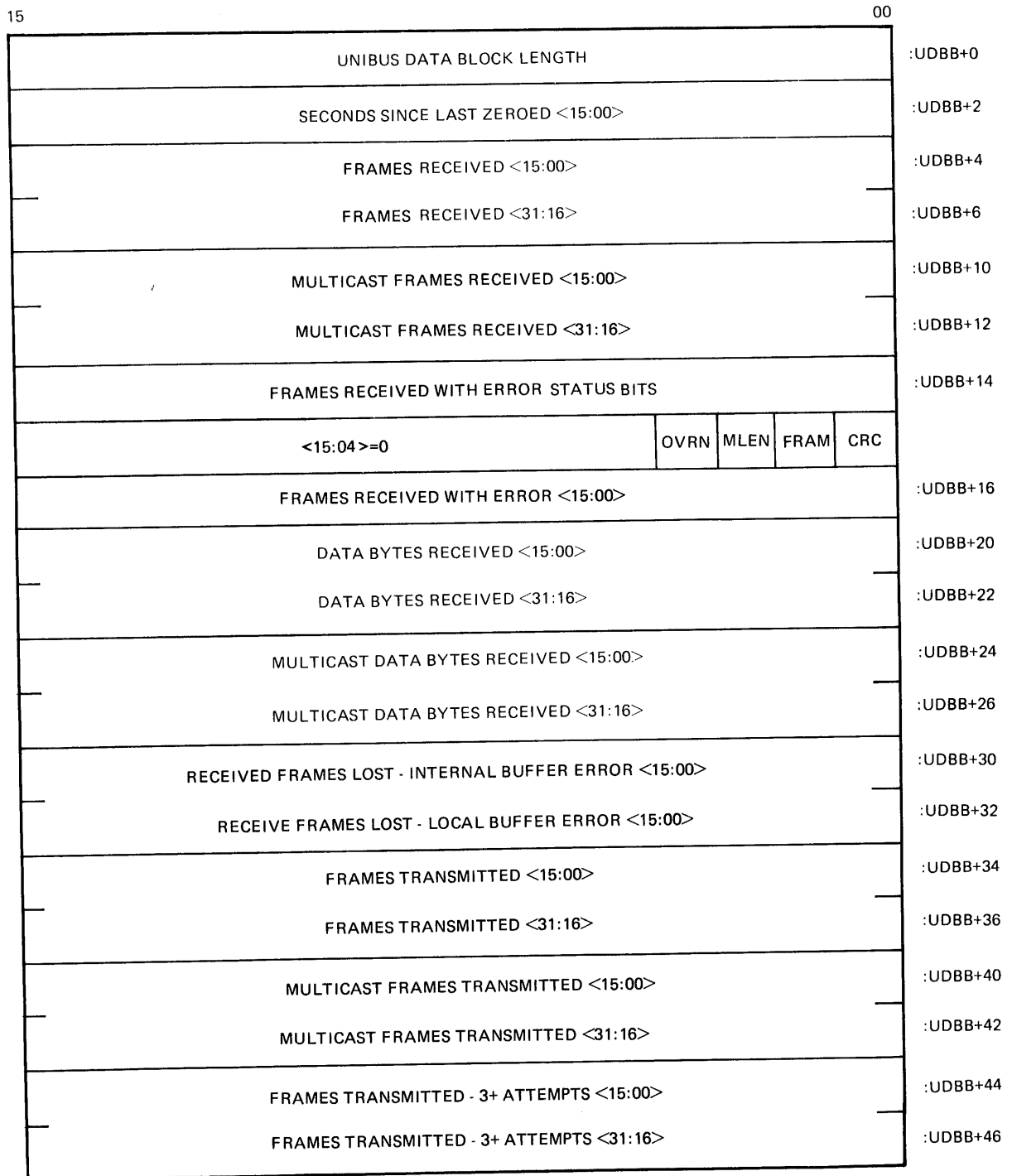
Figure 4-15 Read/Read and Clear Counters UDB Bit Format (Sheet 1 of 2)
