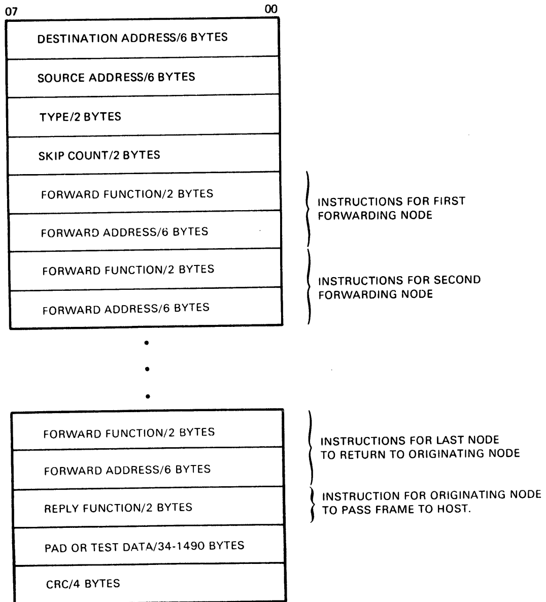
Figure 5-4 Loopback Frame Format
