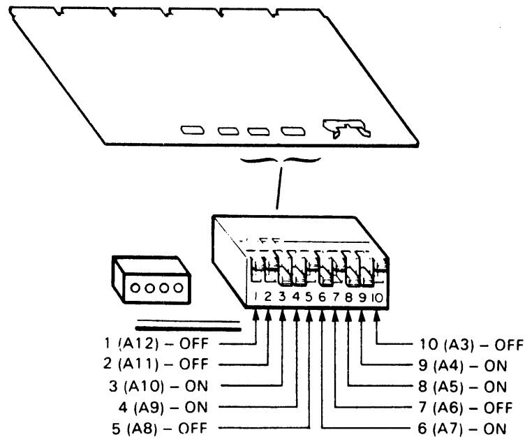
Figure 2-2 Switch Pack at E106, Device Address Assignment
