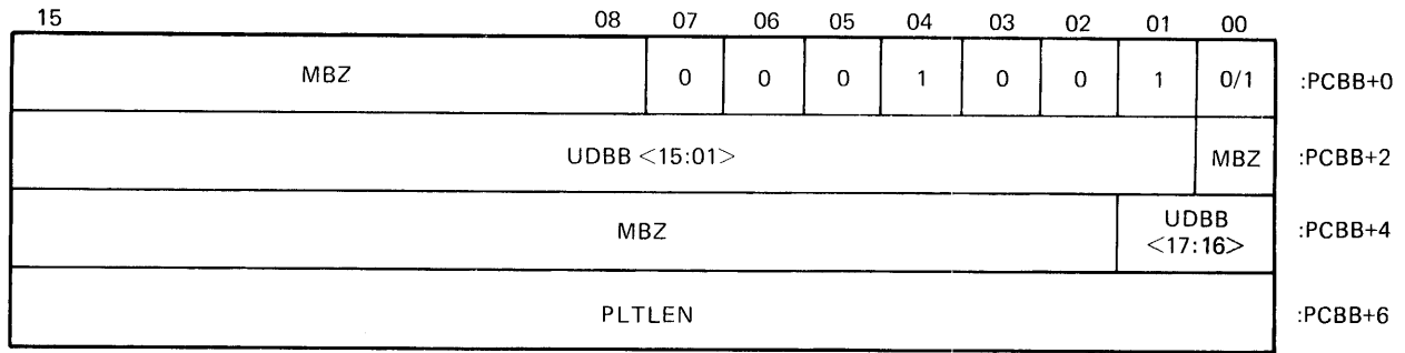
Figure 4-20 Read/Write System ID Parameters, Ancillary Function Codes 22/23 Bit Format
