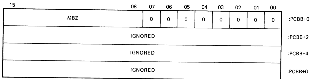
Figure 4-6 No-Operation, Ancillary Function Code 0 Bit Format
