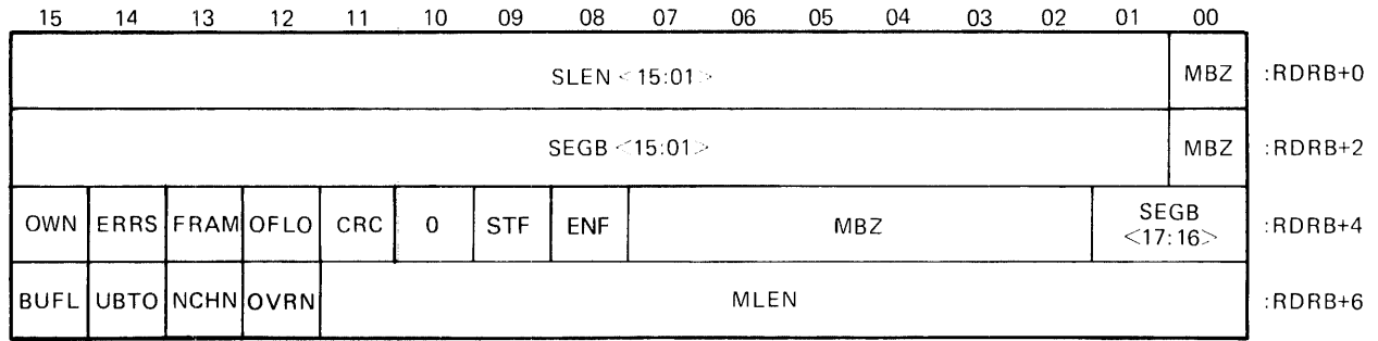
Figure 4-24 Format of an Entry in the Receive Descriptor Ring
