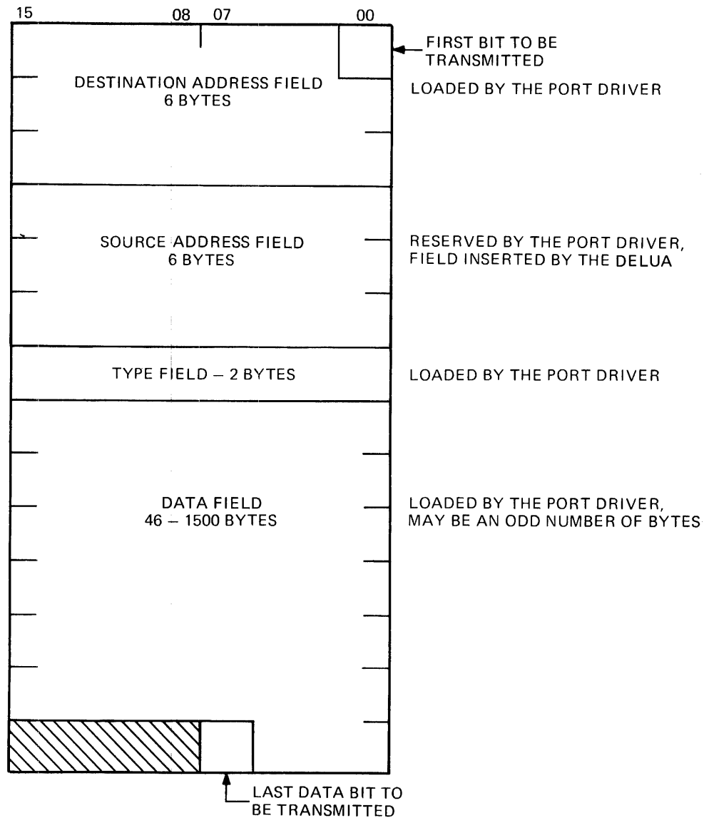
Figure 4-25 Transmit Data Buffer Starting on an Even-Byte Boundary
